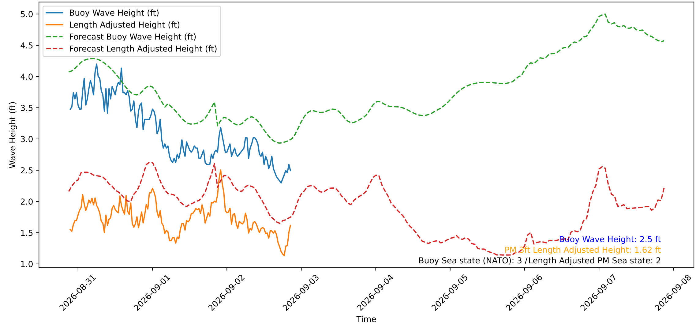
Wave Heights over Time for Red Beach at 2026-09-02 21:10:50
