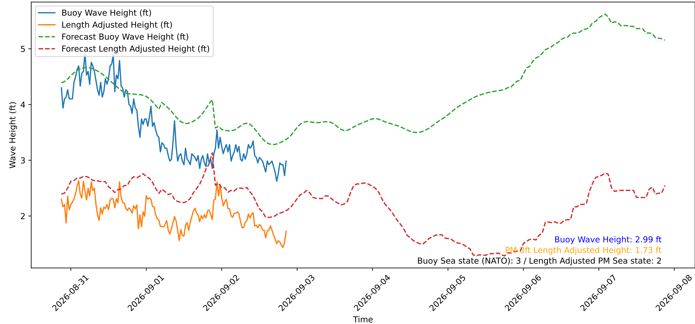
Wave Heights over Time for Oceanside Harbor at 2026-09-02 21:10:30
