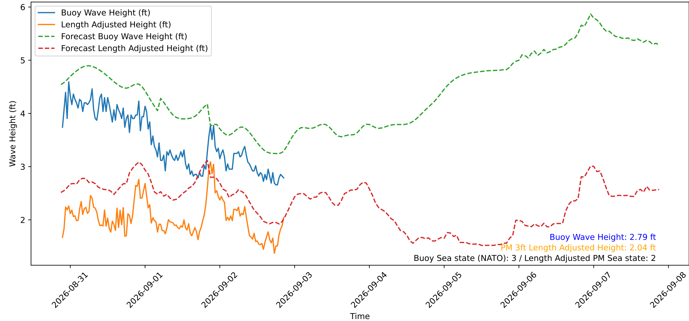
Wave Heights over Time for Green Beach at 2026-09-02 21:11:13
