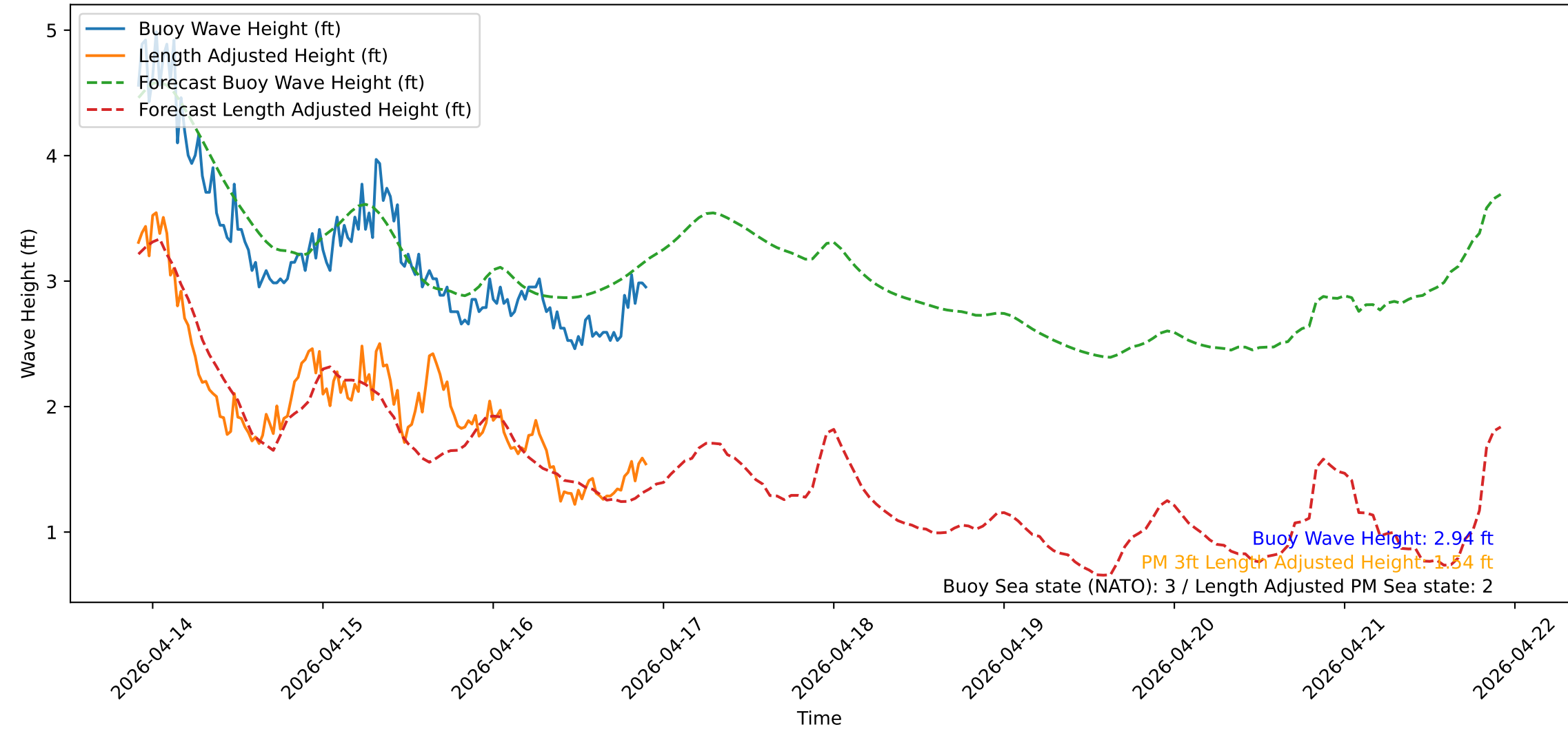
Wave Heights over Time for Green Beach at 2026-04-16 22:11:13
