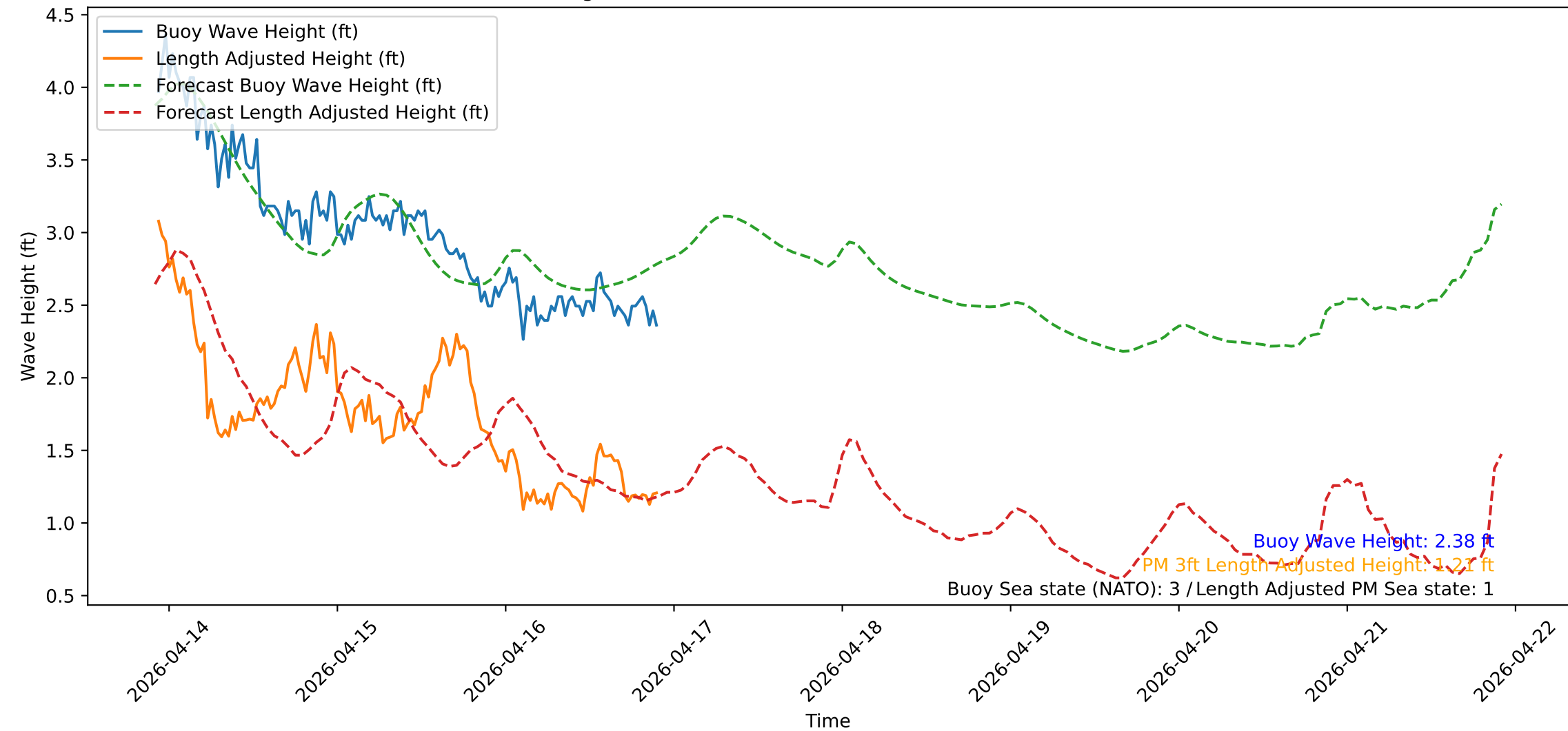
Wave Heights over Time for Red Beach at 2026-04-16 22:10:51
