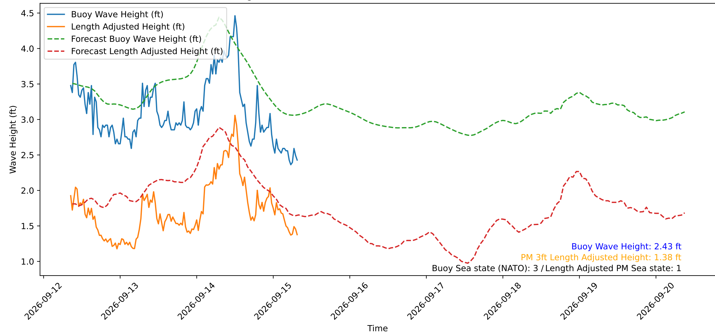
Wave Heights over Time for Oceanside Harbor at 2026-09-15 08:30:30
