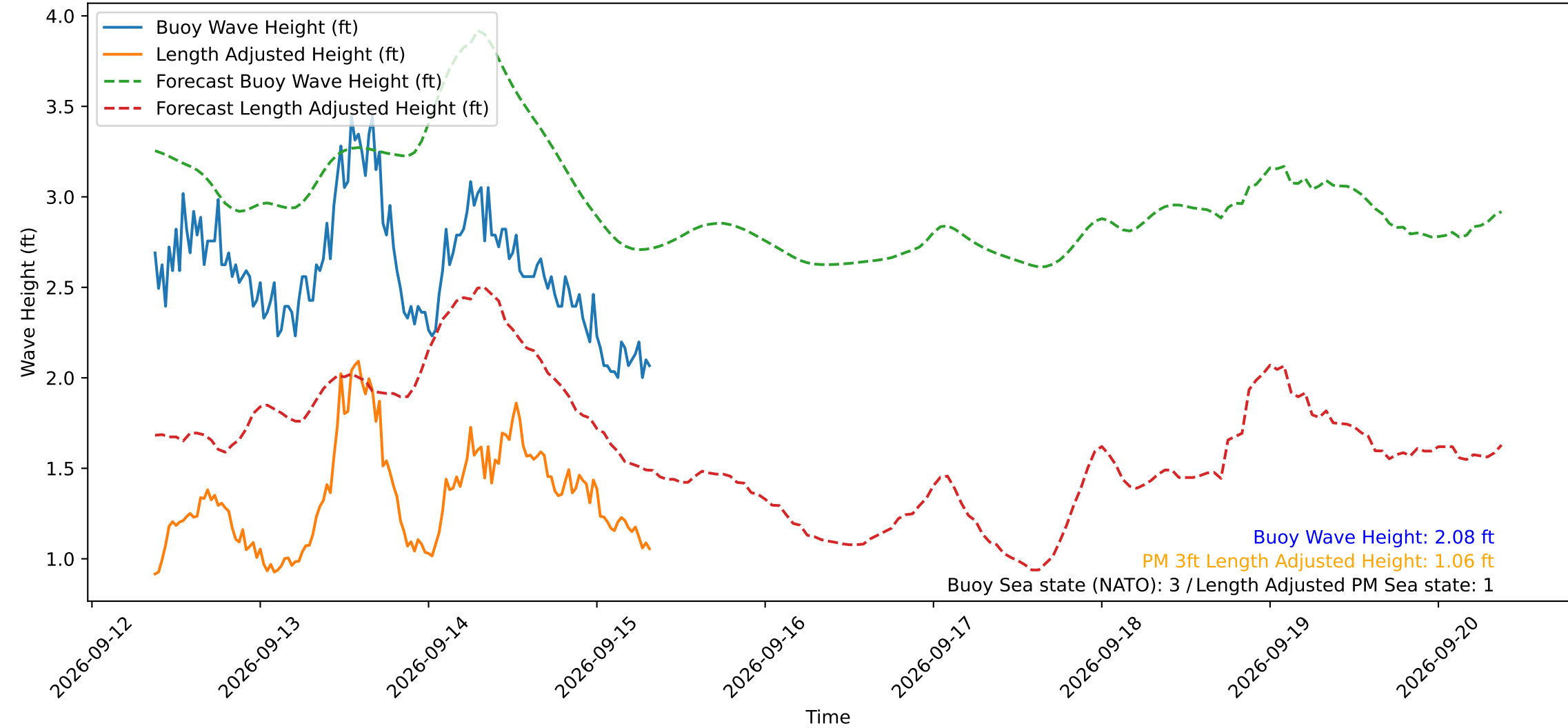
Wave Heights over Time for Red Beach at 2026-09-15 08:30:49
