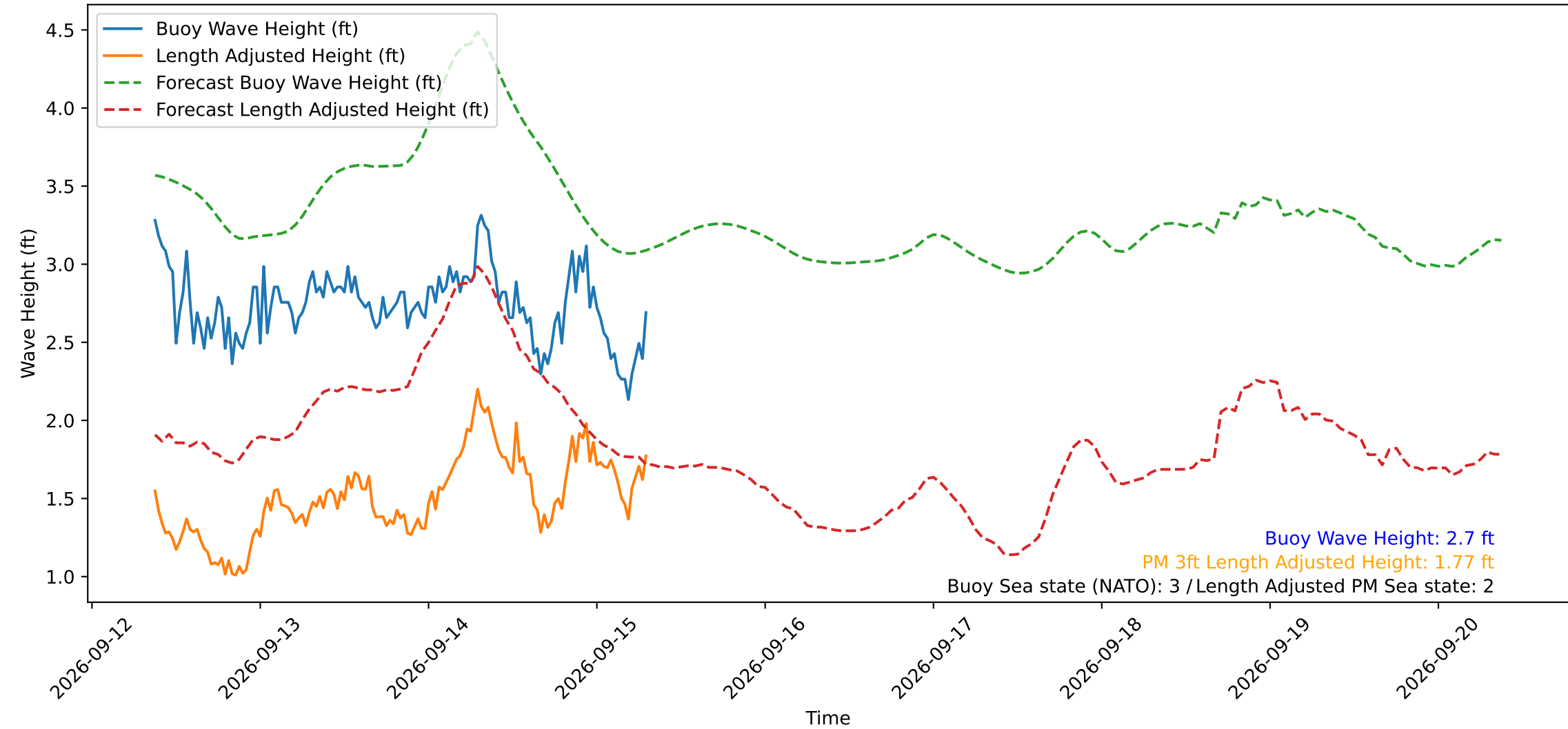
Wave Heights over Time for Green Beach at 2026-09-15 08:31:11
