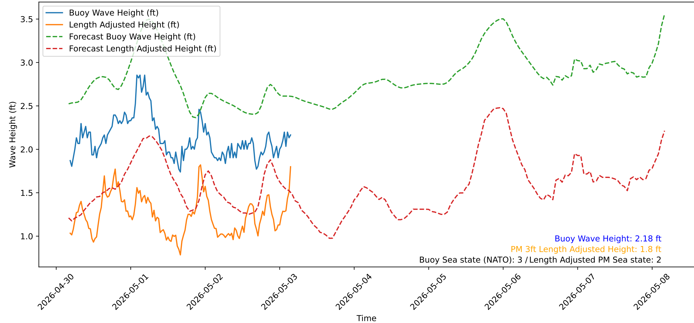
Wave Heights over Time for Green Beach at 2026-05-03 04:21:15
