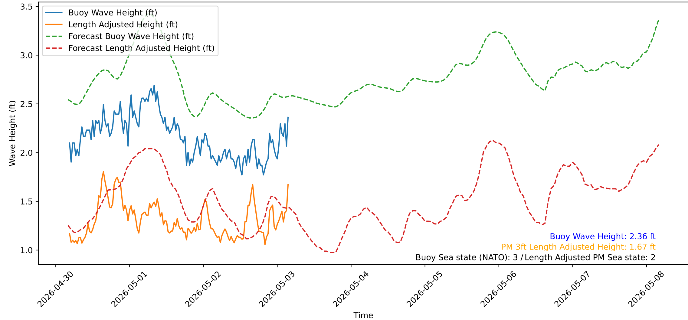
Wave Heights over Time for Oceanside Harbor at 2026-05-03 04:20:32
