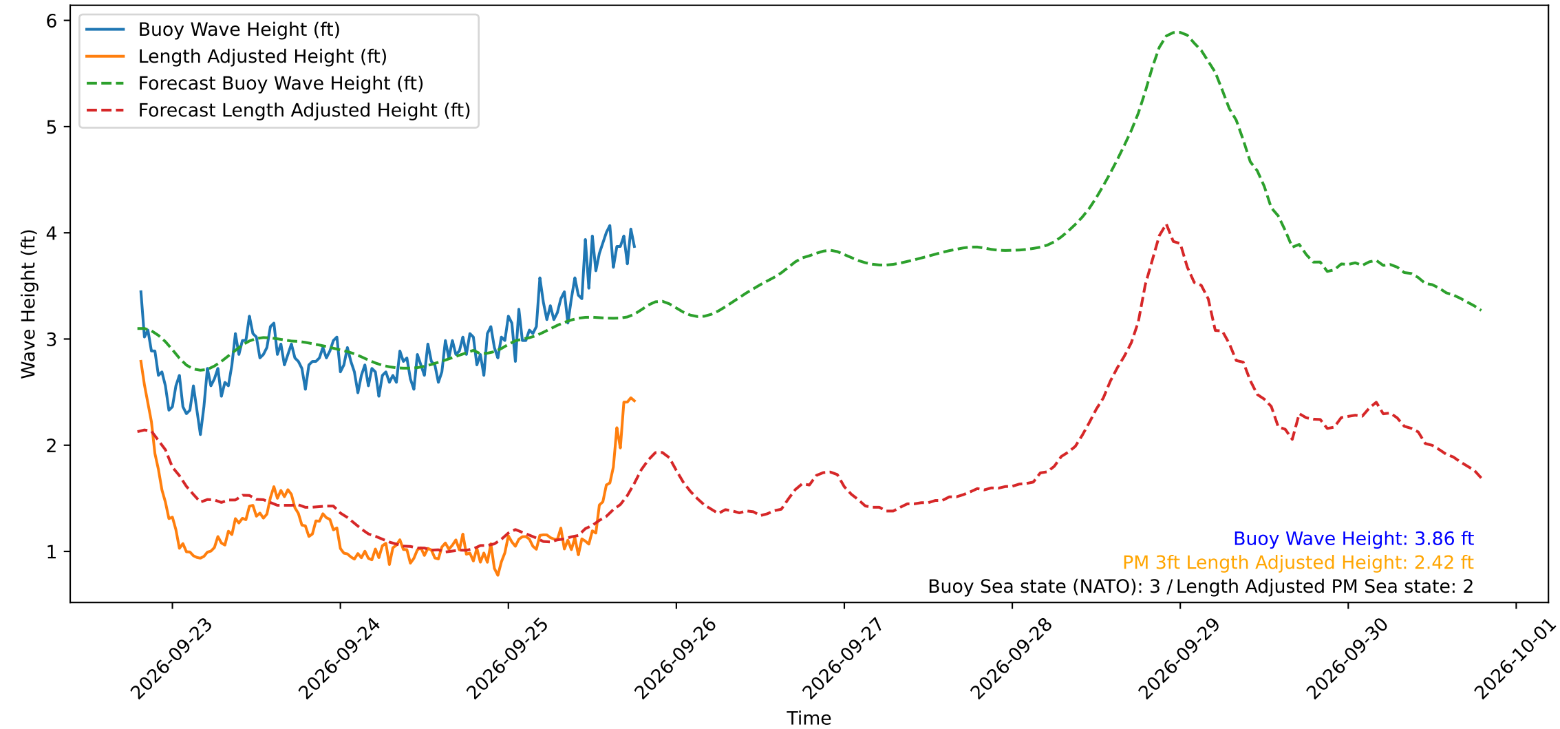
Wave Heights over Time for Green Beach at 2026-09-25 19:01:11
