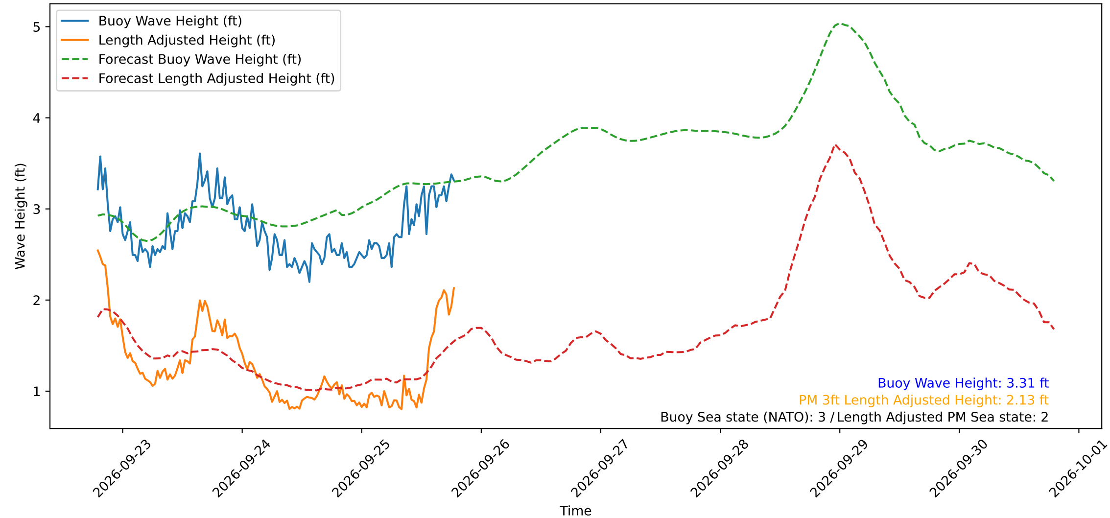
Wave Heights over Time for Oceanside Harbor at 2026-09-25 19:00:30
