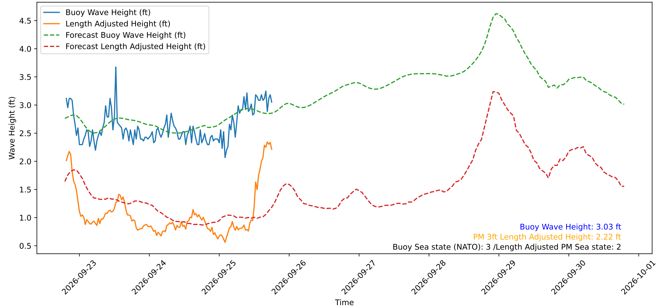
Wave Heights over Time for Red Beach at 2026-09-25 19:00:49
