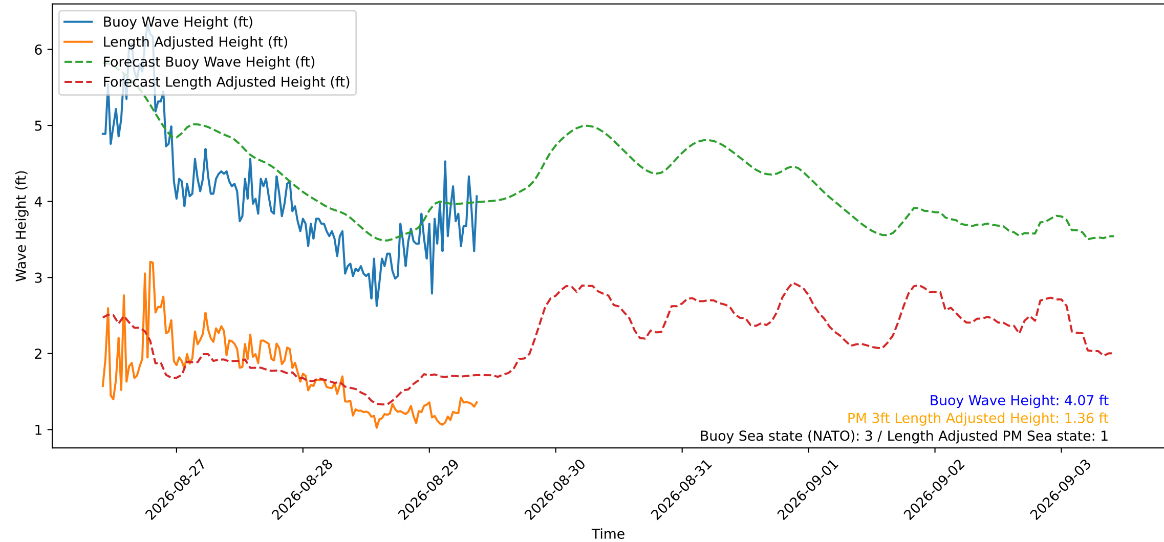
Wave Heights over Time for Green Beach at 2026-08-29 09:51:15
