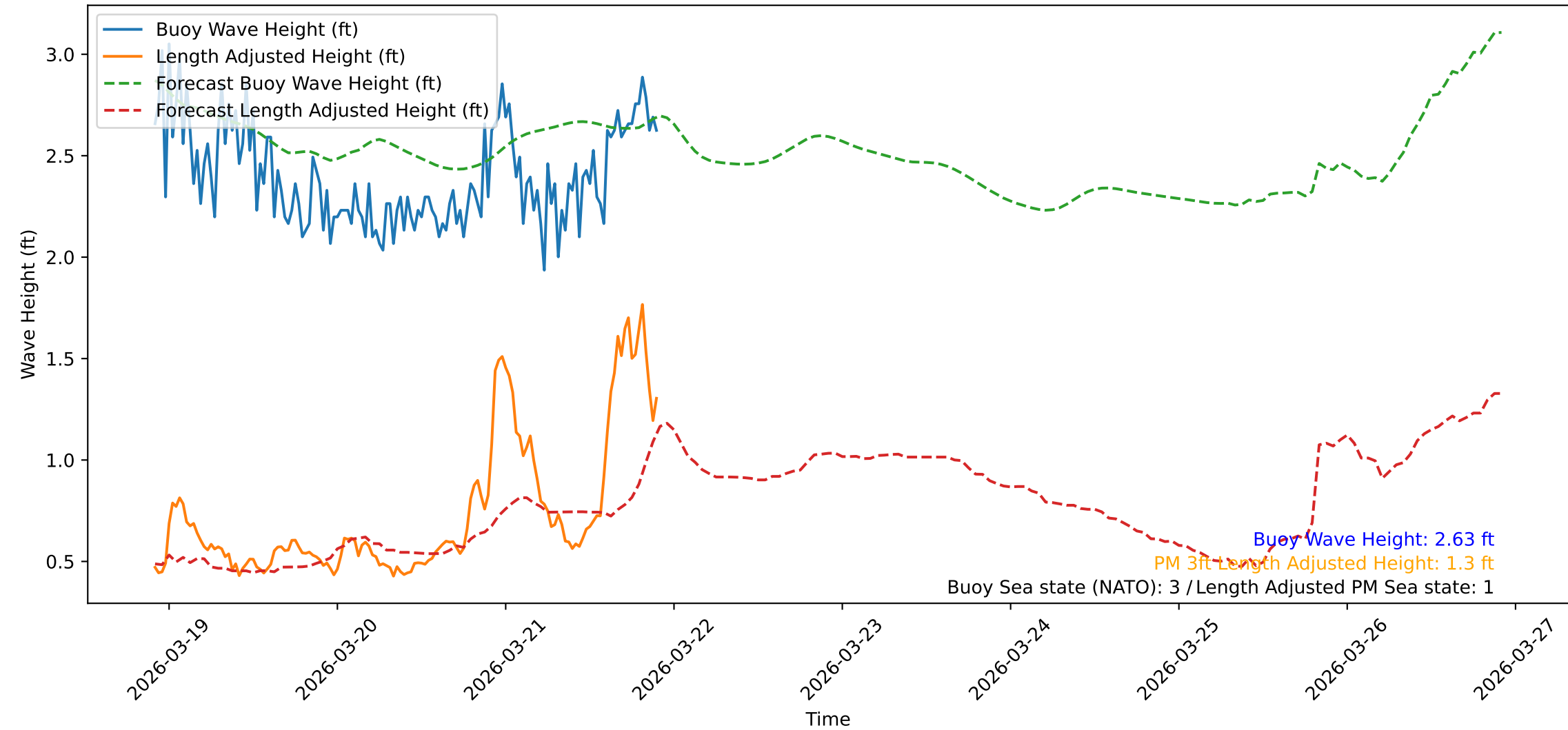
Wave Heights over Time for Green Beach at 2026-03-21 22:11:09
