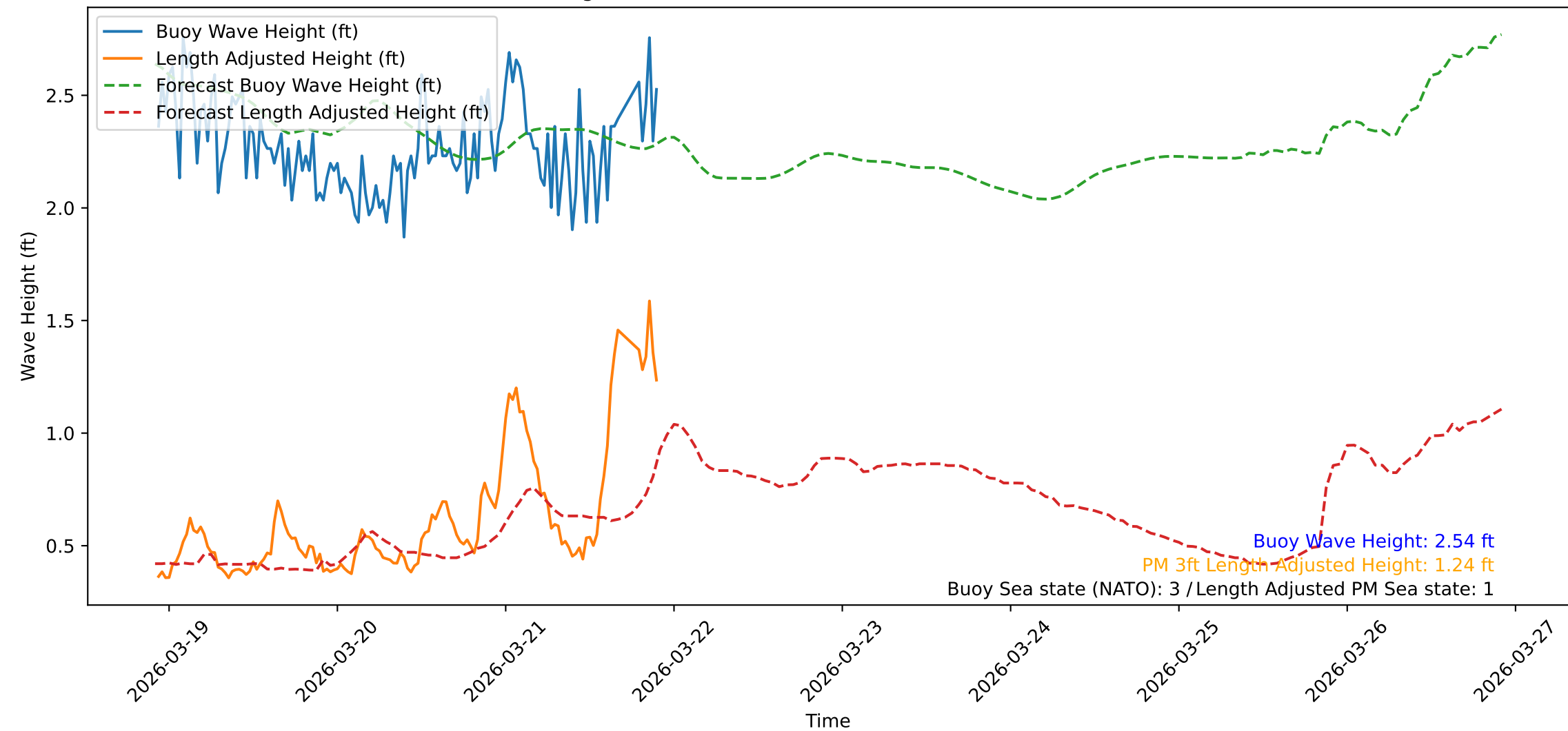
Wave Heights over Time for Red Beach at 2026-03-21 22:10:46
