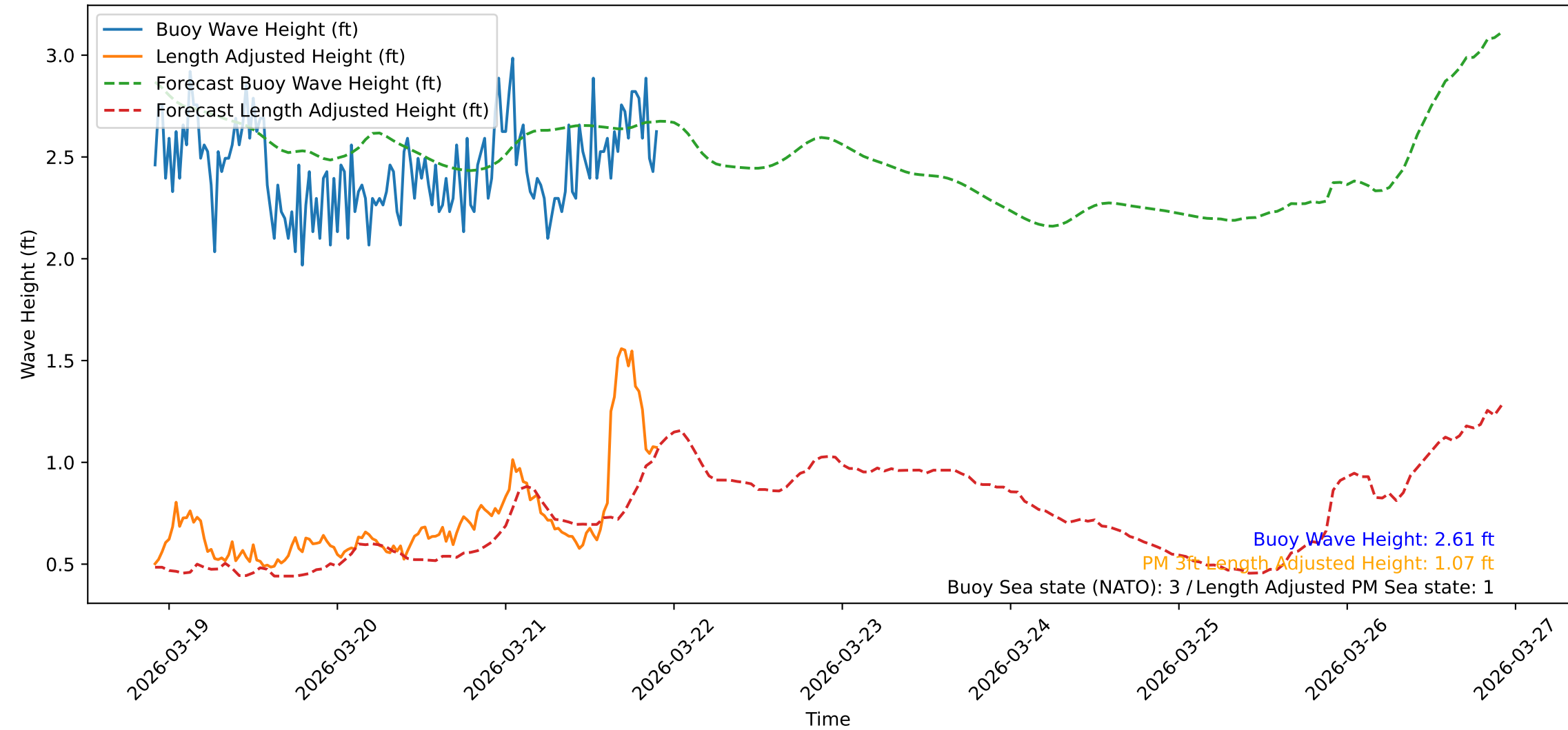
Wave Heights over Time for Oceanside Harbor at 2026-03-21 22:10:31
