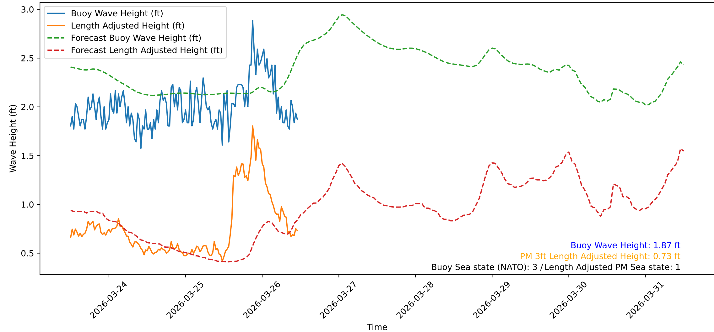
Wave Heights over Time for Oceanside Harbor at 2026-03-26 12:00:31
