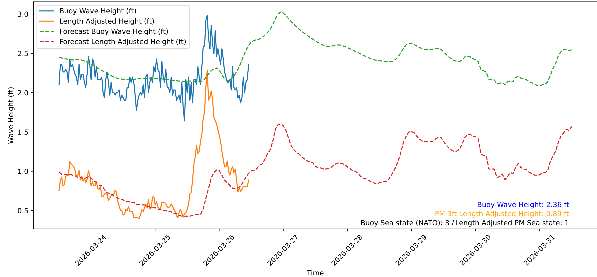
Wave Heights over Time for Green Beach at 2026-03-26 12:01:09
