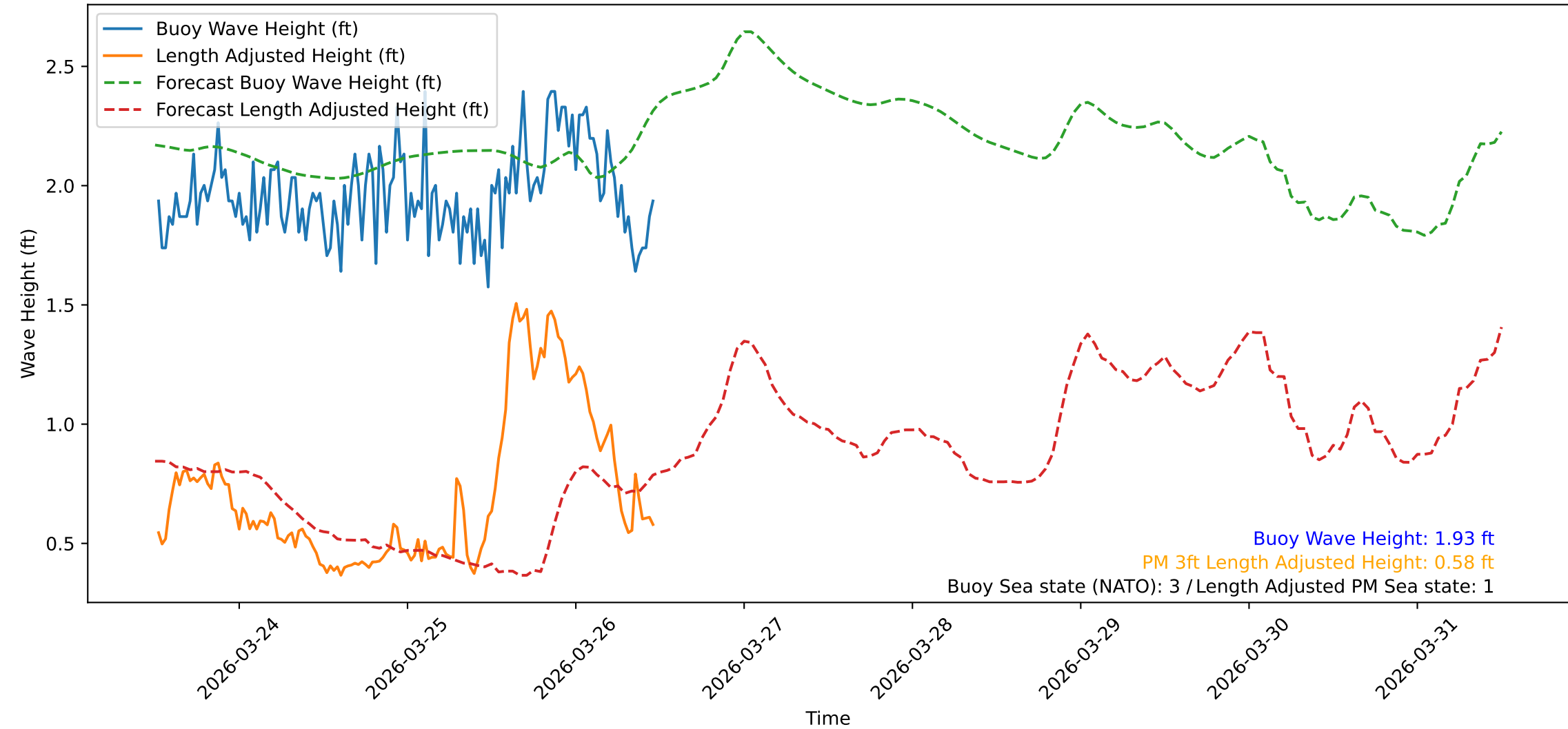
Wave Heights over Time for Red Beach at 2026-03-26 12:00:47
