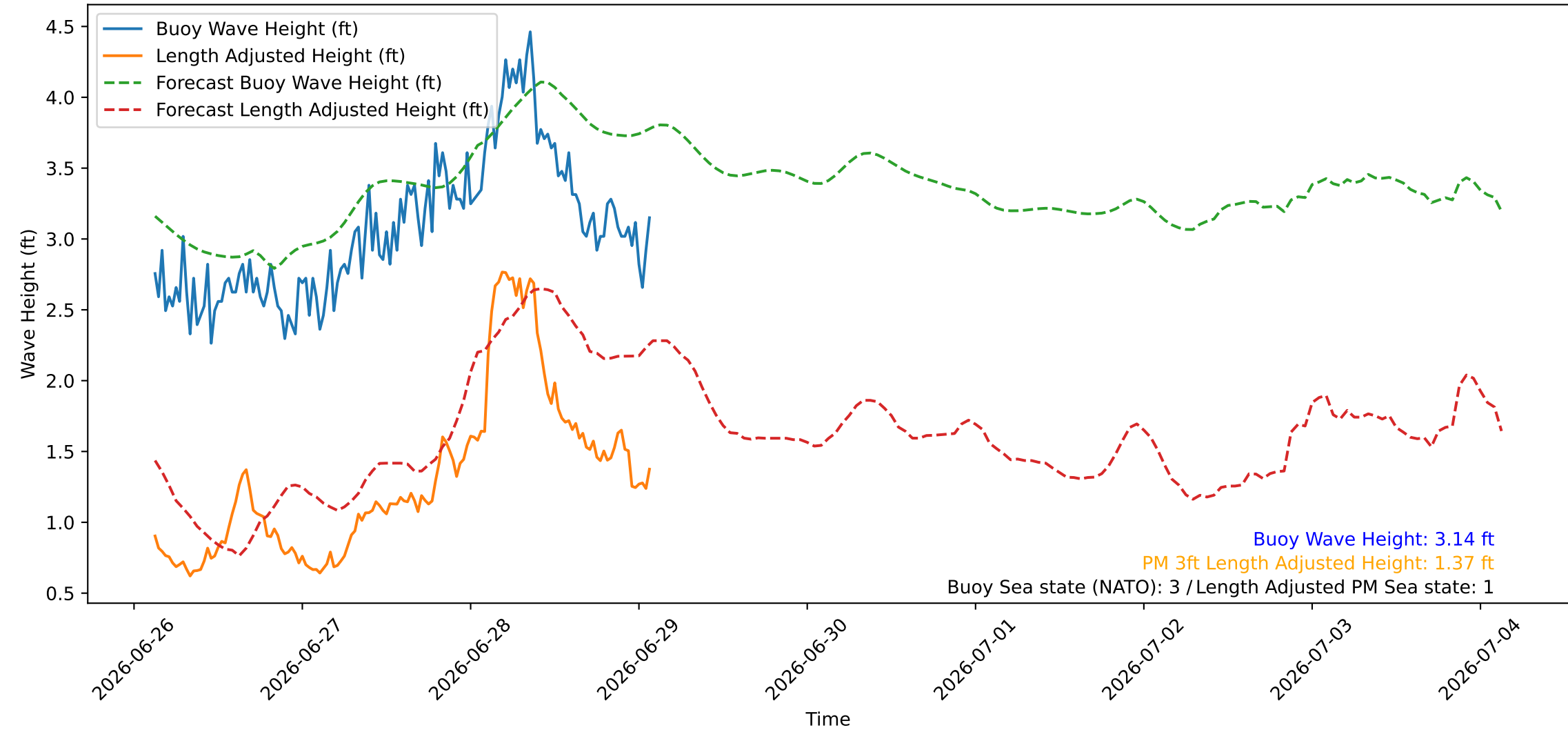
Wave Heights over Time for Red Beach at 2026-06-29 02:30:45
