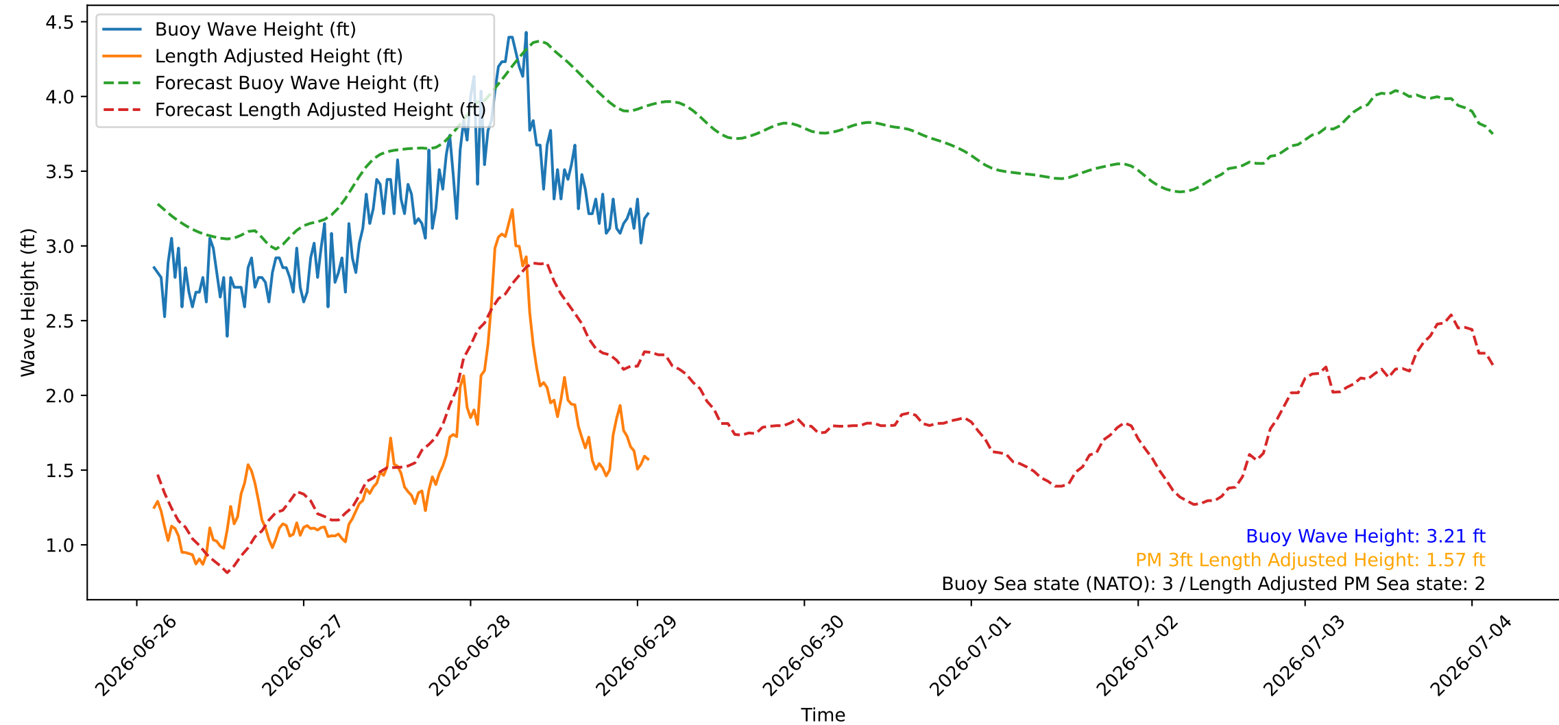
Wave Heights over Time for Oceanside Harbor at 2026-06-29 02:30:26
