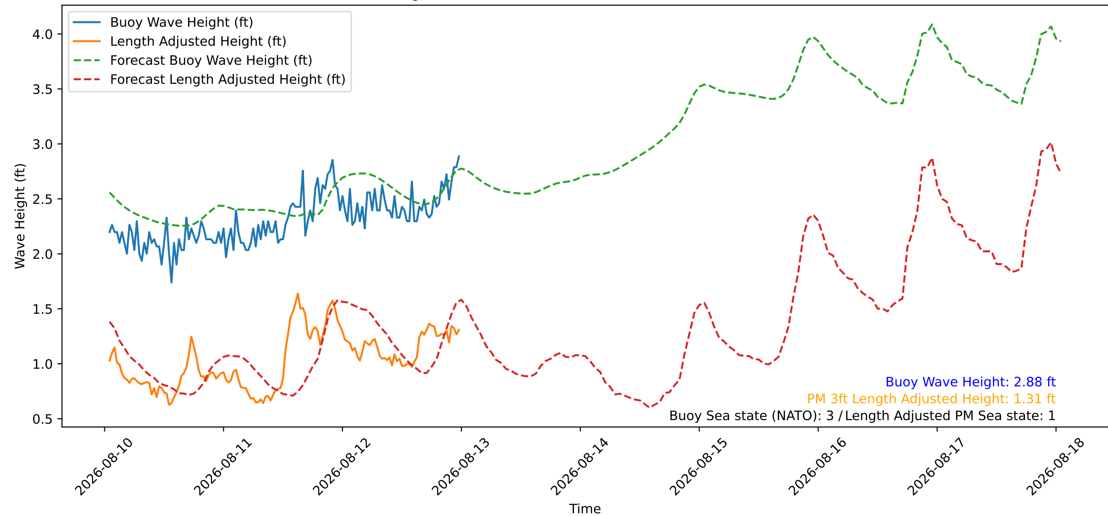
Wave Heights over Time for Red Beach at 2026-08-13 00:30:46
