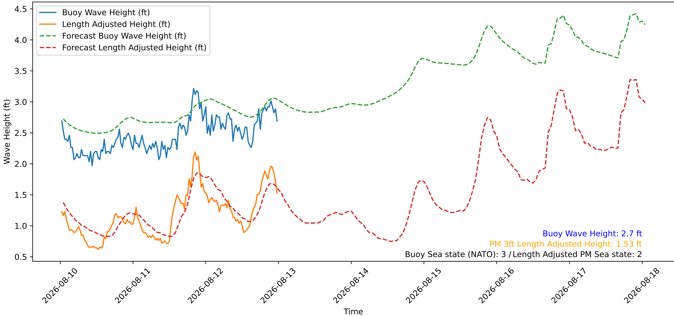
Wave Heights over Time for Green Beach at 2026-08-13 00:31:09
