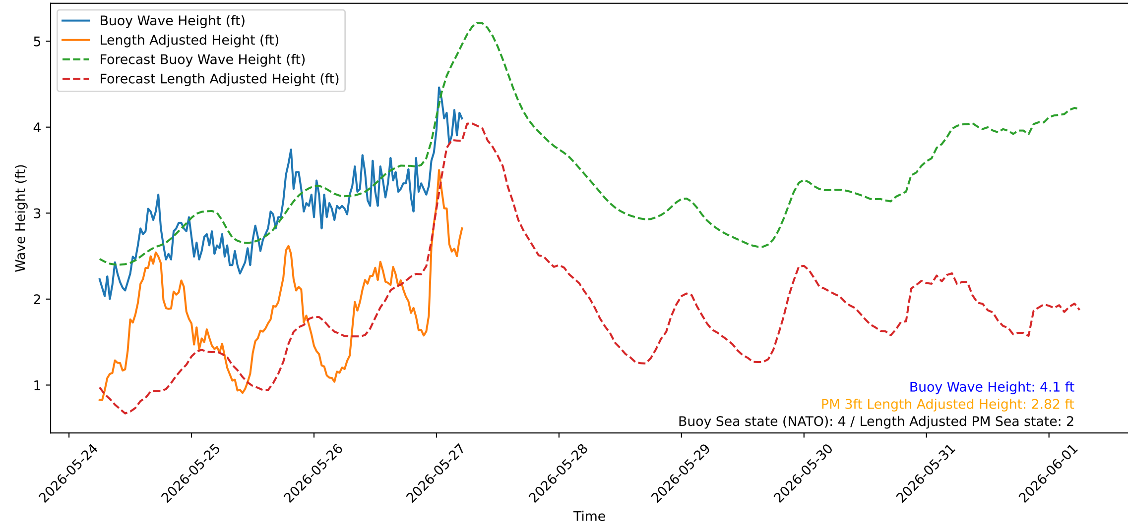
Wave Heights over Time for Red Beach at 2026-05-27 05:50:46
