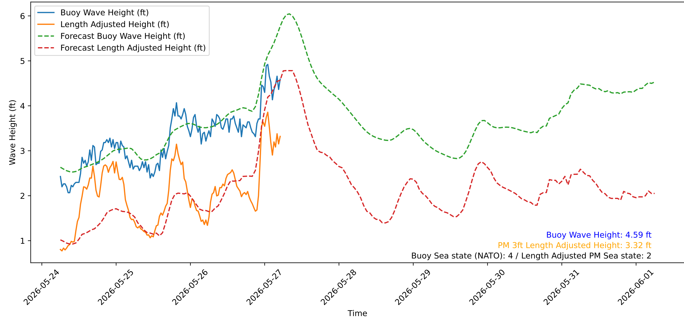
Wave Heights over Time for Green Beach at 2026-05-27 05:51:09
