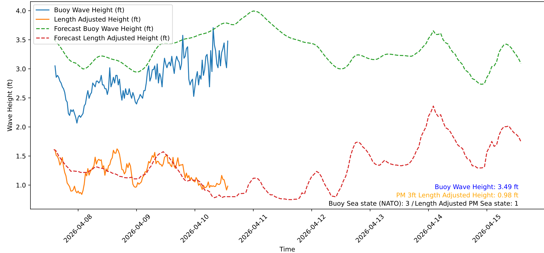
Wave Heights over Time for Red Beach at 2026-04-10 14:10:50
