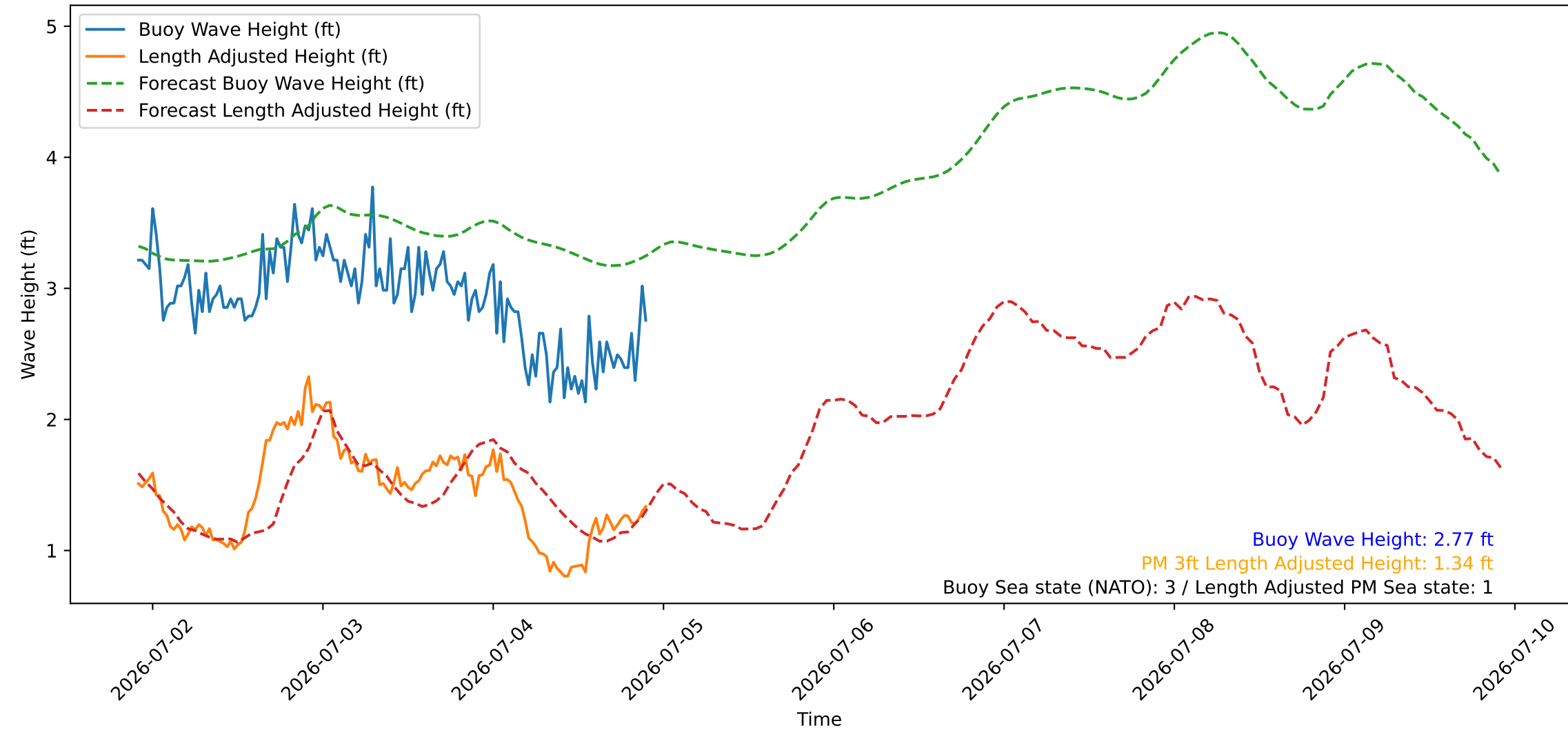
Wave Heights over Time for Oceanside Harbor at 2026-07-04 22:10:27
