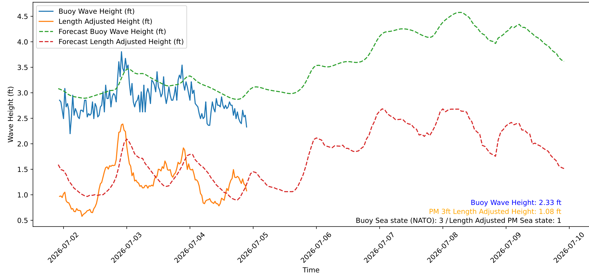
Wave Heights over Time for Red Beach at 2026-07-04 22:10:47
