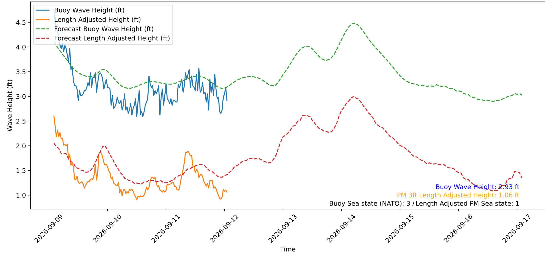
Wave Heights over Time for Green Beach at 2026-09-12 01:41:12
