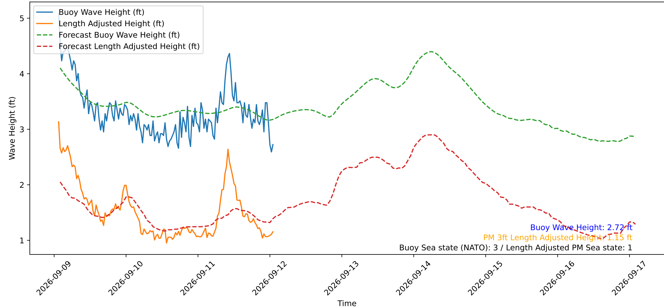
Wave Heights over Time for Oceanside Harbor at 2026-09-12 01:40:30
