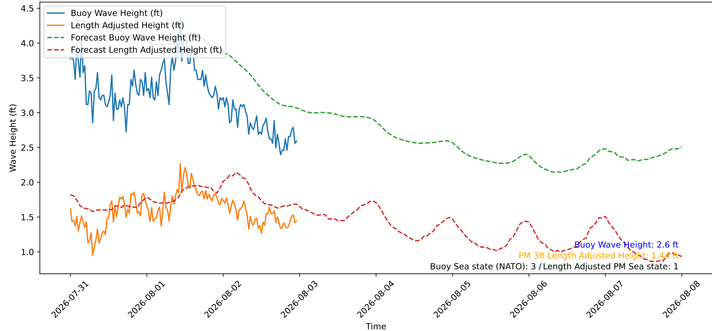
Wave Heights over Time for Oceanside Harbor at 2026-08-03 00:00:26
