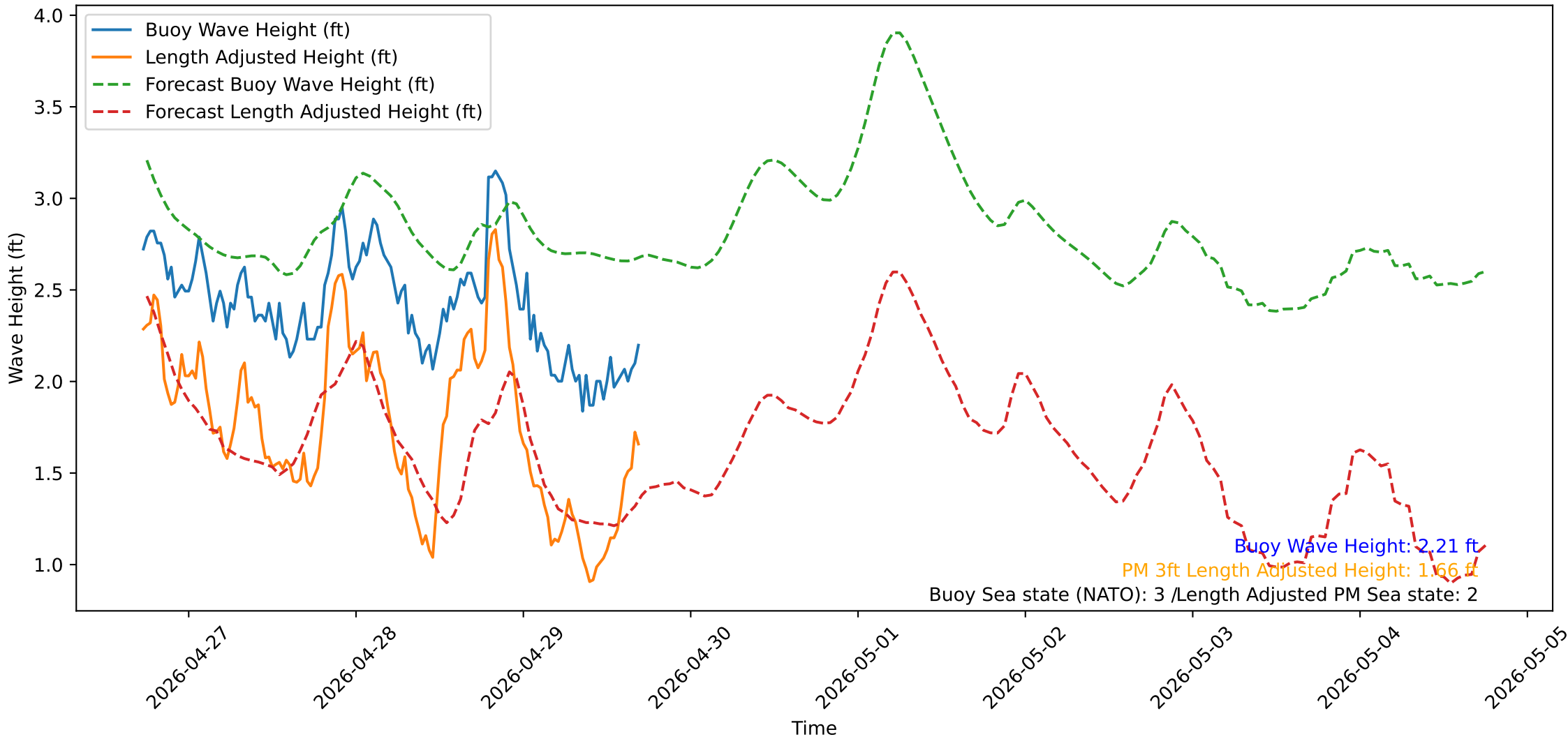
Wave Heights over Time for Green Beach at 2026-04-29 17:31:12
