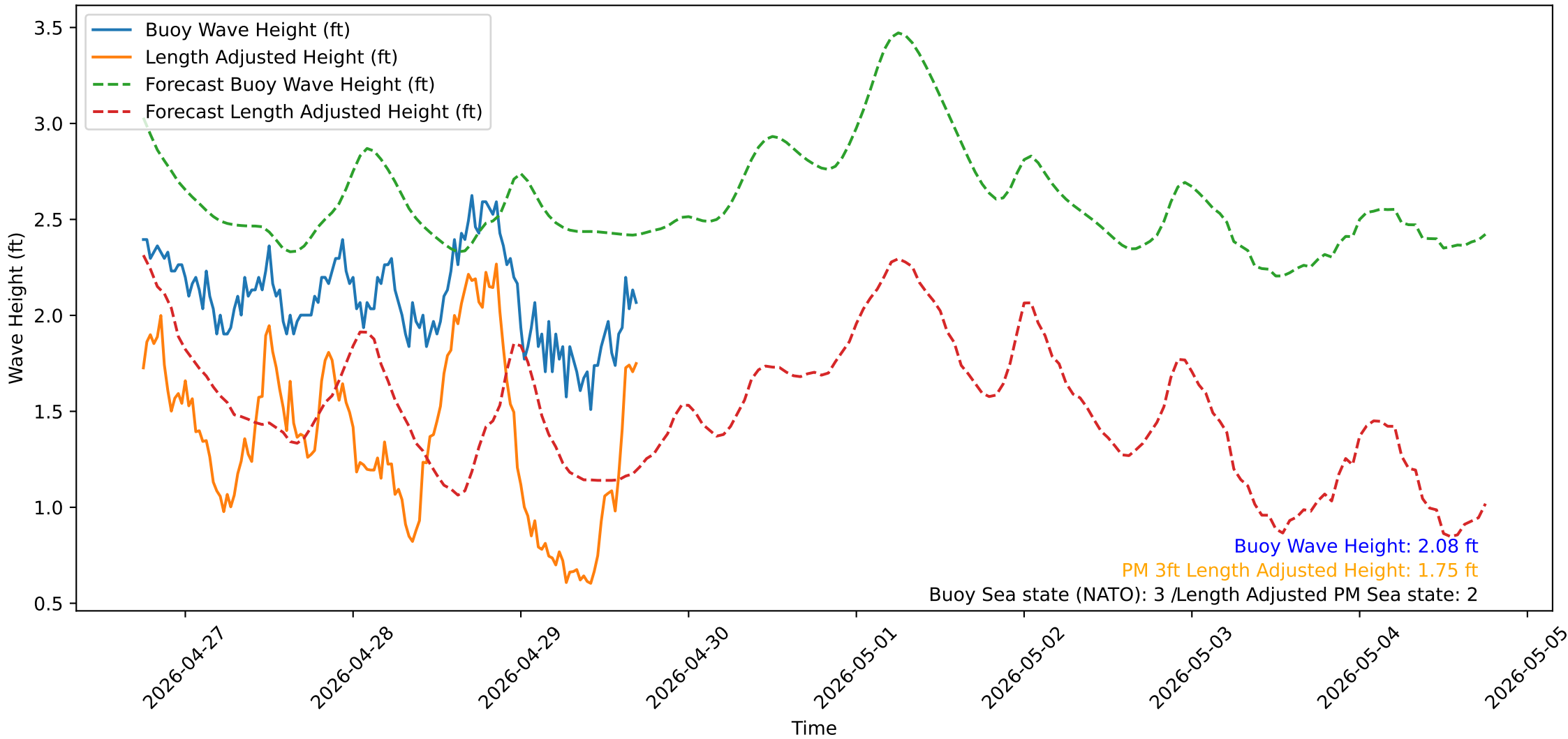
Wave Heights over Time for Red Beach at 2026-04-29 17:30:50
