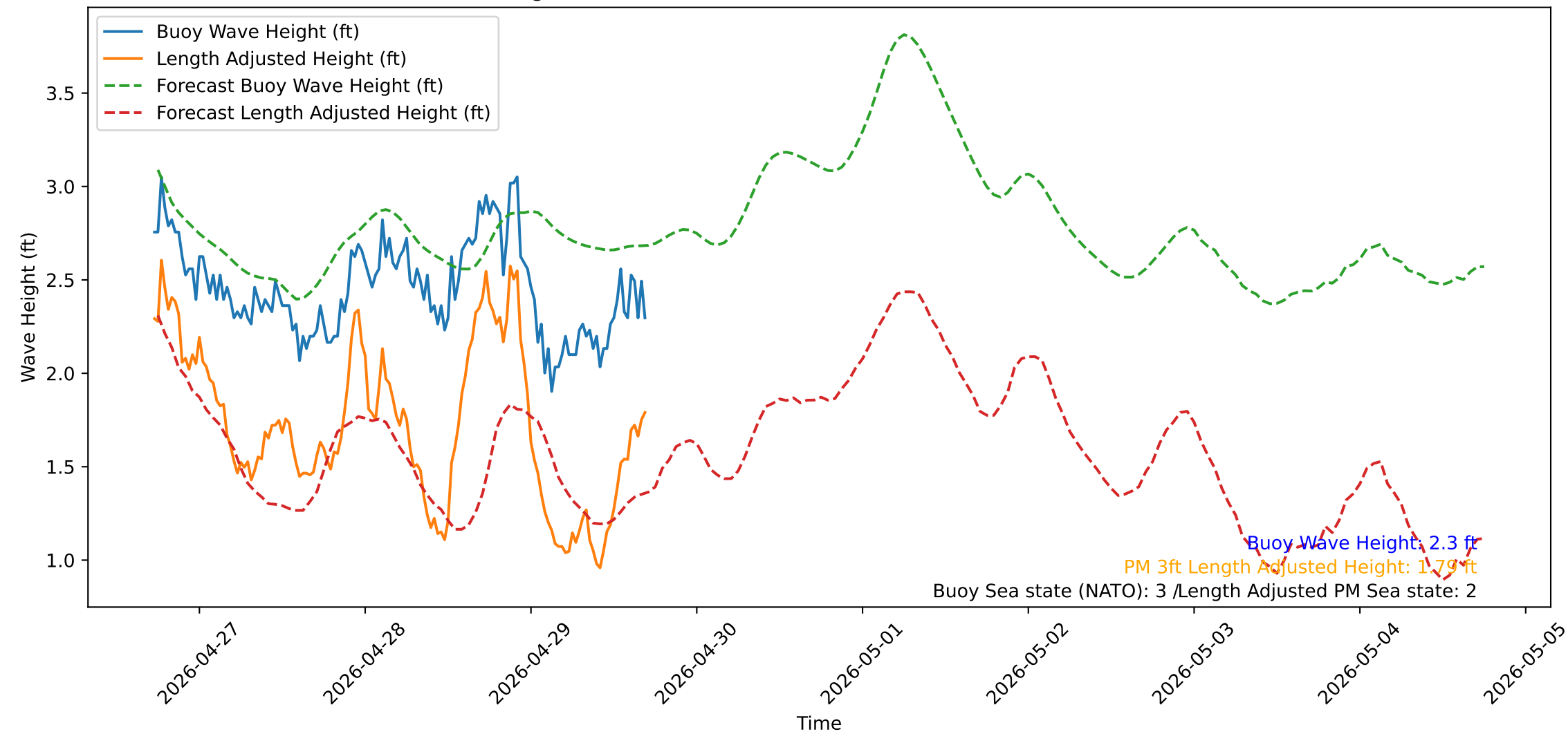
Wave Heights over Time for Oceanside Harbor at 2026-04-29 17:30:31
