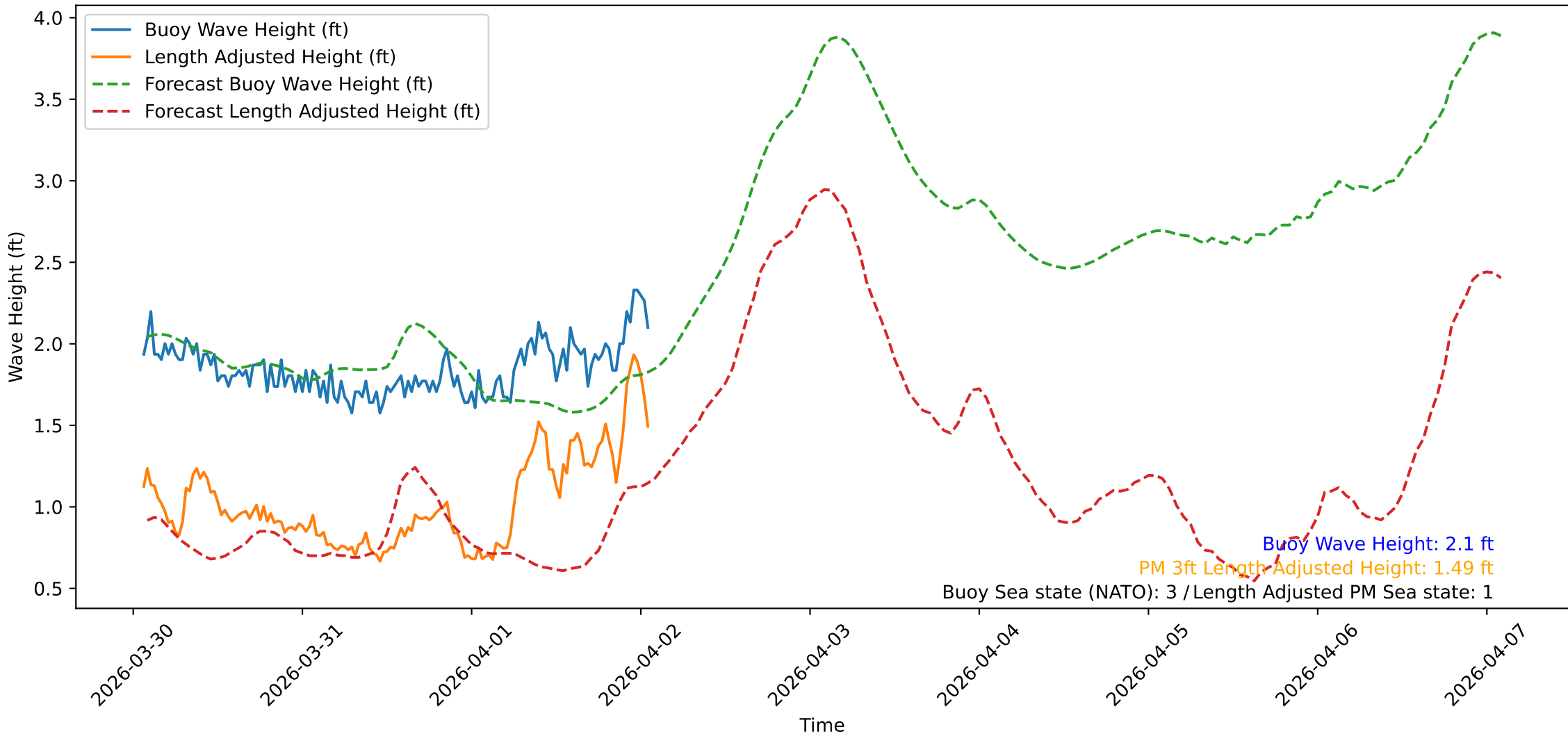
Wave Heights over Time for Oceanside Harbor at 2026-04-02 01:30:32
