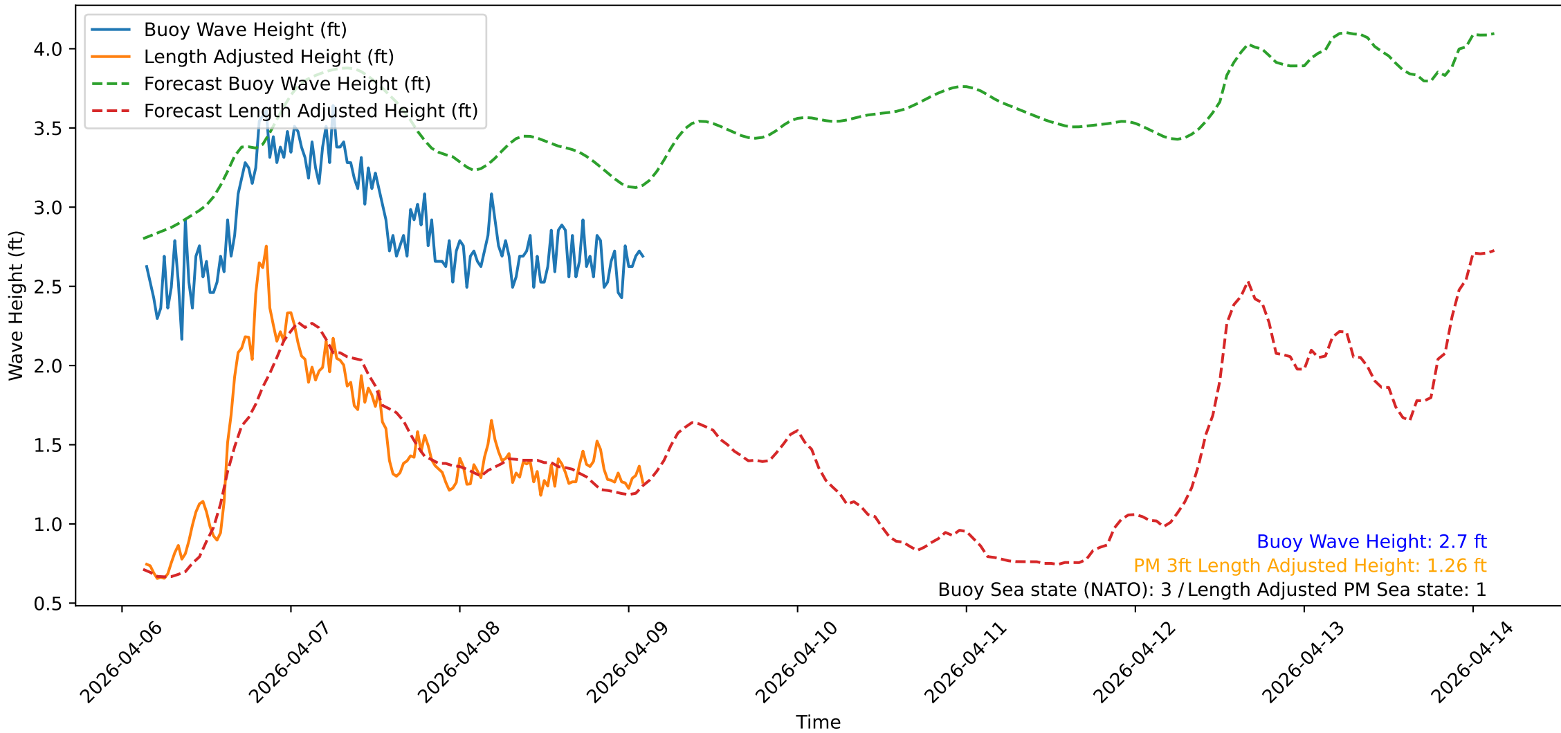
Wave Heights over Time for Oceanside Harbor at 2026-04-09 03:20:31
