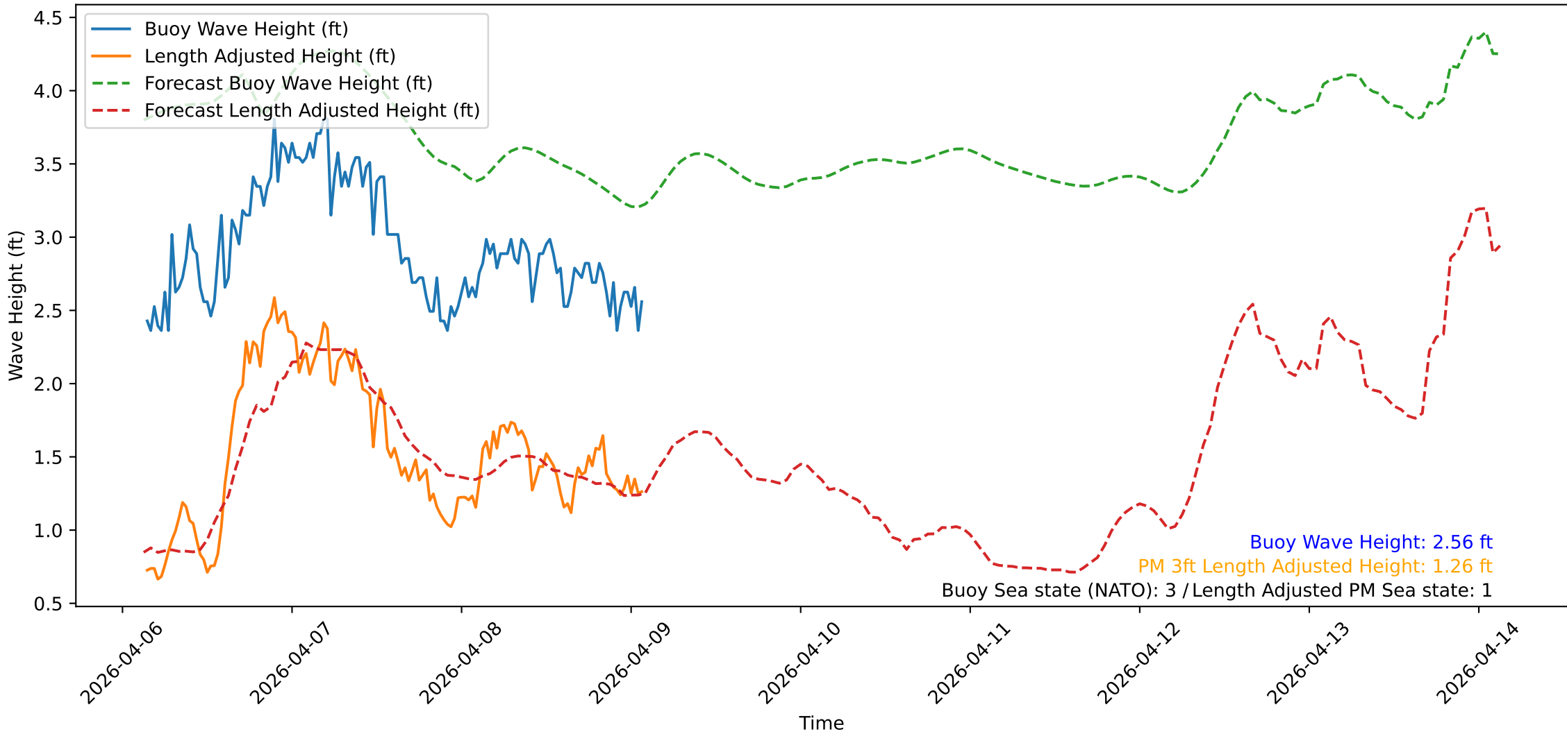
Wave Heights over Time for Green Beach at 2026-04-09 03:21:09
