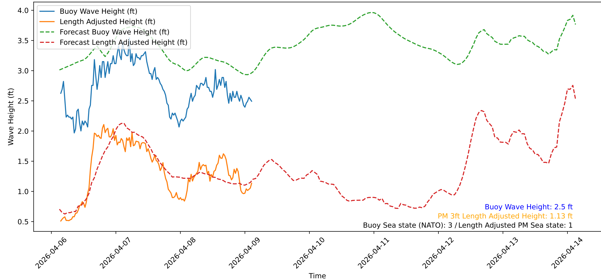
Wave Heights over Time for Red Beach at 2026-04-09 03:20:47
