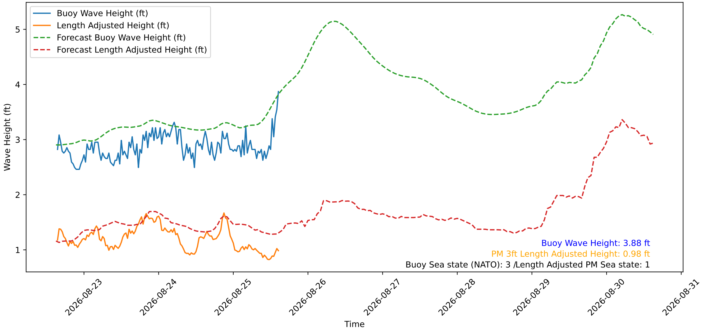
Wave Heights over Time for Green Beach at 2026-08-25 15:21:15
