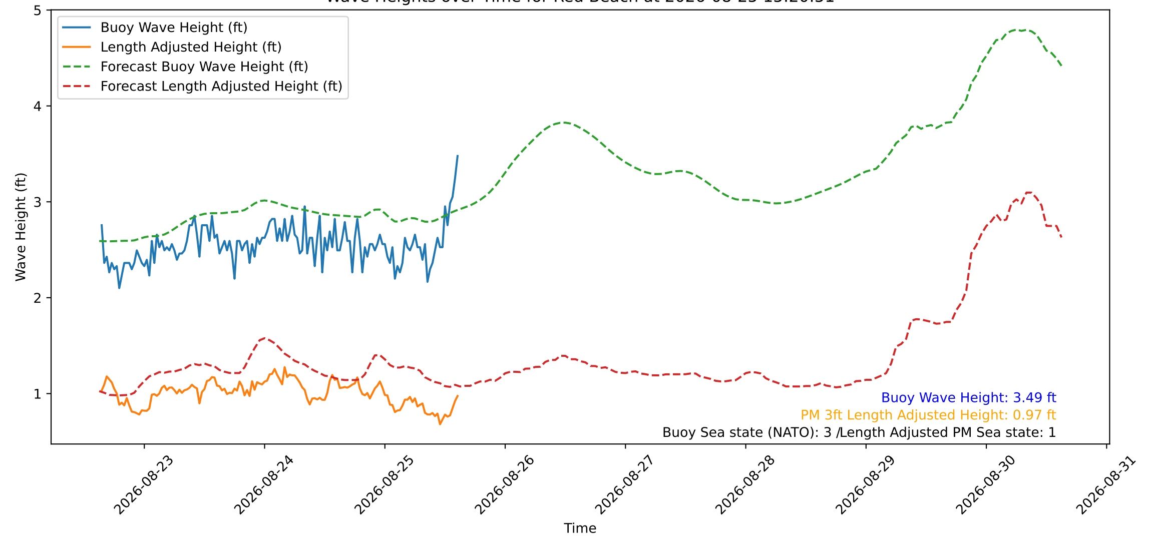
Wave Heights over Time for Red Beach at 2026-08-25 15:20:51
