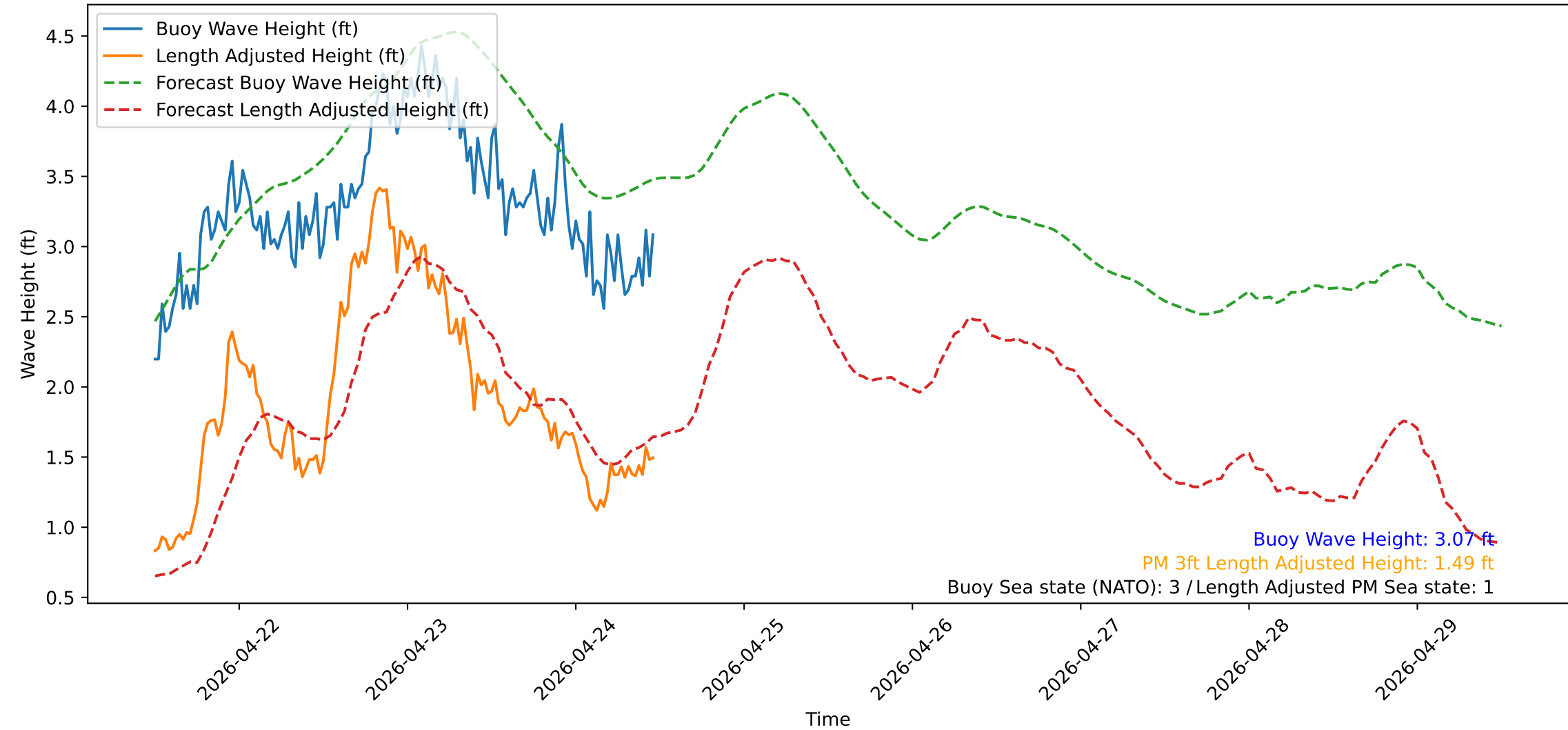
Wave Heights over Time for Oceanside Harbor at 2026-04-24 12:00:31
