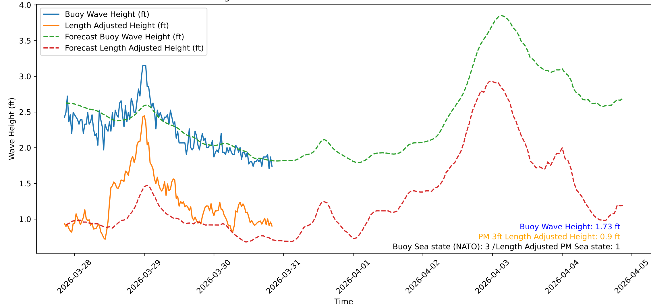
Wave Heights over Time for Oceanside Harbor at 2026-03-30 20:30:32
