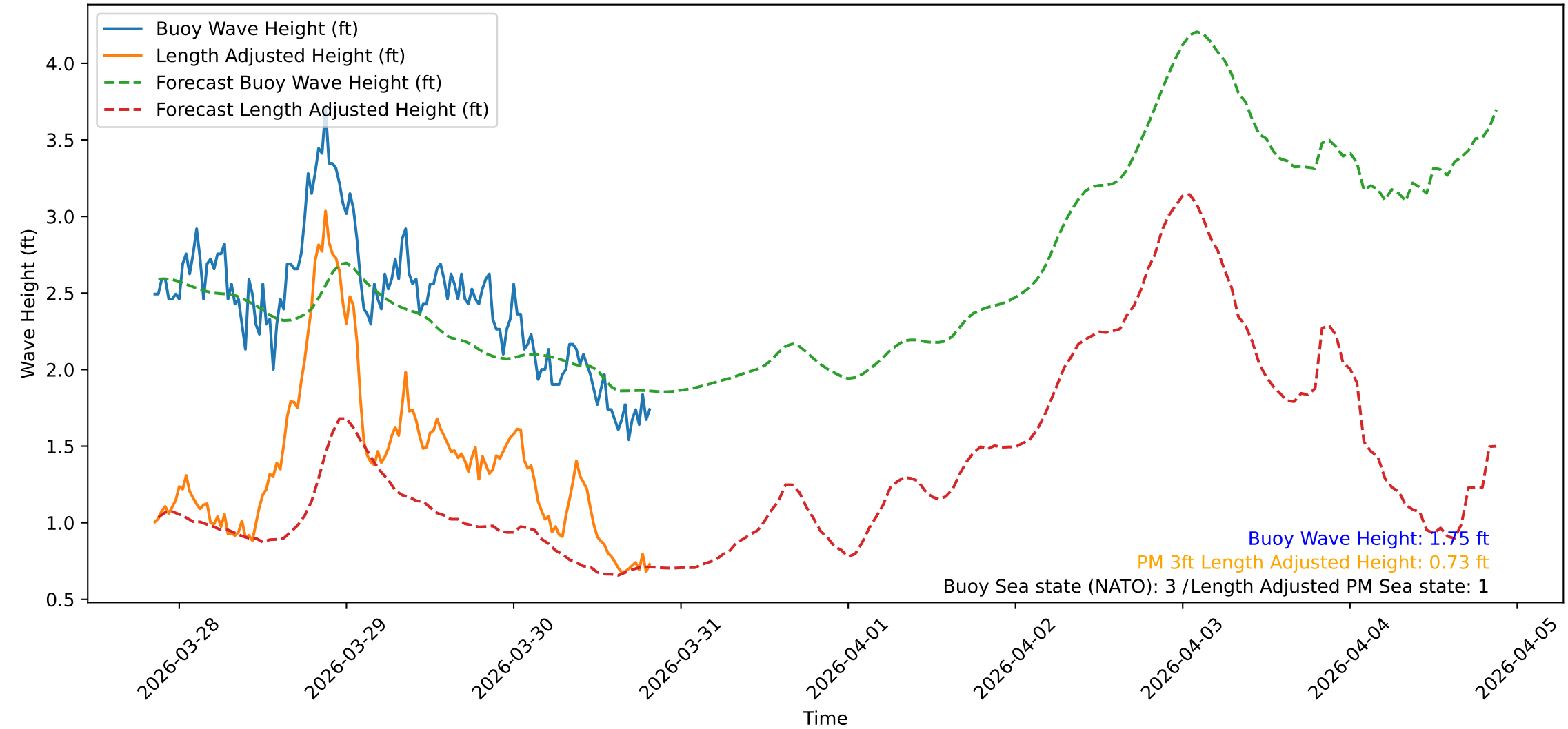
Wave Heights over Time for Green Beach at 2026-03-30 20:31:10
