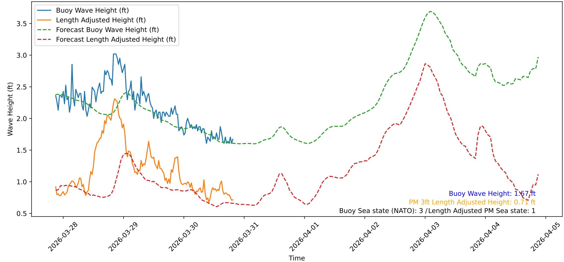
Wave Heights over Time for Red Beach at 2026-03-30 20:30:48
