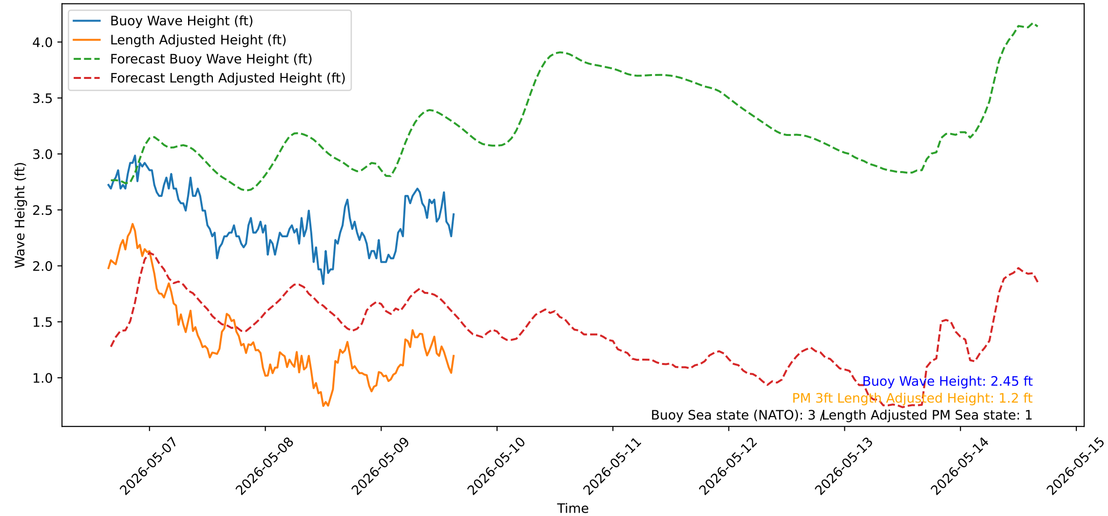
Wave Heights over Time for Green Beach at 2026-05-09 15:41:13
