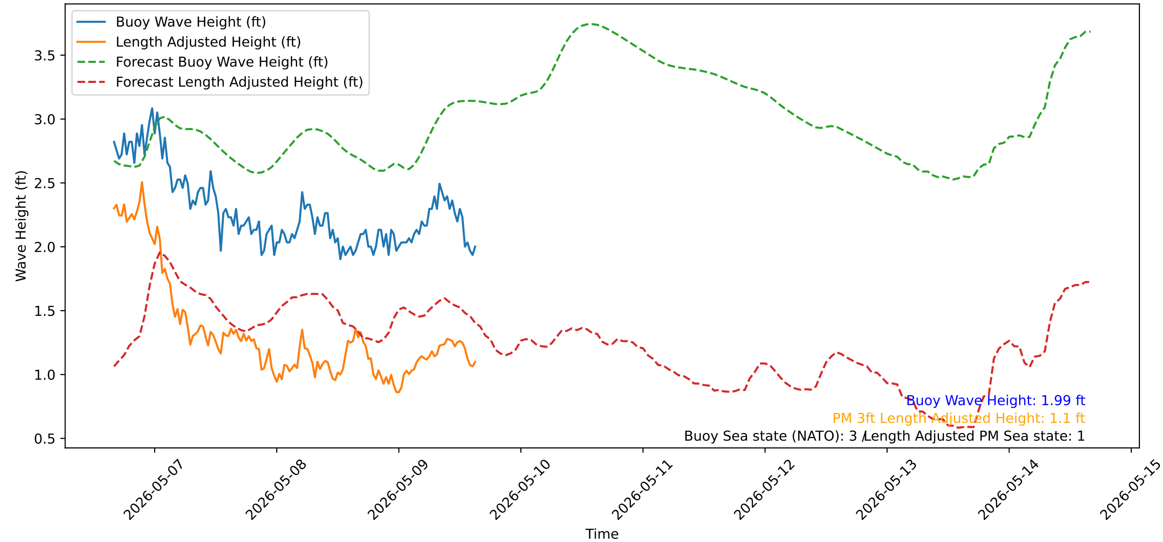
Wave Heights over Time for Red Beach at 2026-05-09 15:40:50
