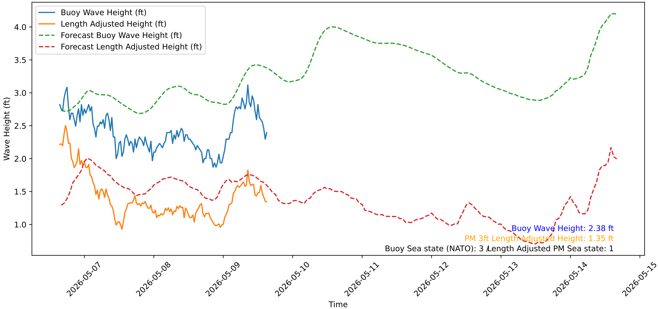
Wave Heights over Time for Oceanside Harbor at 2026-05-09 15:40:31
