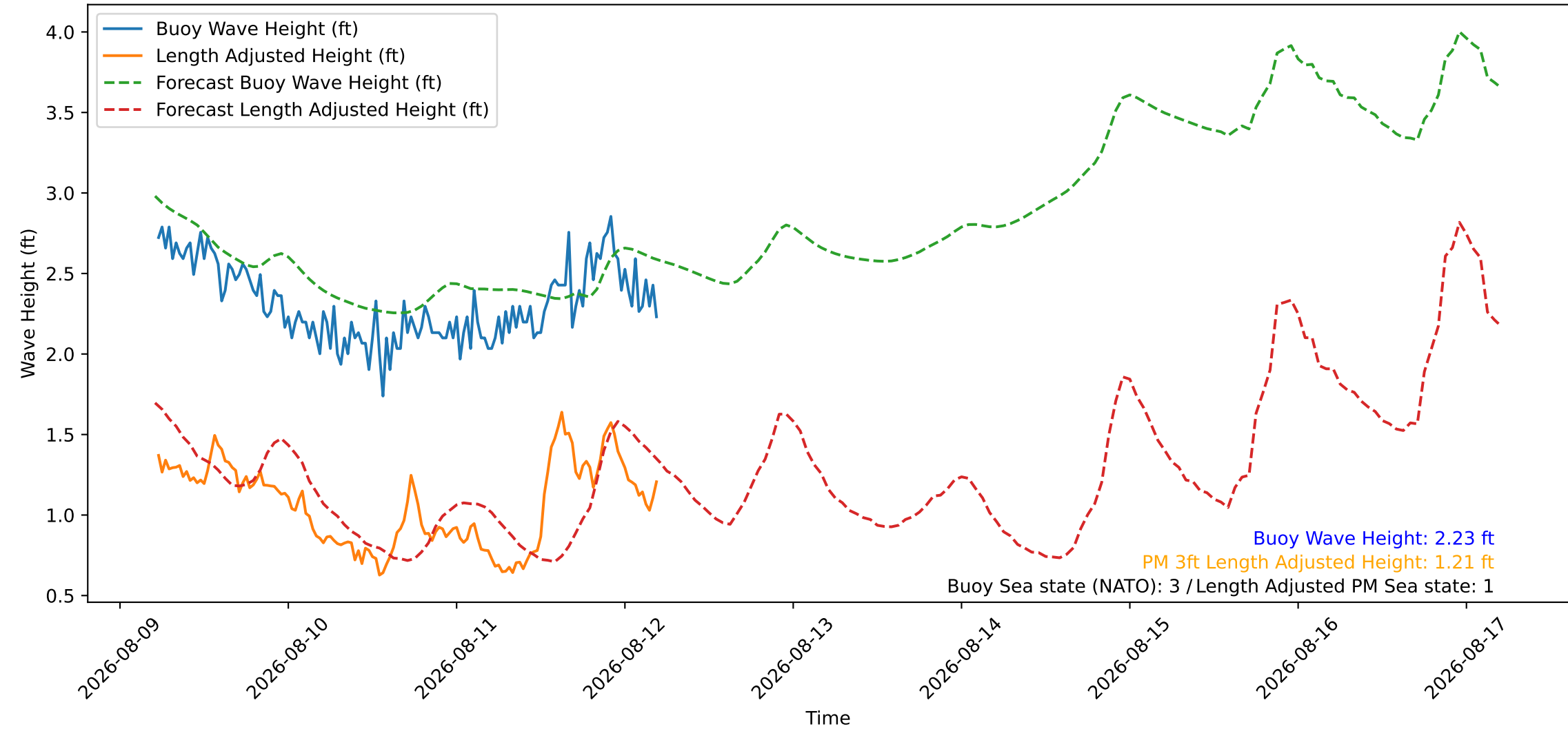
Wave Heights over Time for Red Beach at 2026-08-12 05:20:47
