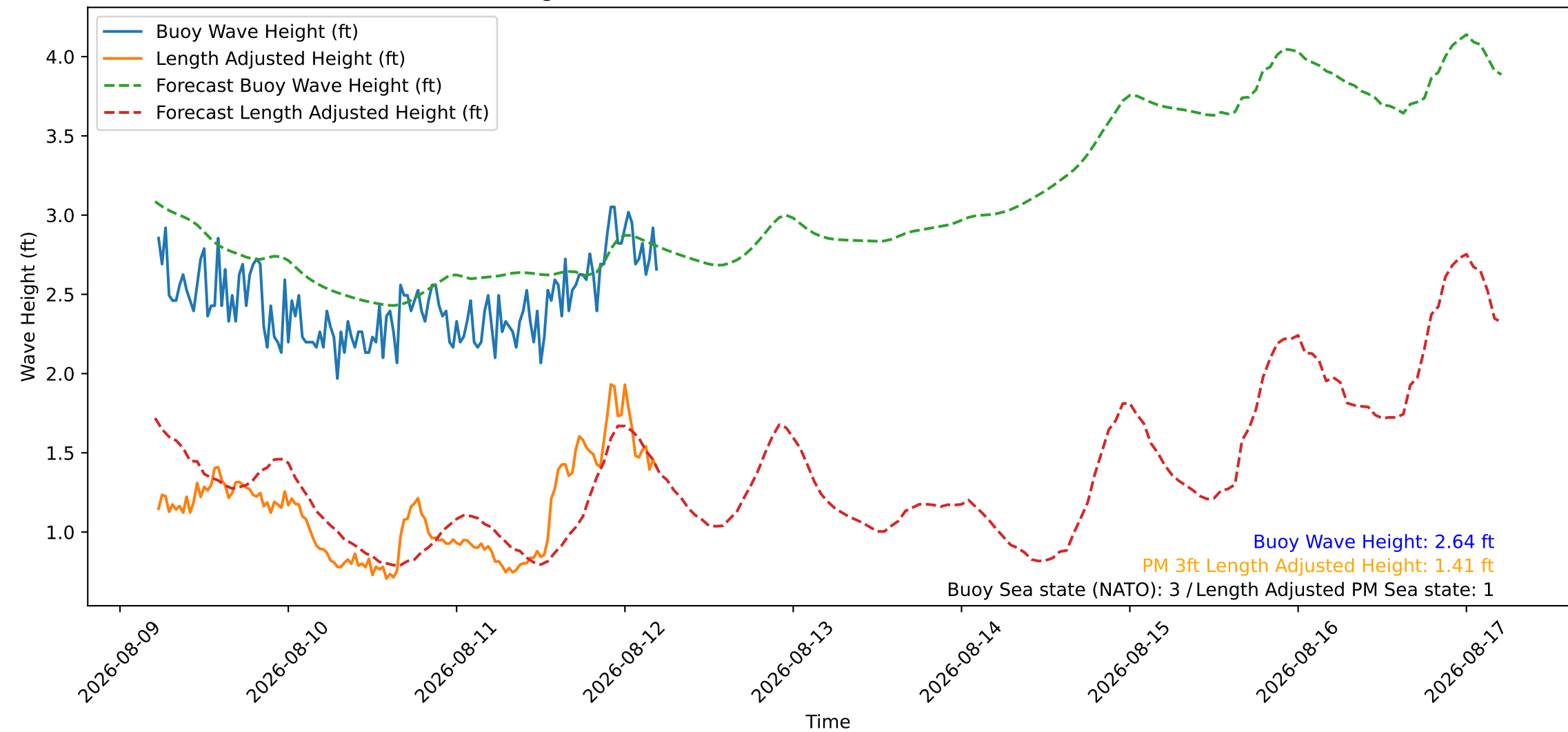
Wave Heights over Time for Oceanside Harbor at 2026-08-12 05:20:26
