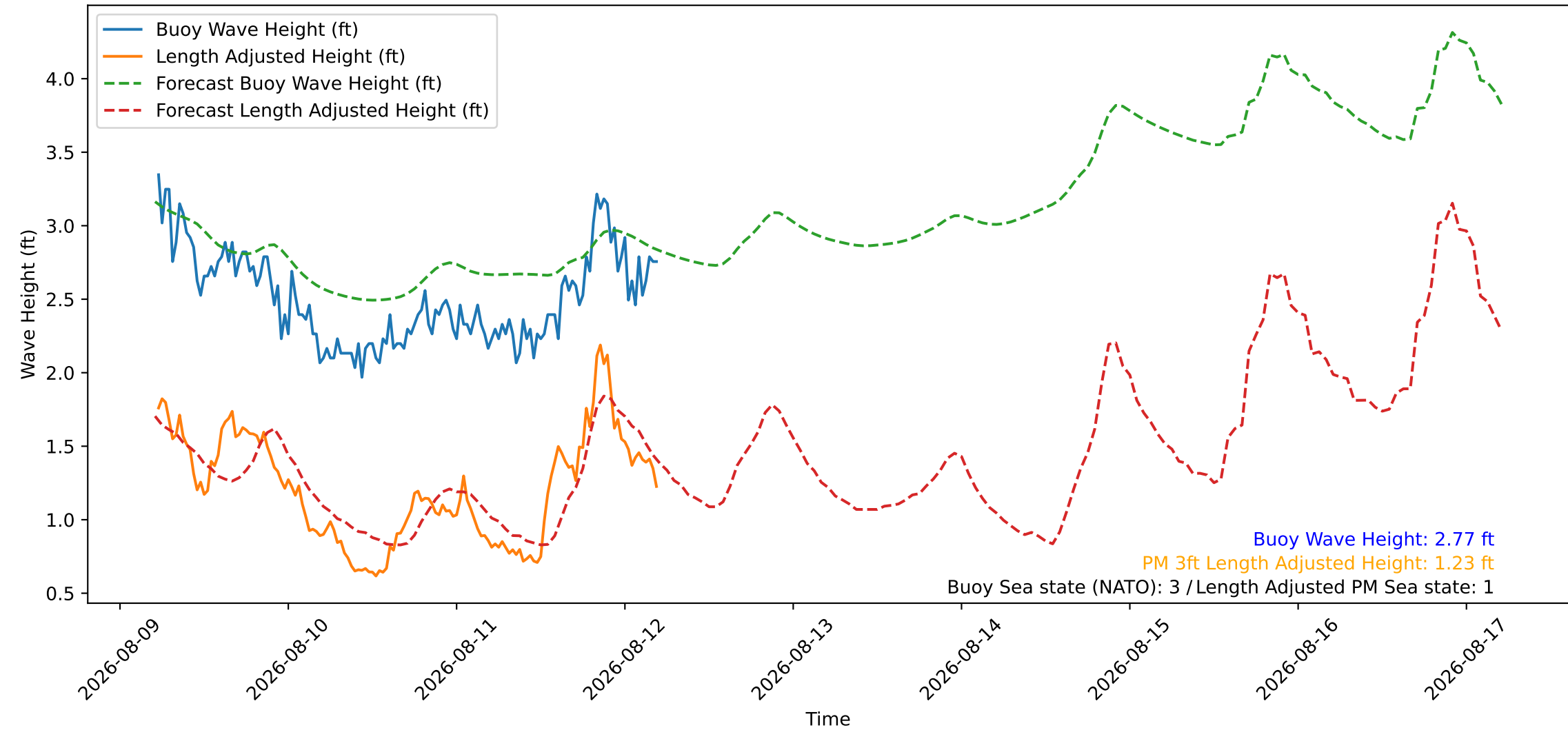
Wave Heights over Time for Green Beach at 2026-08-12 05:21:10
