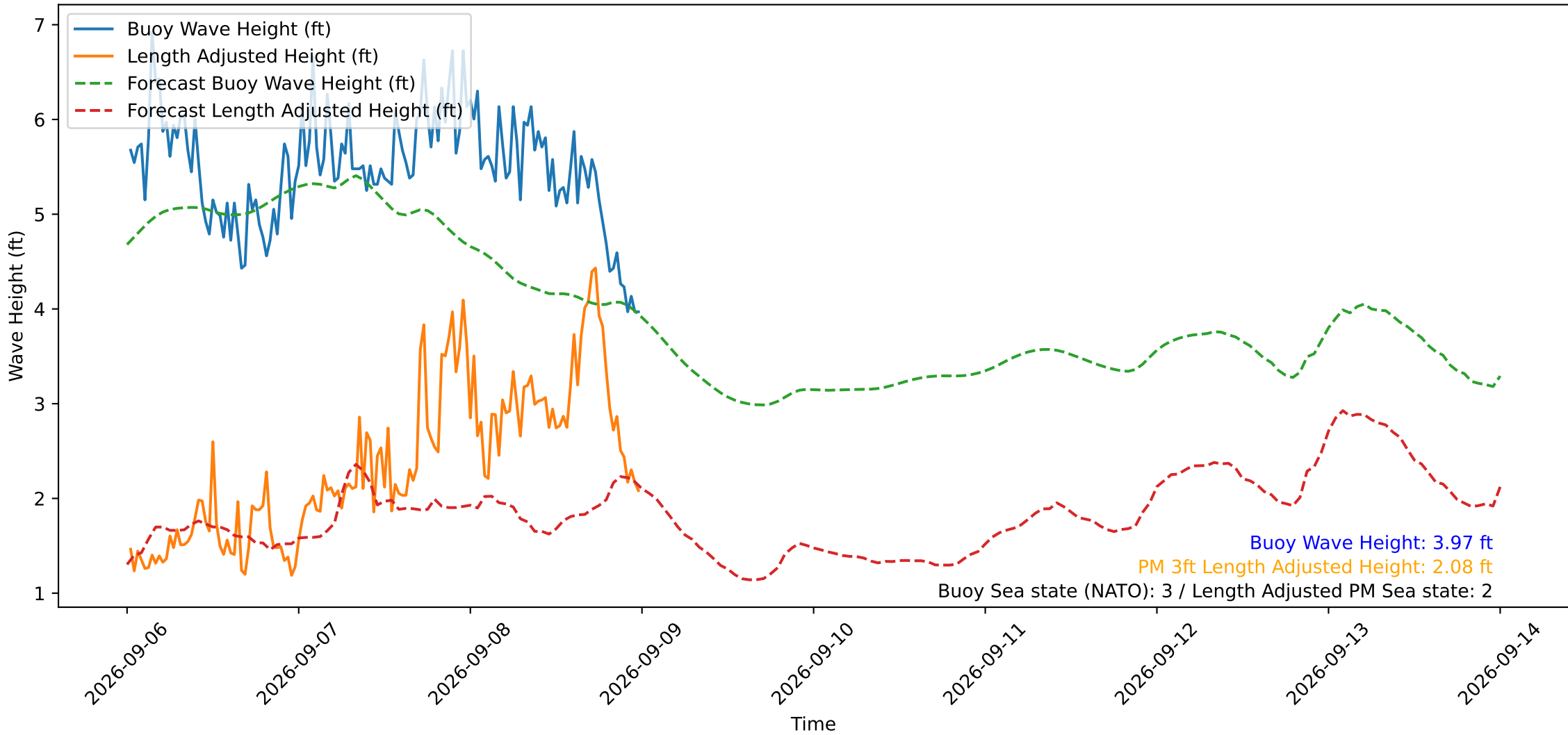
Wave Heights over Time for Red Beach at 2026-09-09 00:10:49
