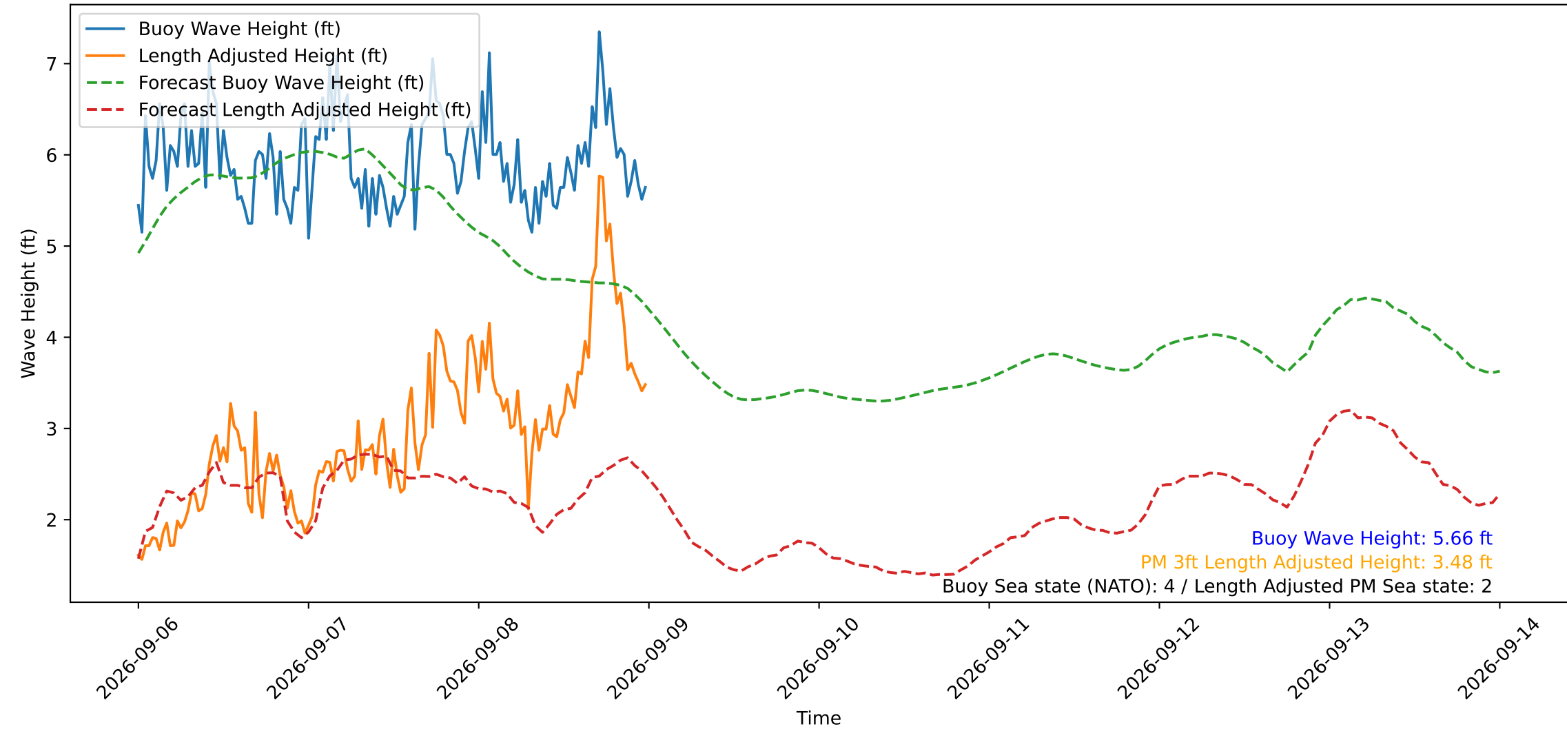
Wave Heights over Time for Oceanside Harbor at 2026-09-09 00:10:29
