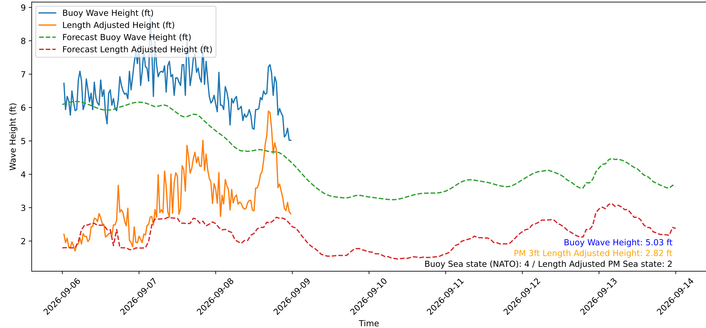
Wave Heights over Time for Green Beach at 2026-09-09 00:11:11
