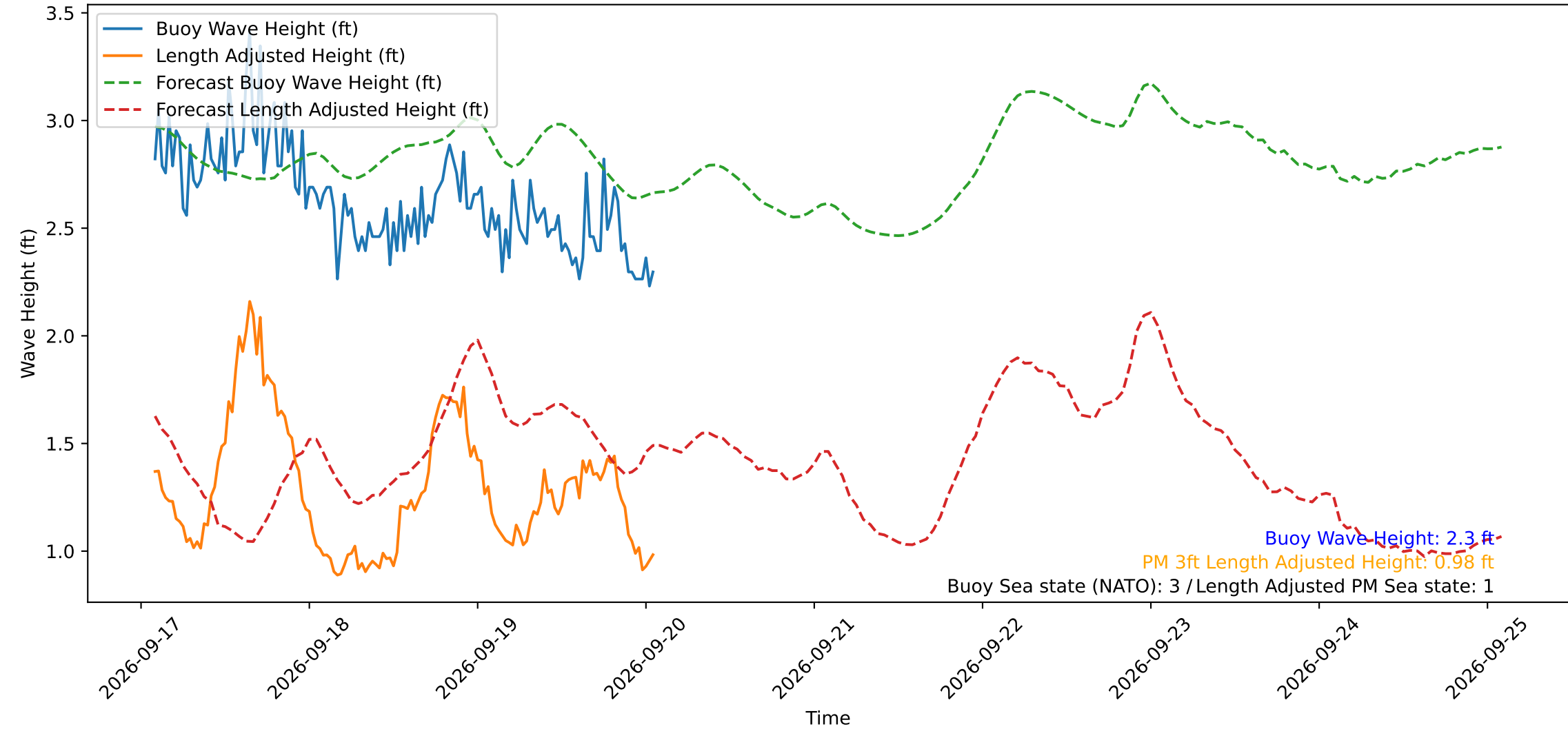
Wave Heights over Time for Red Beach at 2026-09-20 01:40:49
