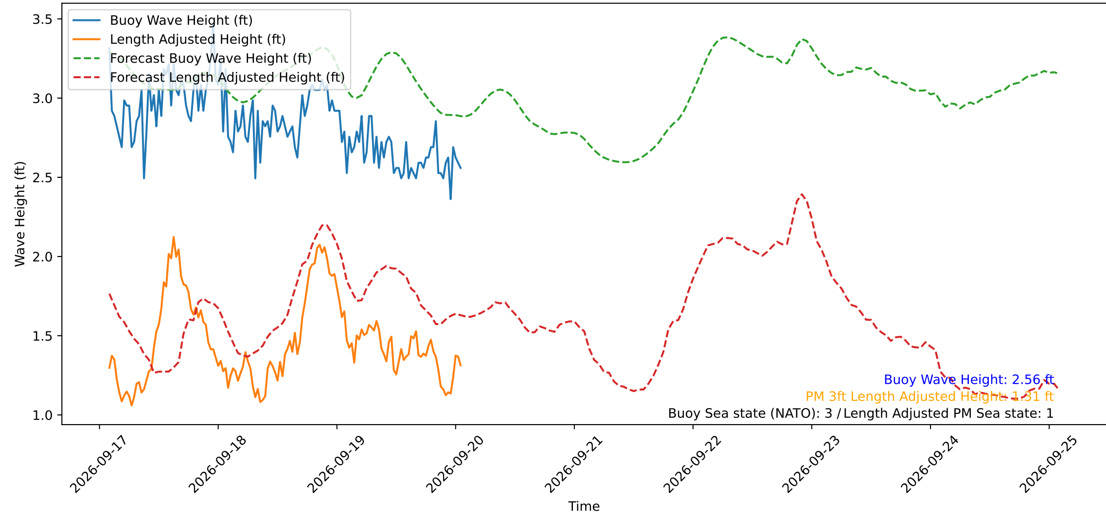
Wave Heights over Time for Green Beach at 2026-09-20 01:41:11
