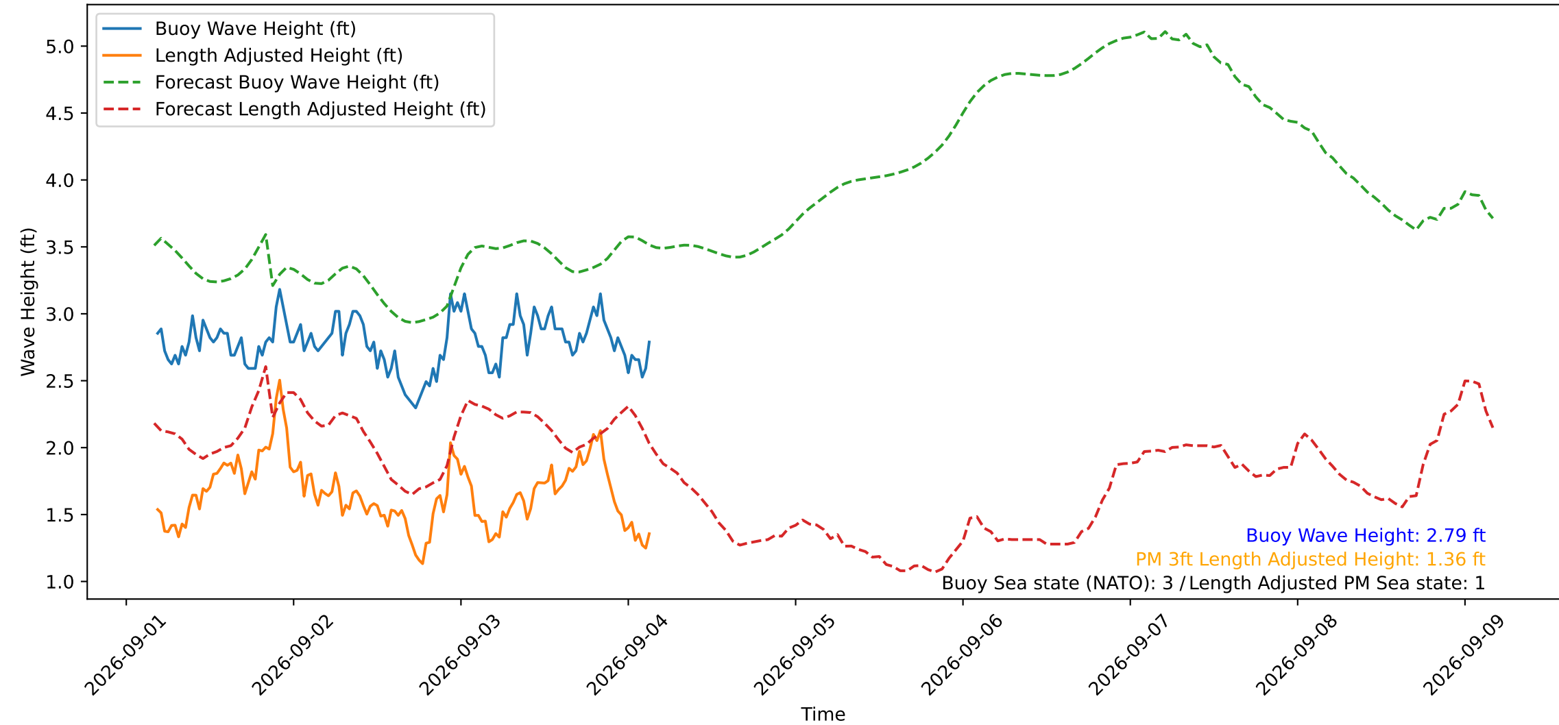
Wave Heights over Time for Red Beach at 2026-09-04 04:00:49
