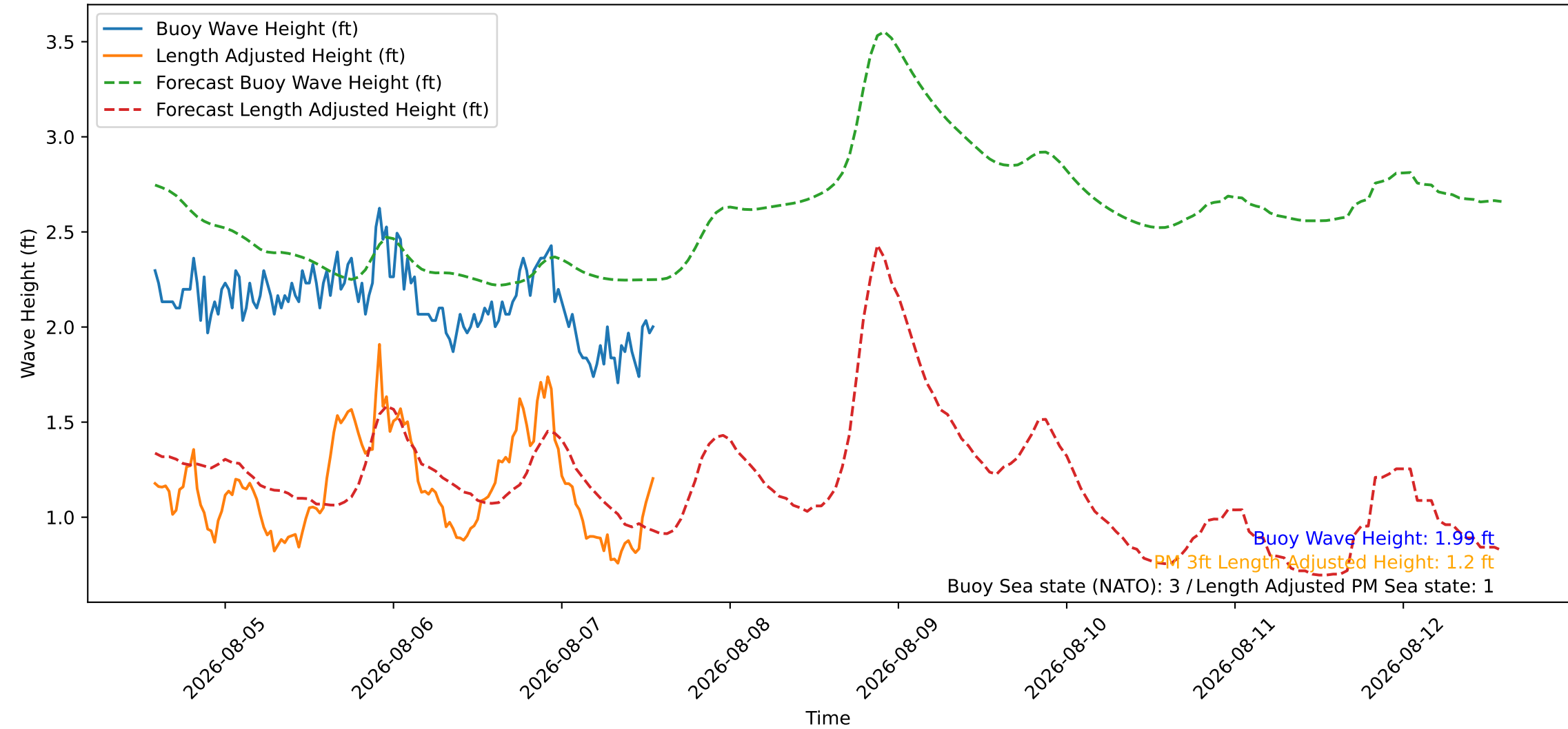
Wave Heights over Time for Green Beach at 2026-08-07 14:01:09
