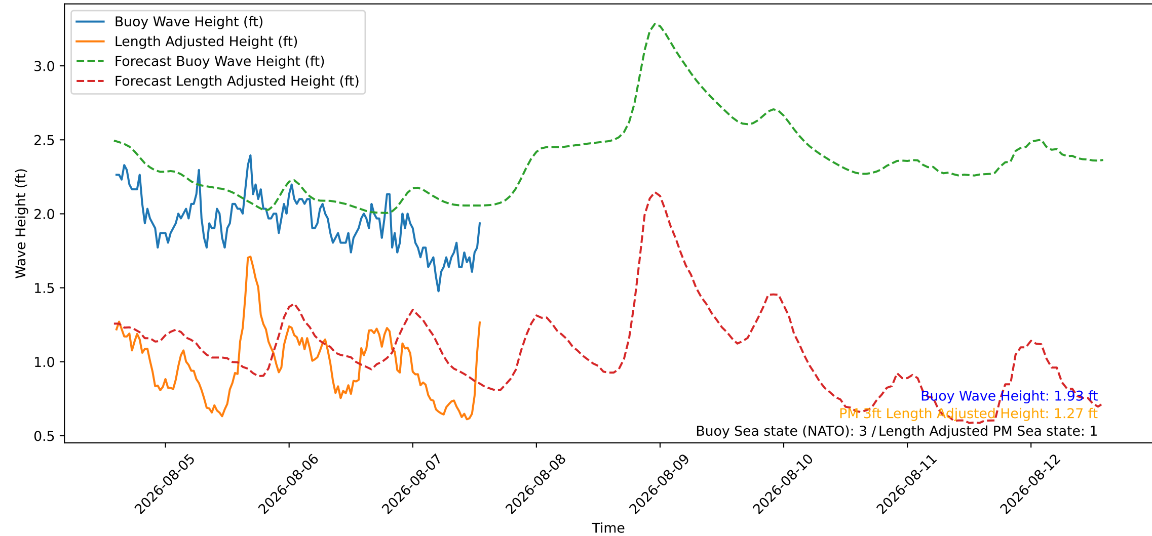
Wave Heights over Time for Red Beach at 2026-08-07 14:00:46
