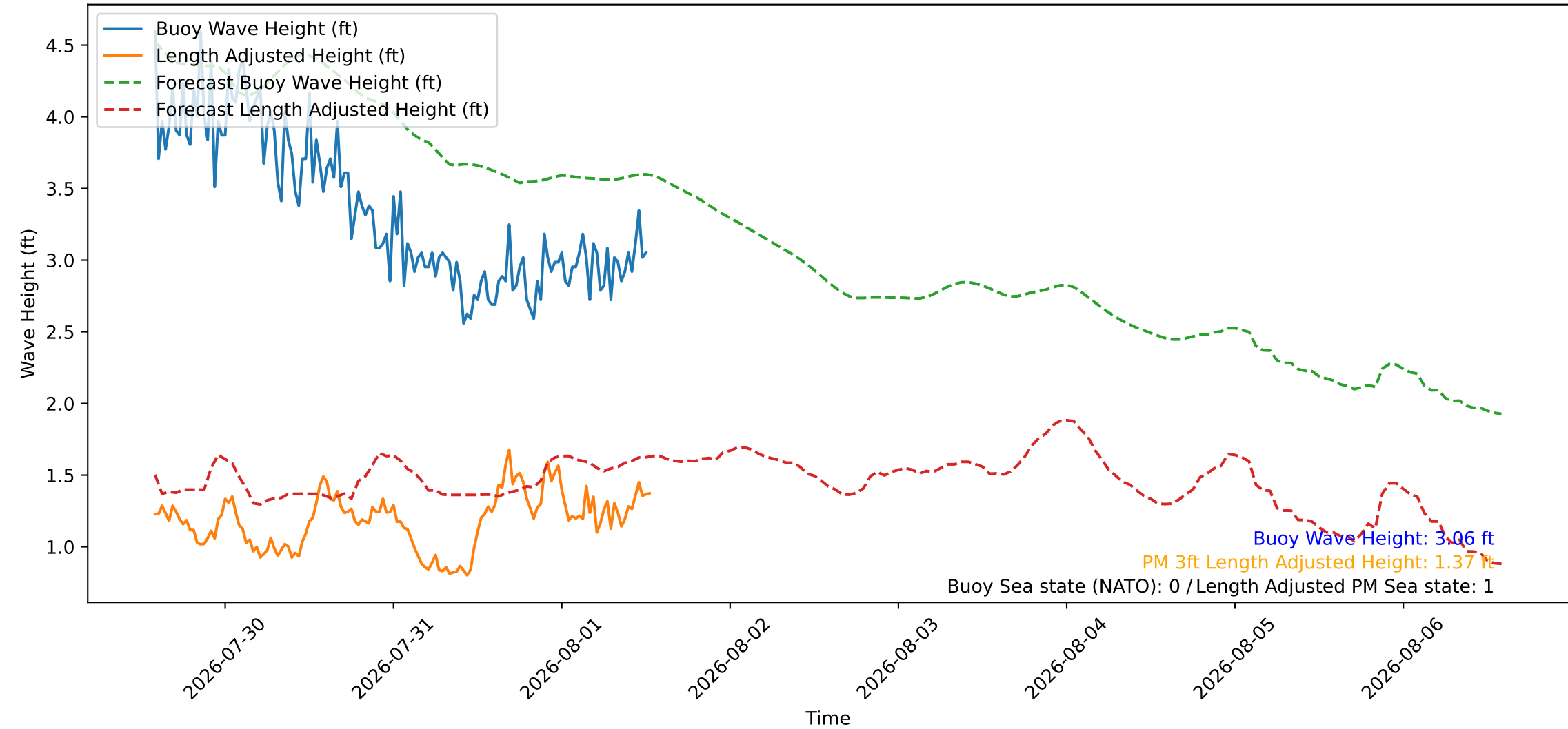
Wave Heights over Time for Red Beach at 2026-08-01 13:30:46
