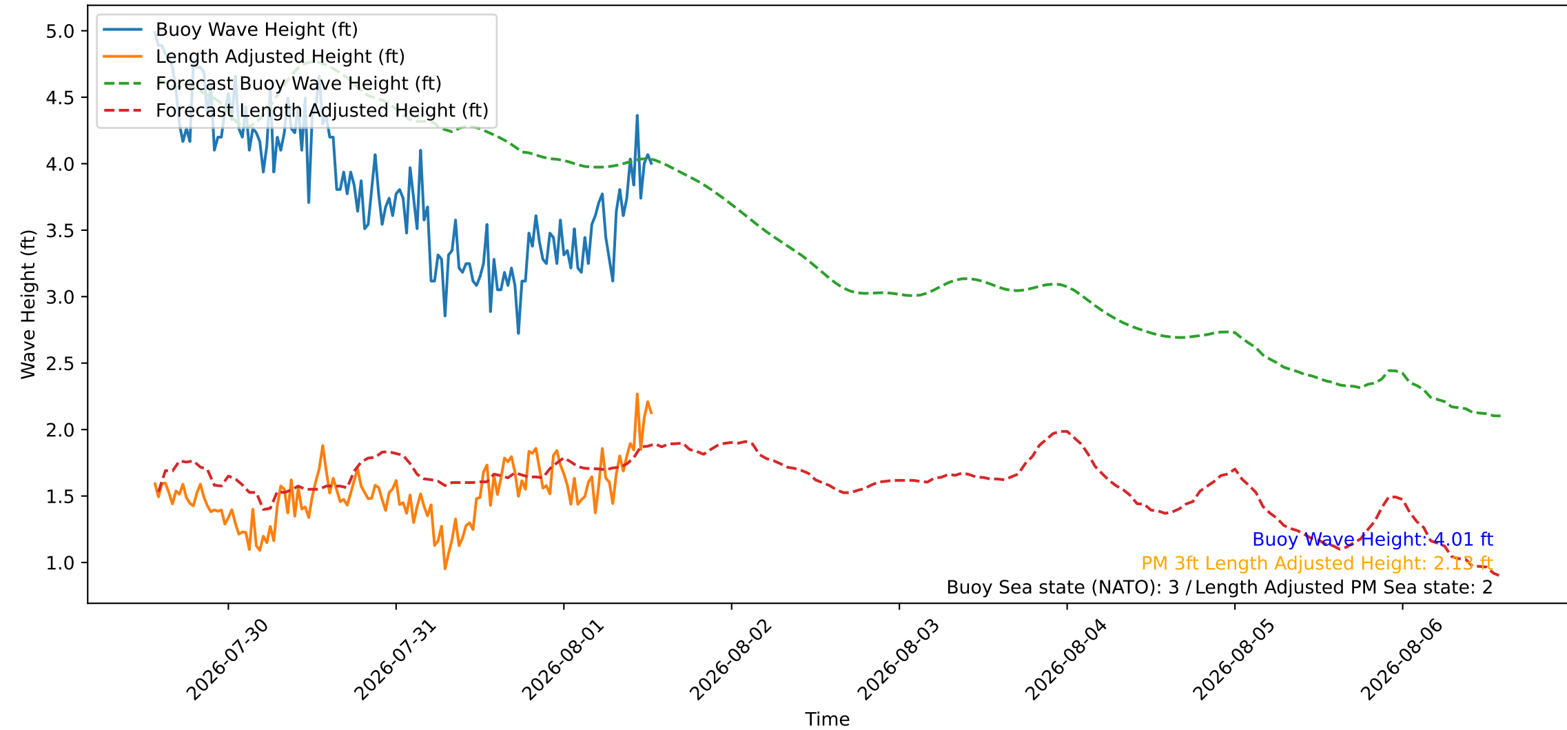
Wave Heights over Time for Oceanside Harbor at 2026-08-01 13:30:26
