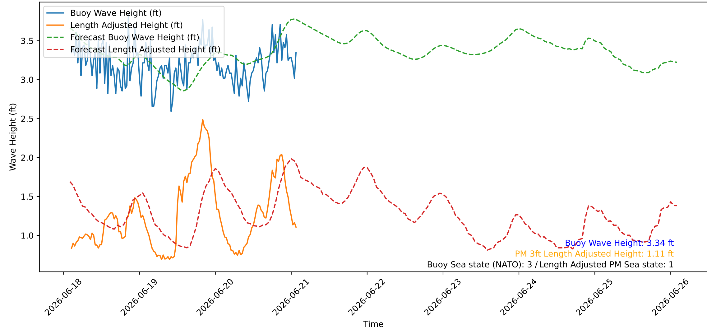
Wave Heights over Time for Red Beach at 2026-06-21 02:10:45
