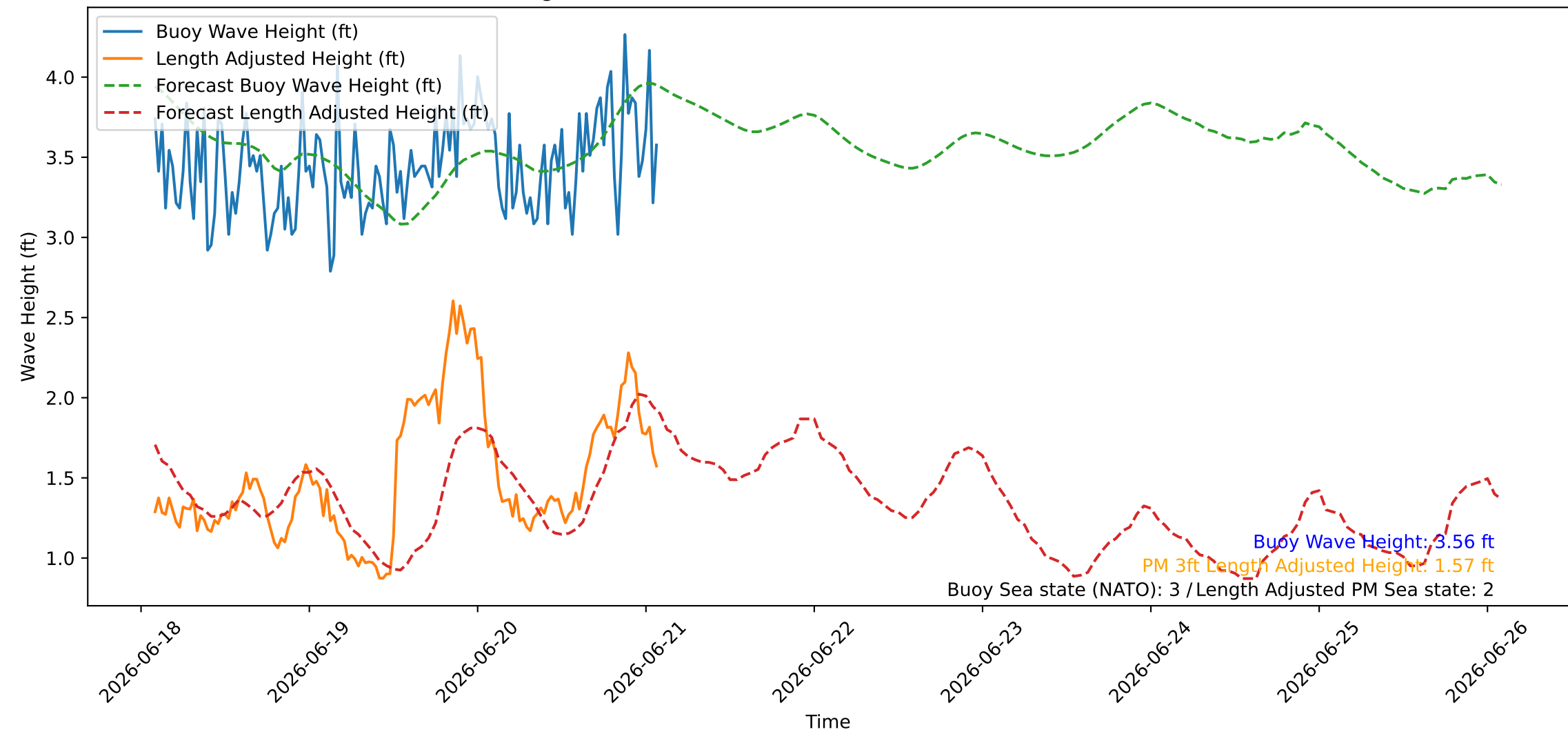
Wave Heights over Time for Oceanside Harbor at 2026-06-21 02:10:26
