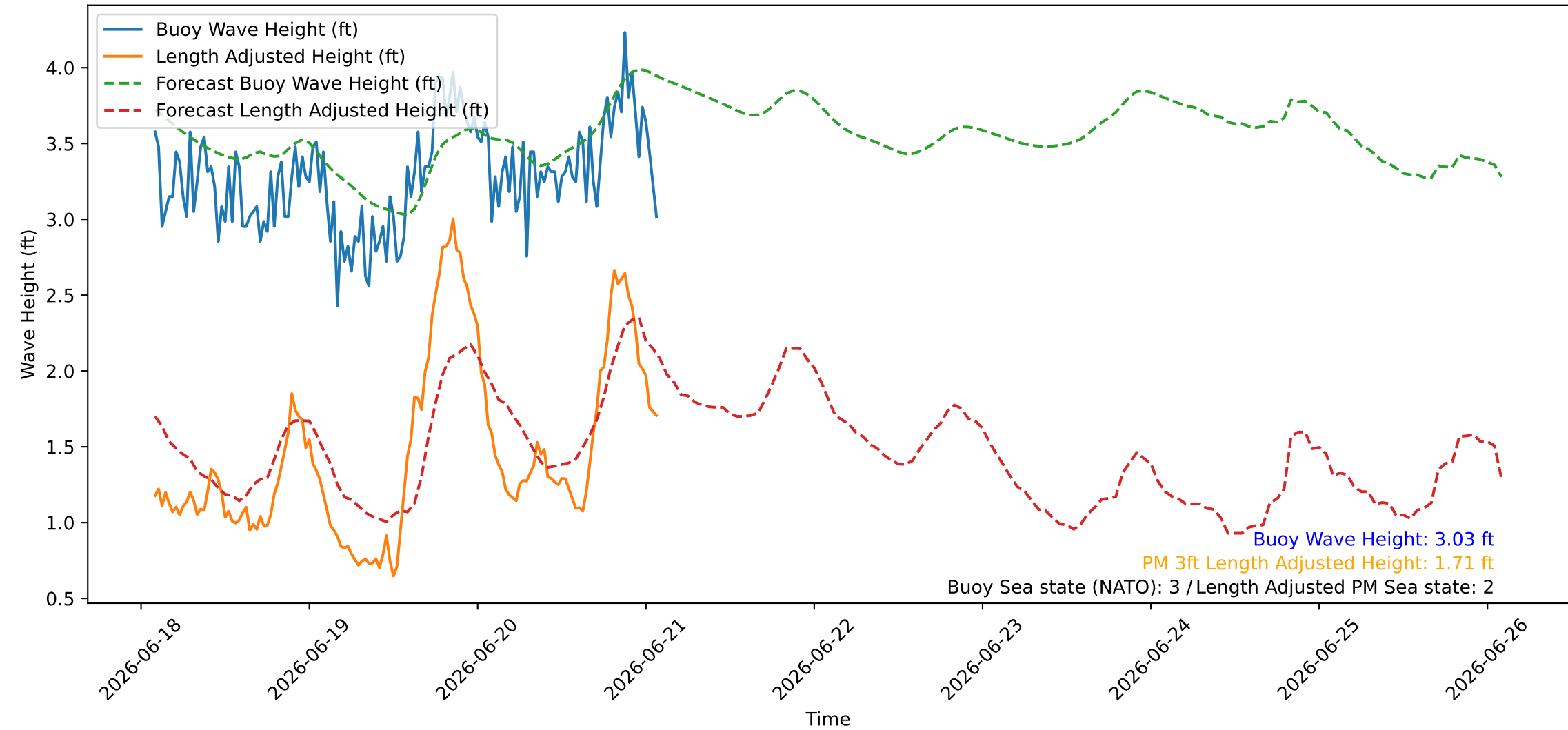
Wave Heights over Time for Green Beach at 2026-06-21 02:11:07
