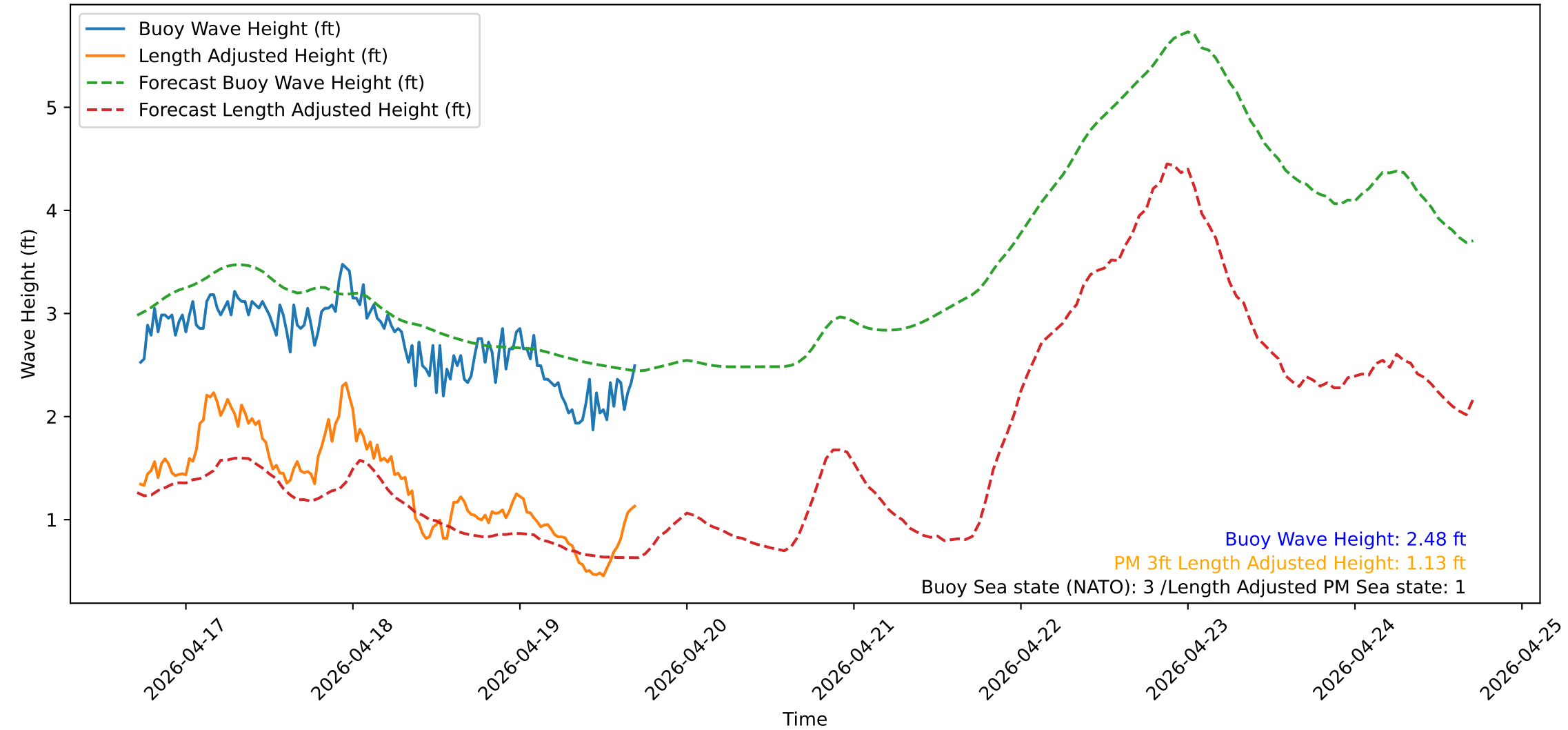
Wave Heights over Time for Green Beach at 2026-04-19 17:21:15
