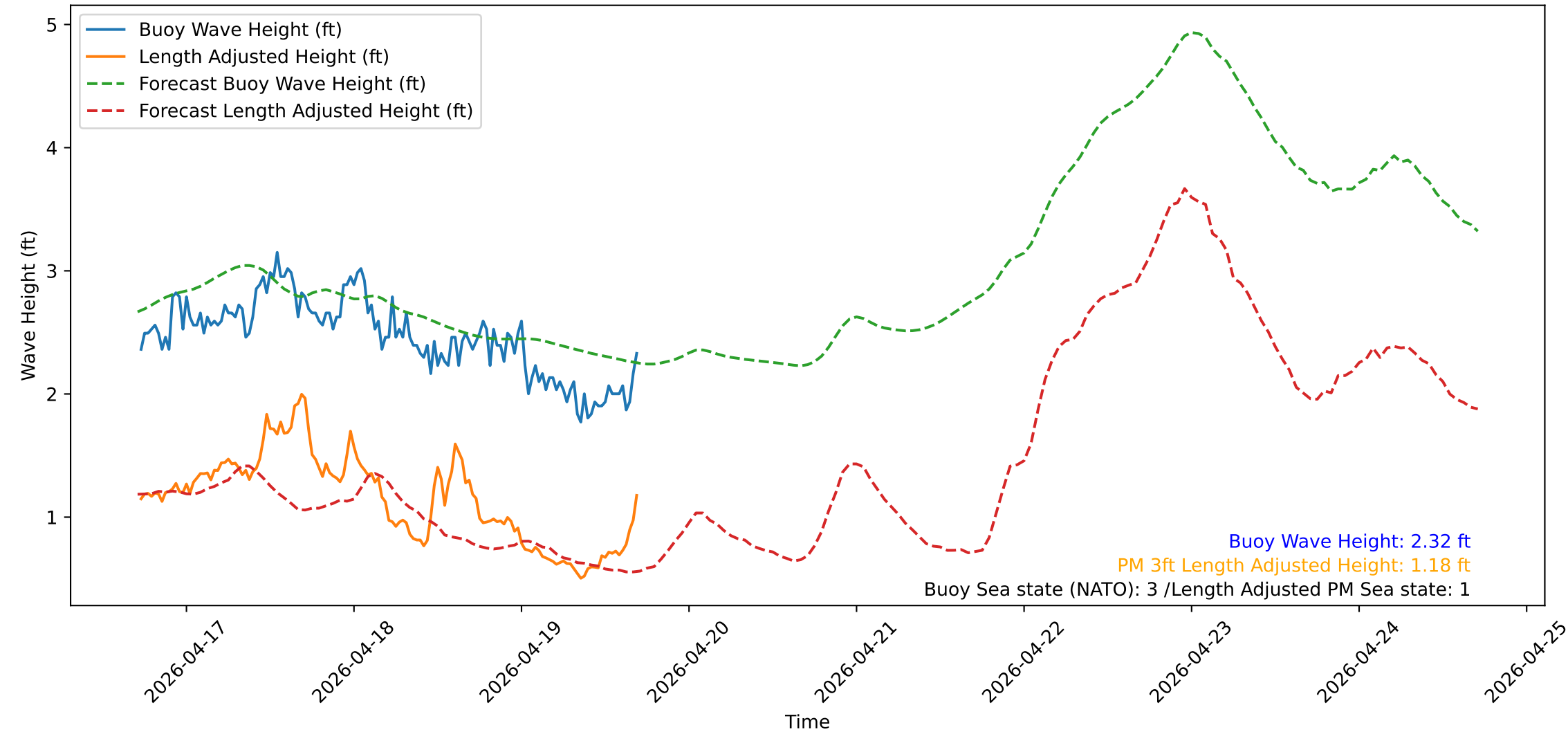
Wave Heights over Time for Red Beach at 2026-04-19 17:20:52
