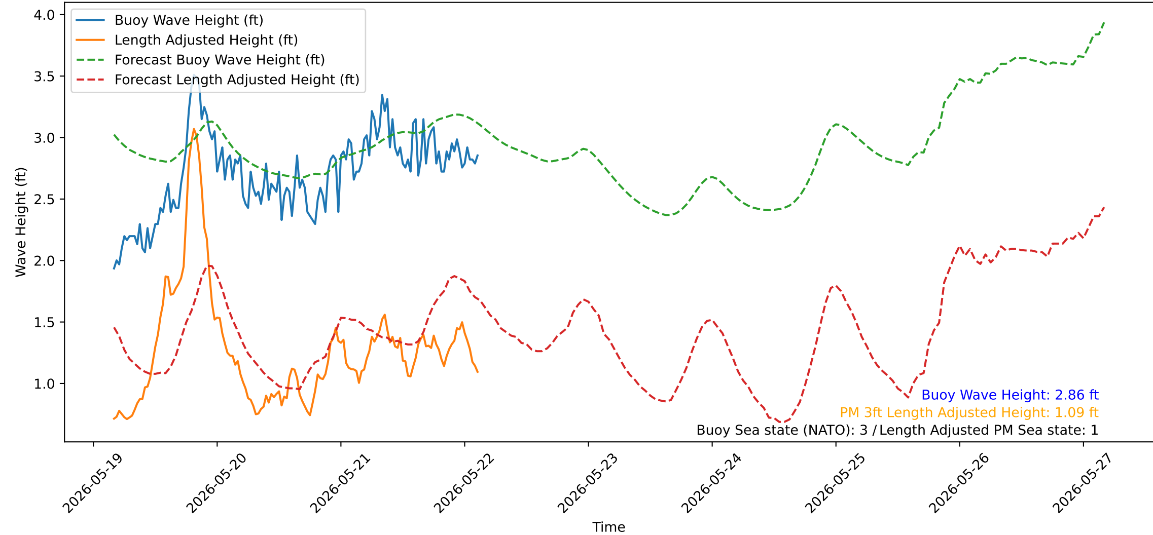
Wave Heights over Time for Red Beach at 2026-05-22 03:30:51
