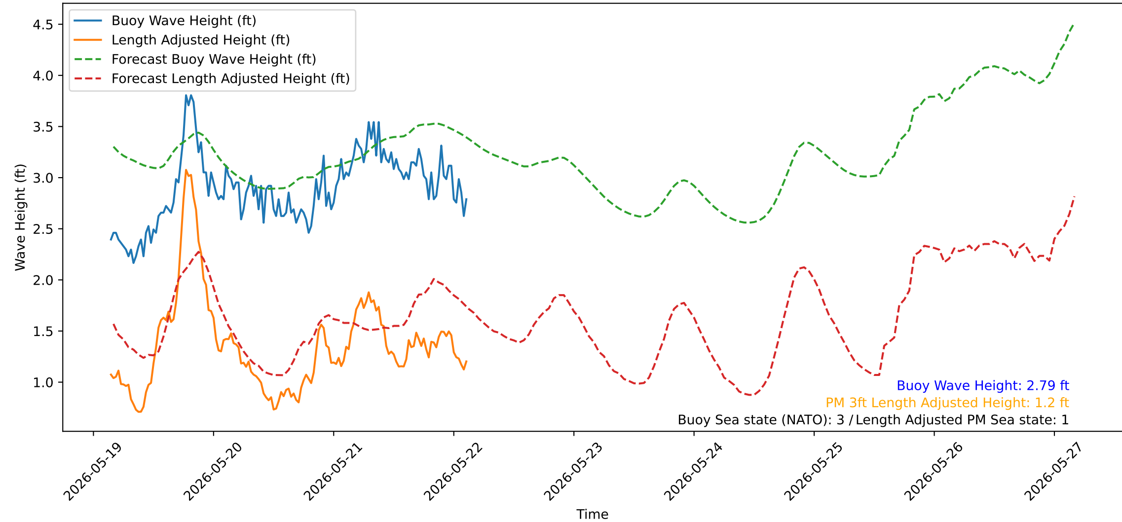
Wave Heights over Time for Green Beach at 2026-05-22 03:31:14
