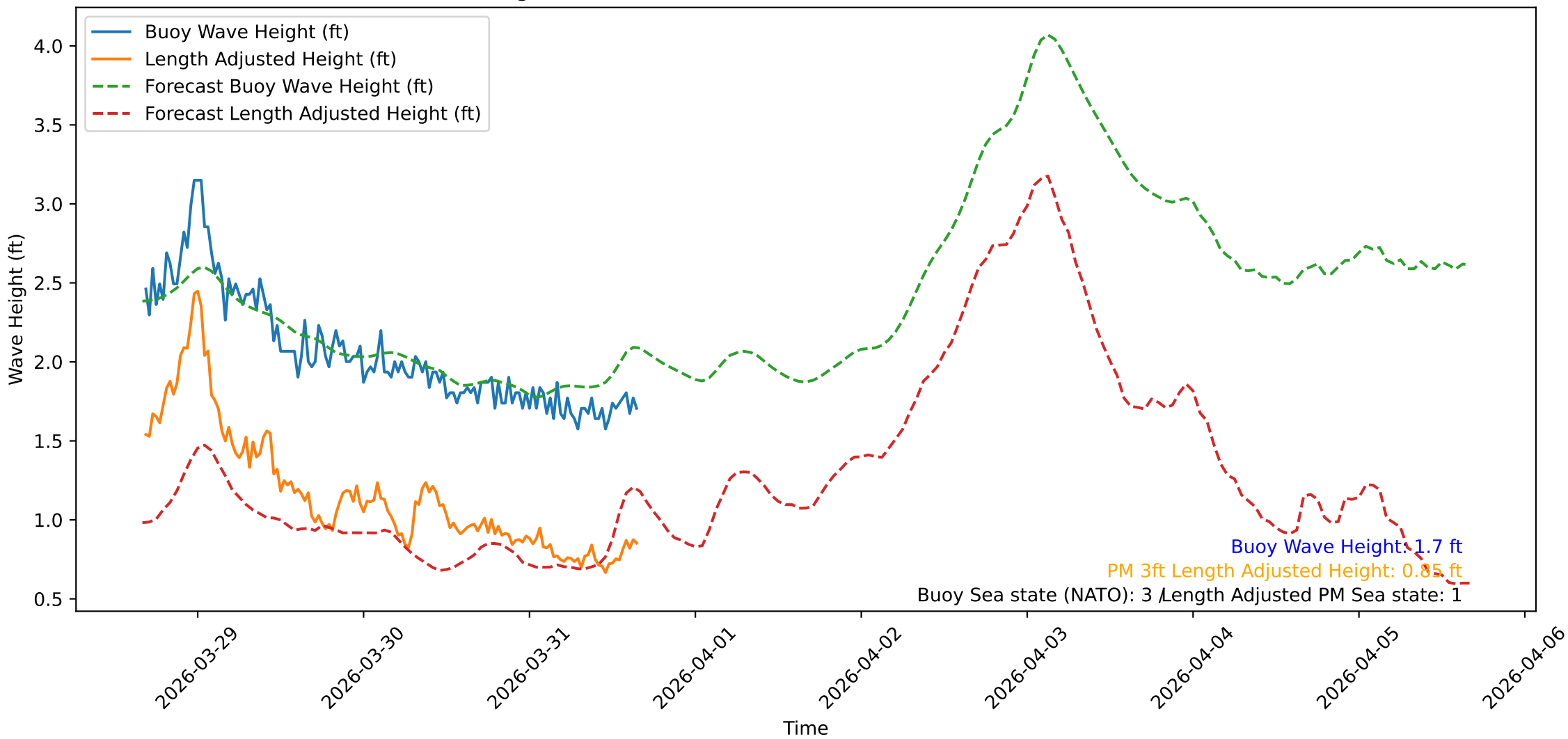
Wave Heights over Time for Oceanside Harbor at 2026-03-31 16:20:32
