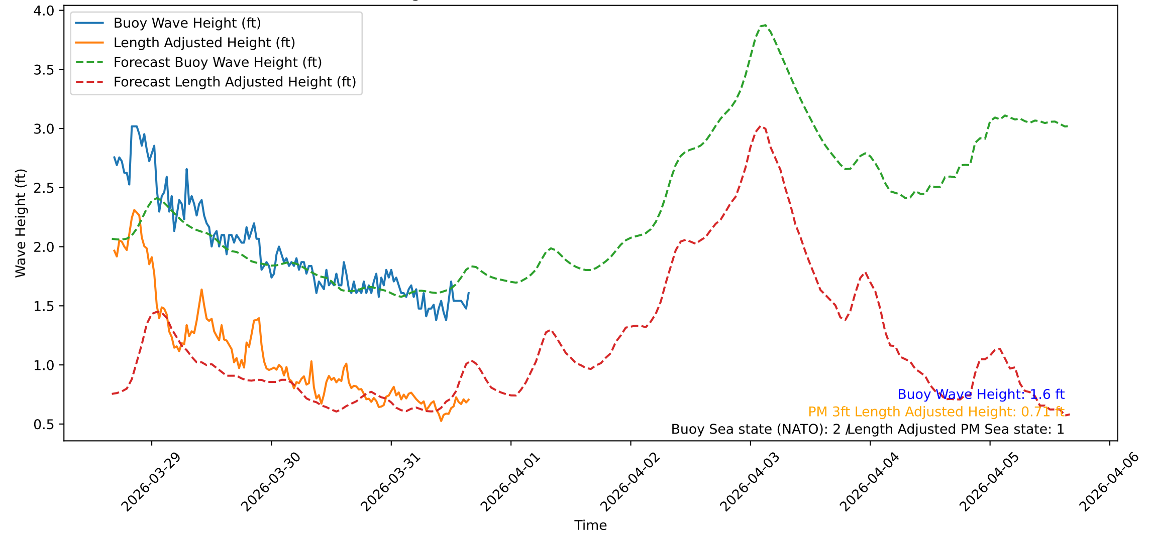
Wave Heights over Time for Red Beach at 2026-03-31 16:20:48
