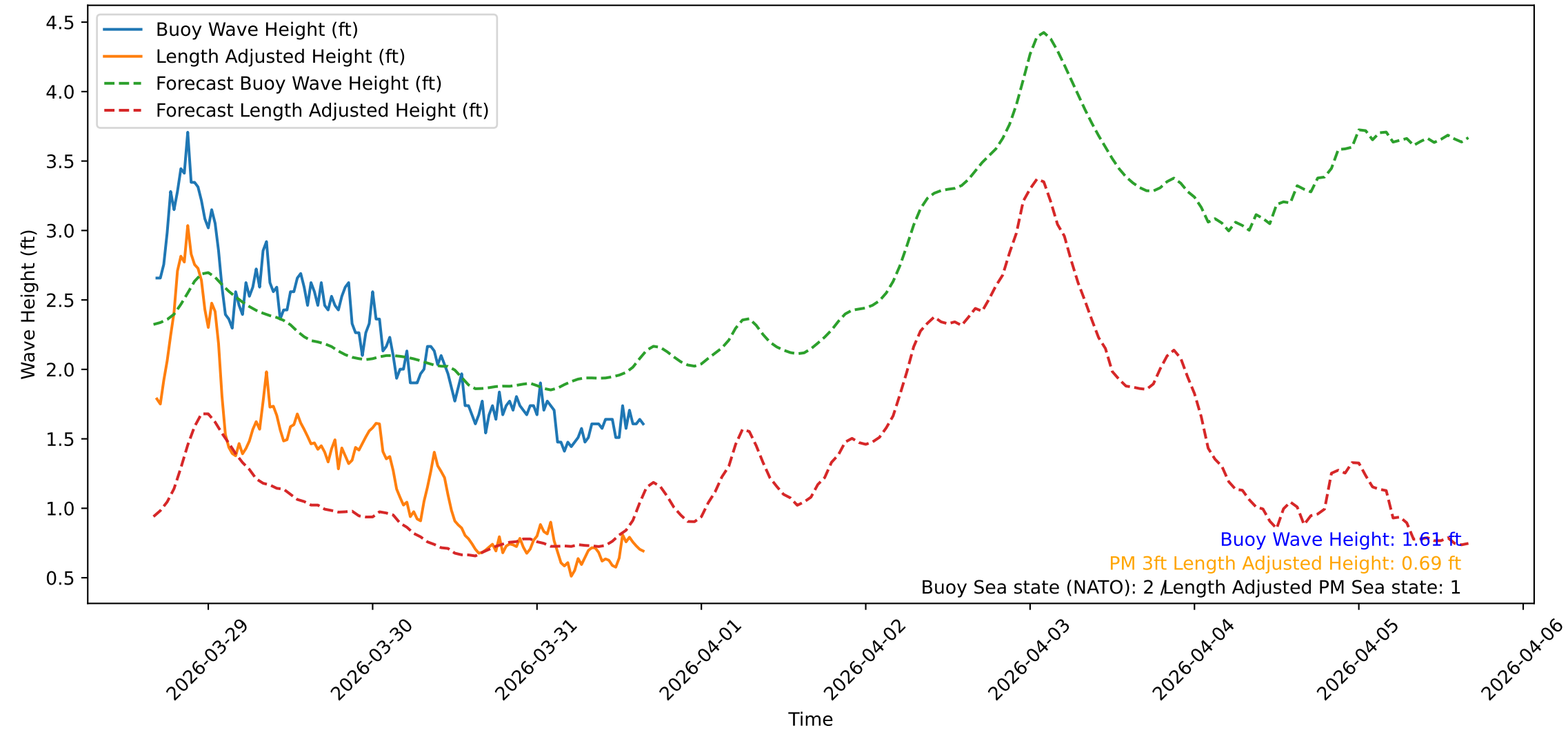
Wave Heights over Time for Green Beach at 2026-03-31 16:21:11
