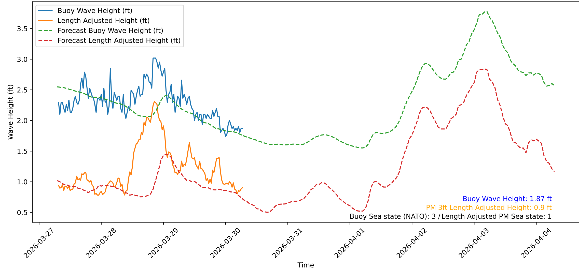
Wave Heights over Time for Red Beach at 2026-03-30 07:20:47
