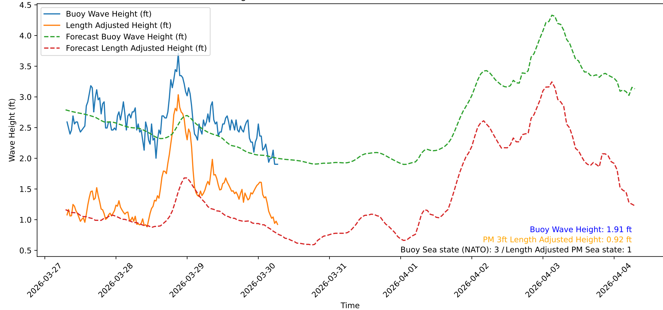
Wave Heights over Time for Green Beach at 2026-03-30 07:21:09
