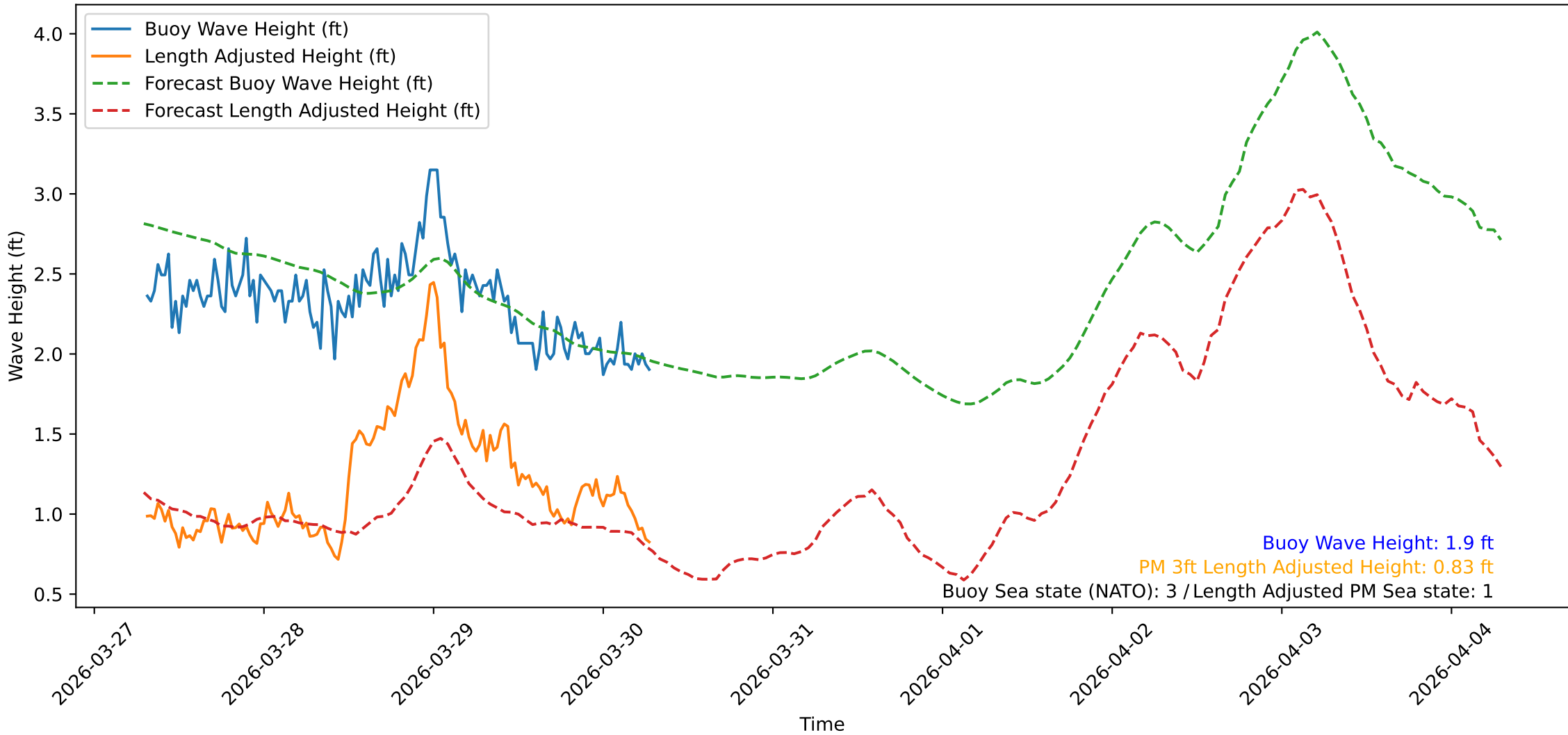
Wave Heights over Time for Oceanside Harbor at 2026-03-30 07:20:31
