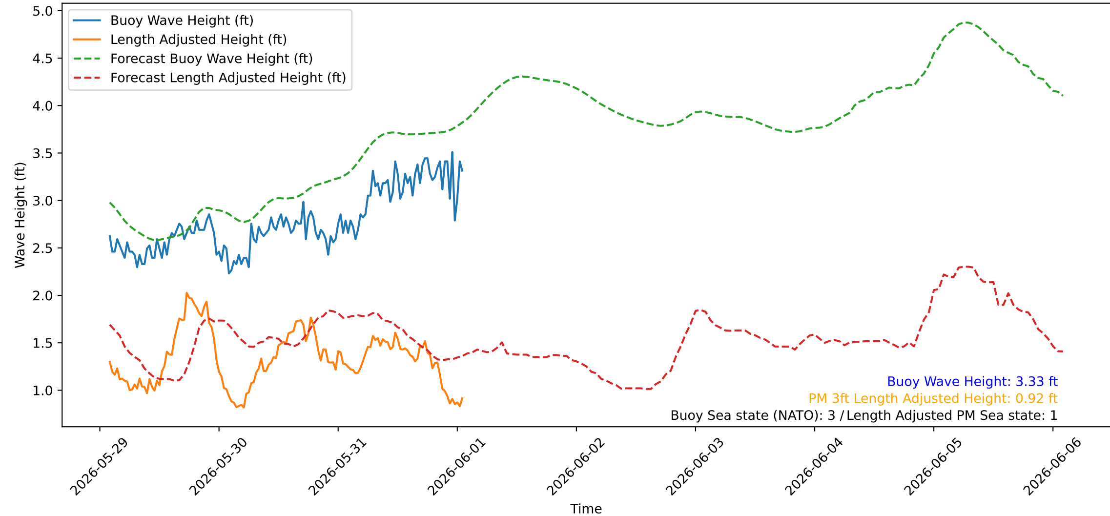
Wave Heights over Time for Red Beach at 2026-06-01 01:40:46
