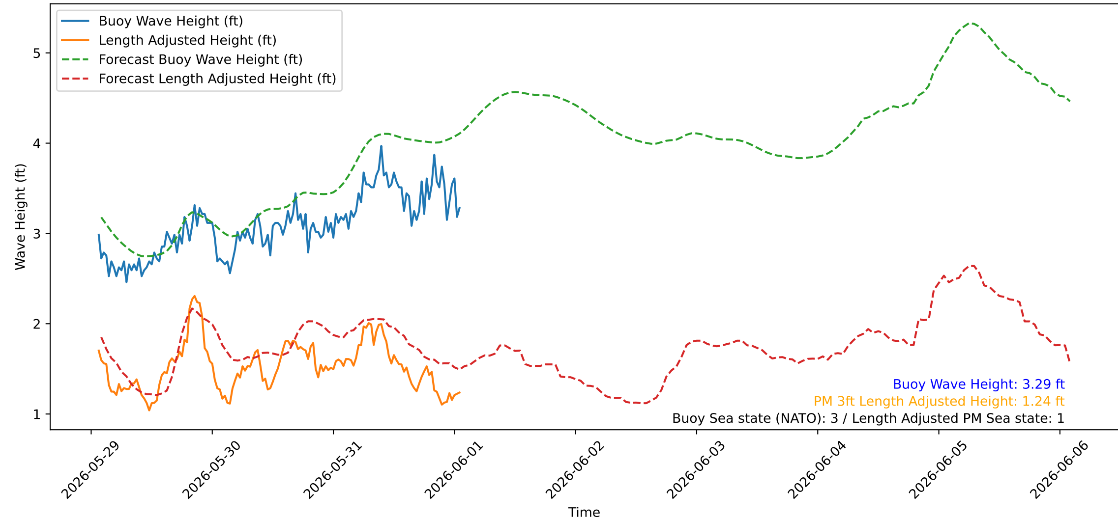
Wave Heights over Time for Green Beach at 2026-06-01 01:41:09
