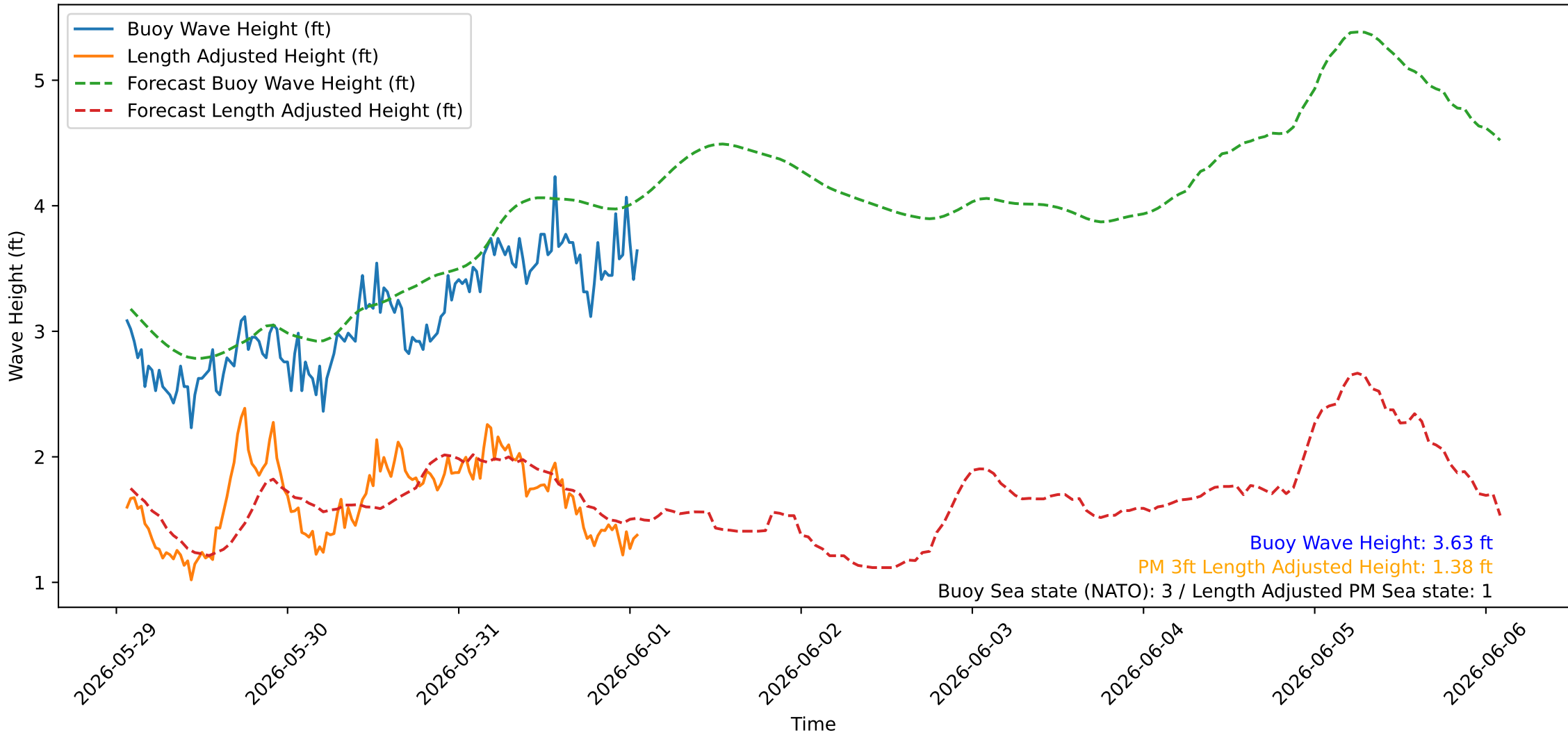
Wave Heights over Time for Oceanside Harbor at 2026-06-01 01:40:26
