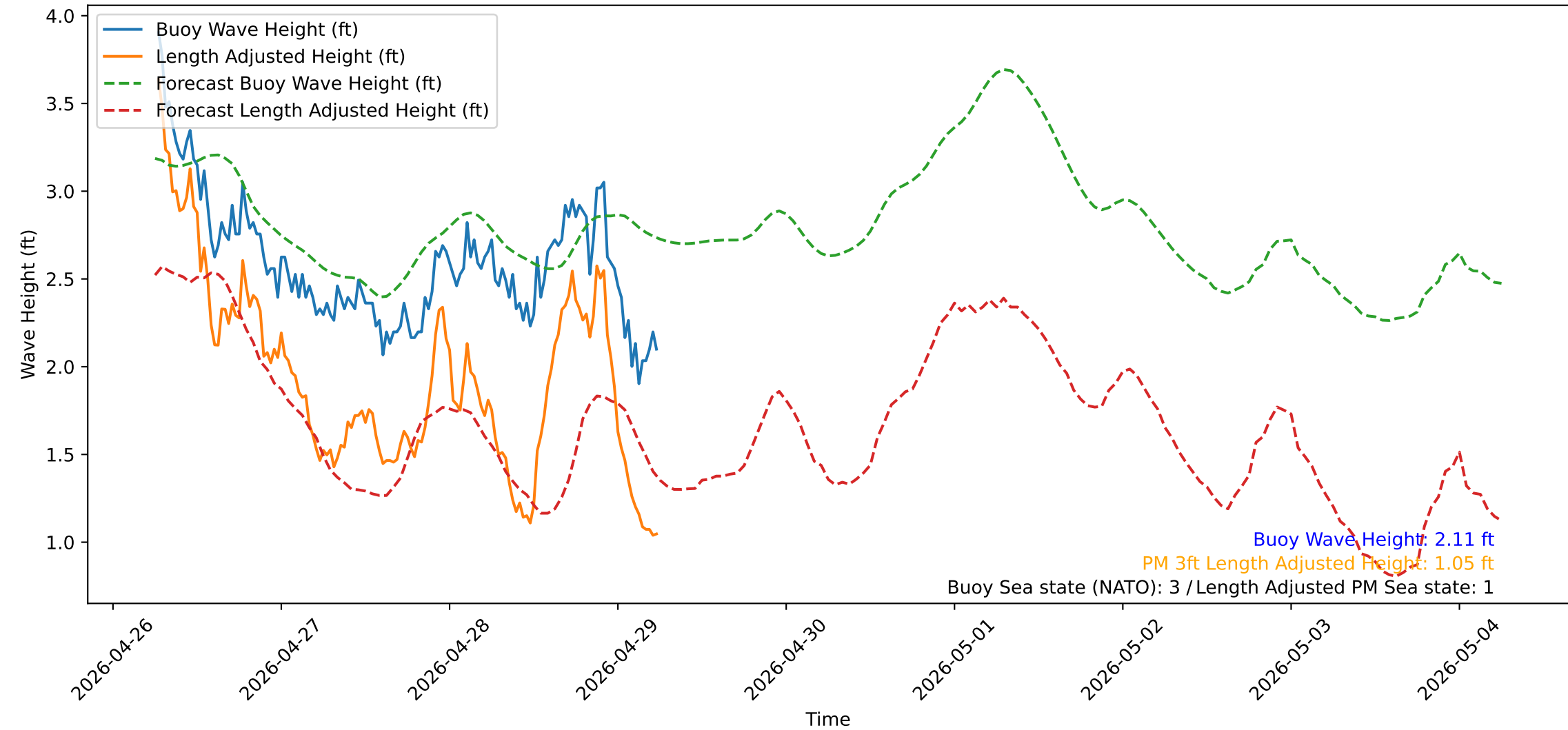
Wave Heights over Time for Oceanside Harbor at 2026-04-29 06:20:31
