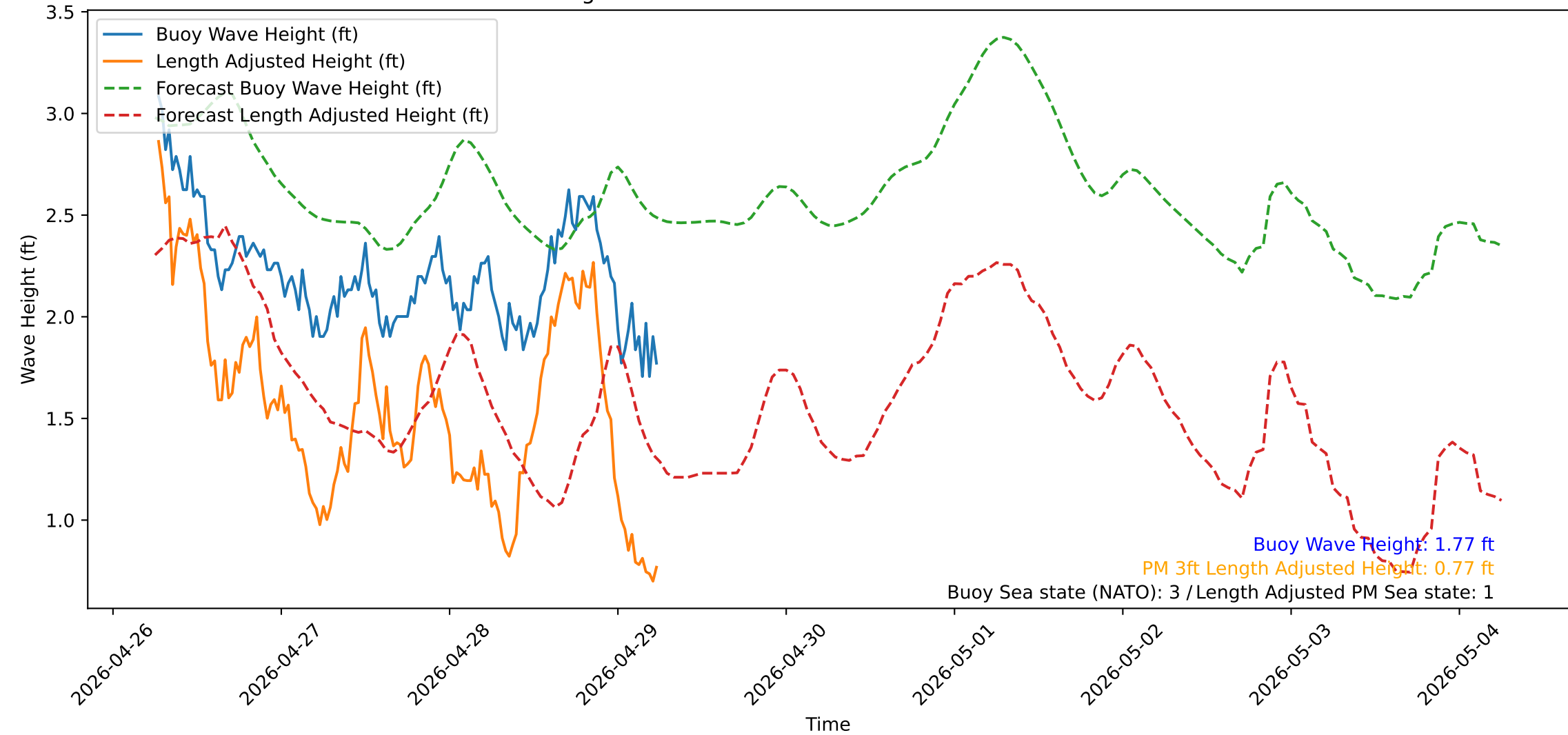
Wave Heights over Time for Red Beach at 2026-04-29 06:20:52
