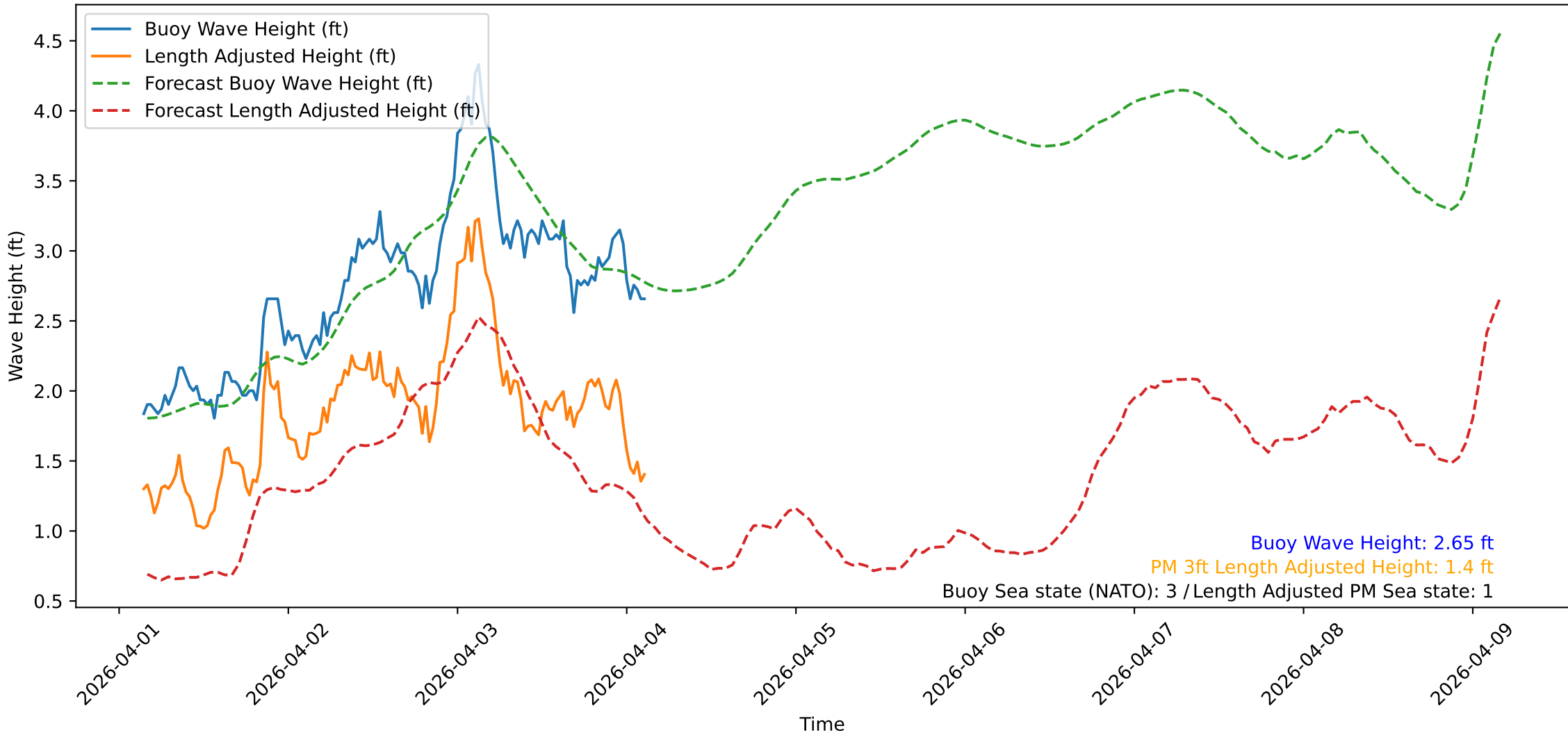
Wave Heights over Time for Green Beach at 2026-04-04 03:31:10
