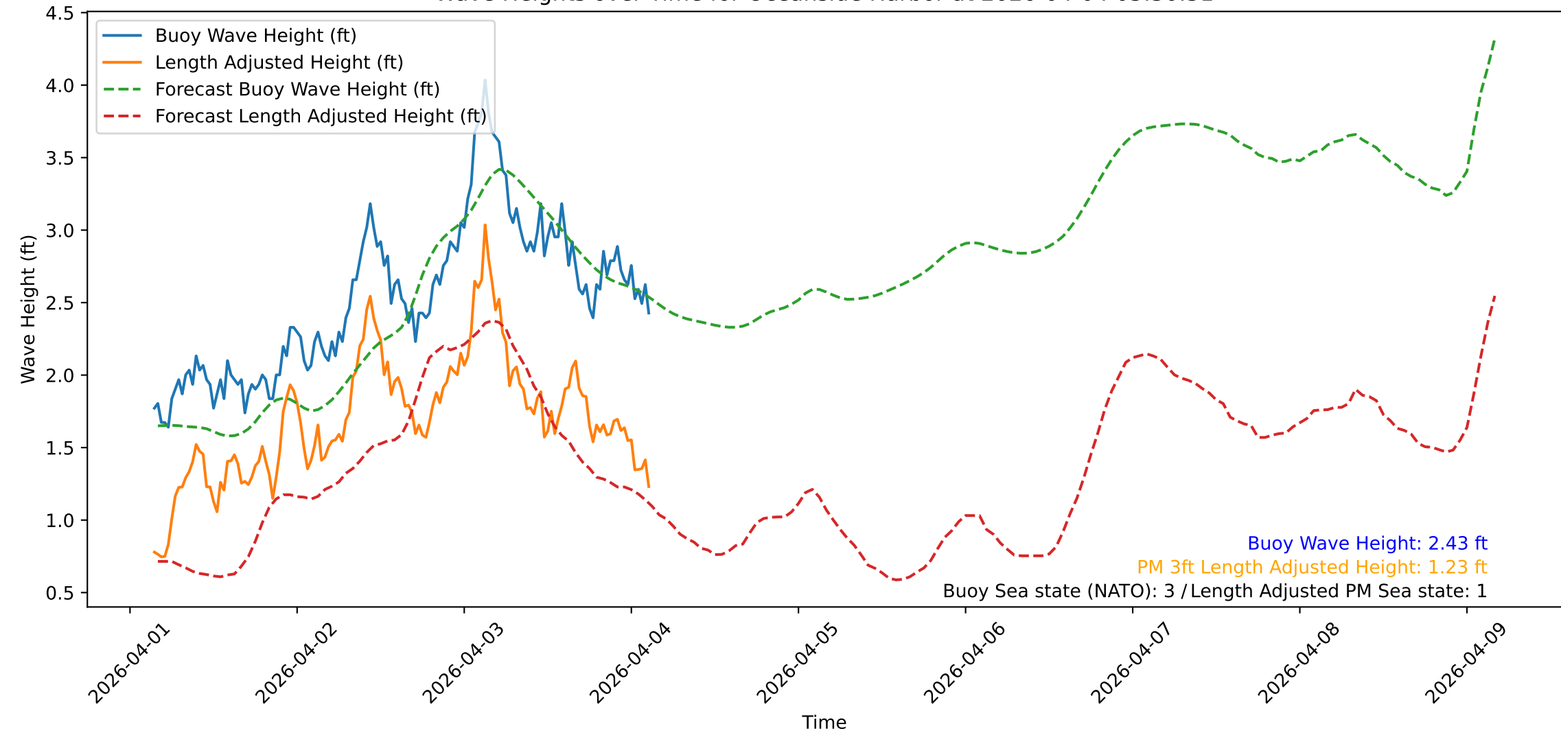
Wave Heights over Time for Oceanside Harbor at 2026-04-04 03:30:31
