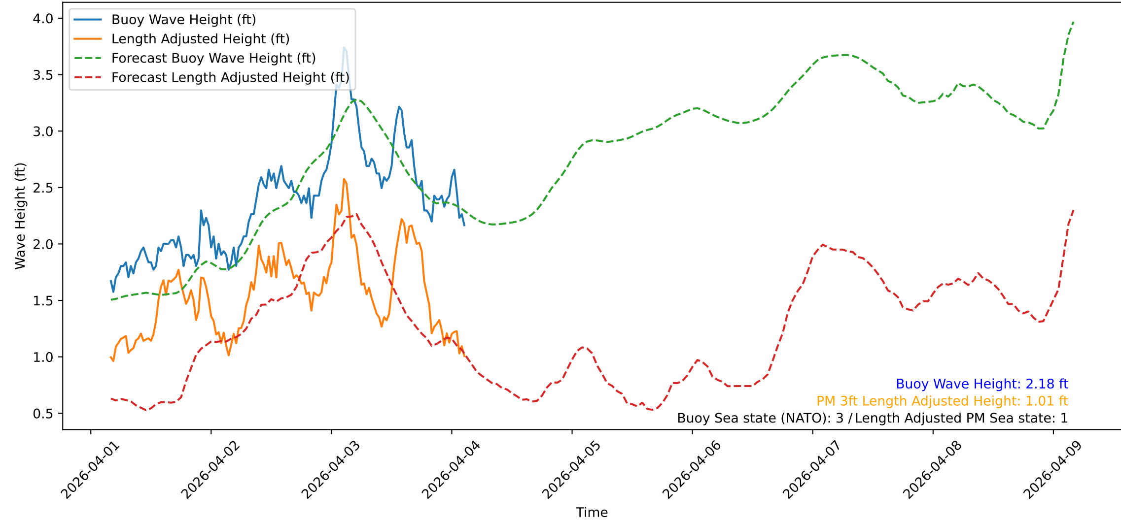
Wave Heights over Time for Red Beach at 2026-04-04 03:30:47
