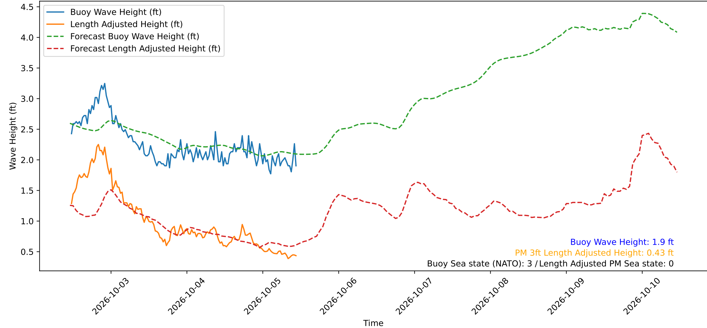
Wave Heights over Time for Red Beach at 2026-10-05 11:20:51
