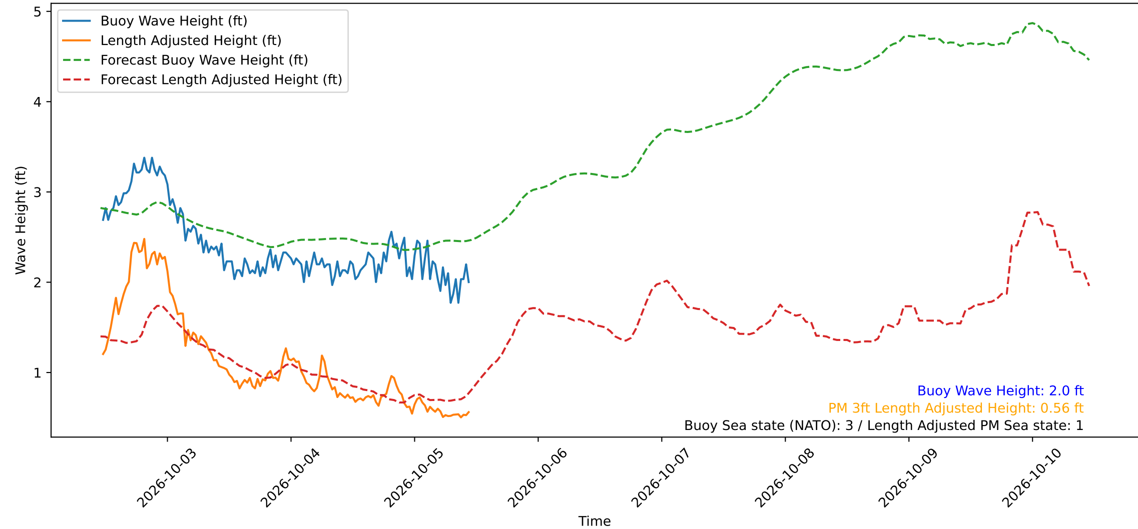
Wave Heights over Time for Green Beach at 2026-10-05 11:21:15
