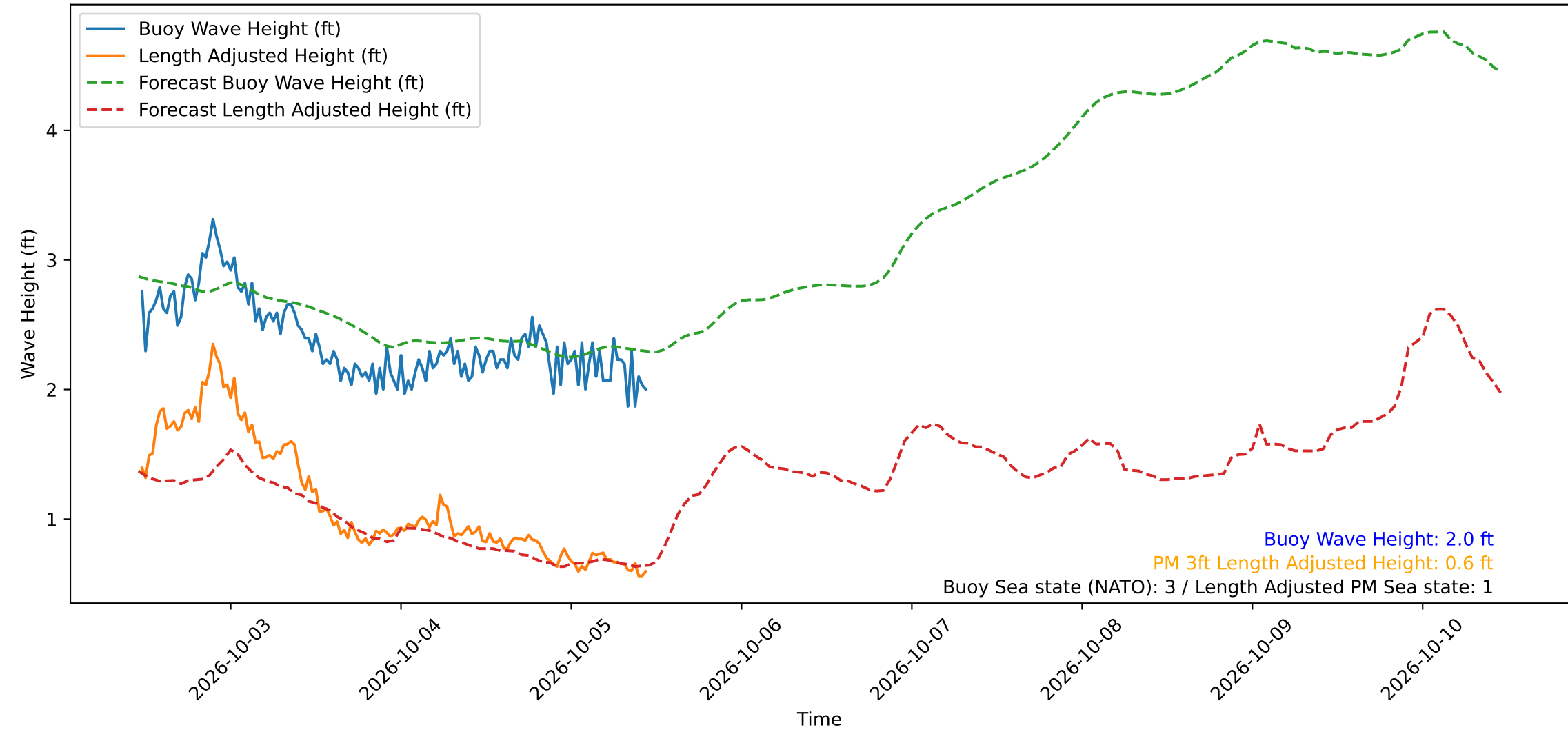
Wave Heights over Time for Oceanside Harbor at 2026-10-05 11:20:30
