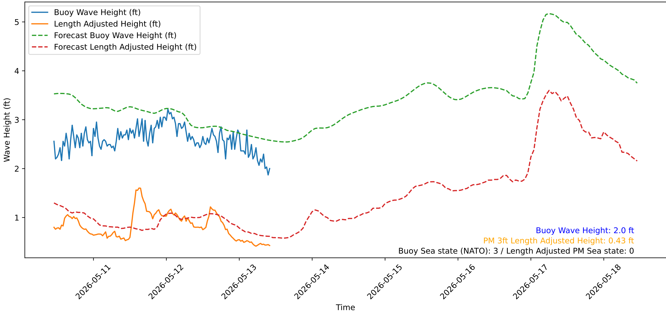
Wave Heights over Time for Red Beach at 2026-05-13 10:50:52
