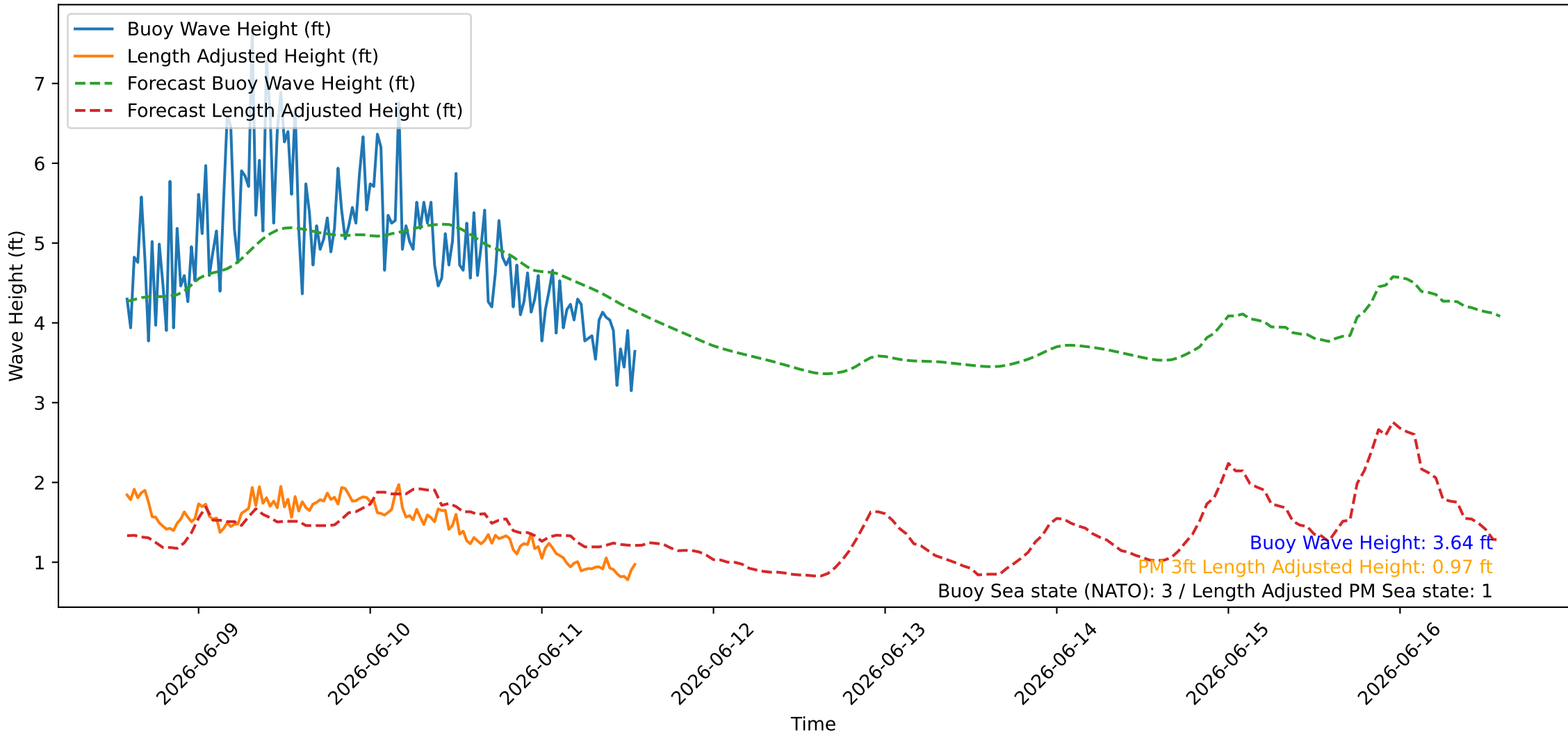
Wave Heights over Time for Red Beach at 2026-06-11 13:50:47
