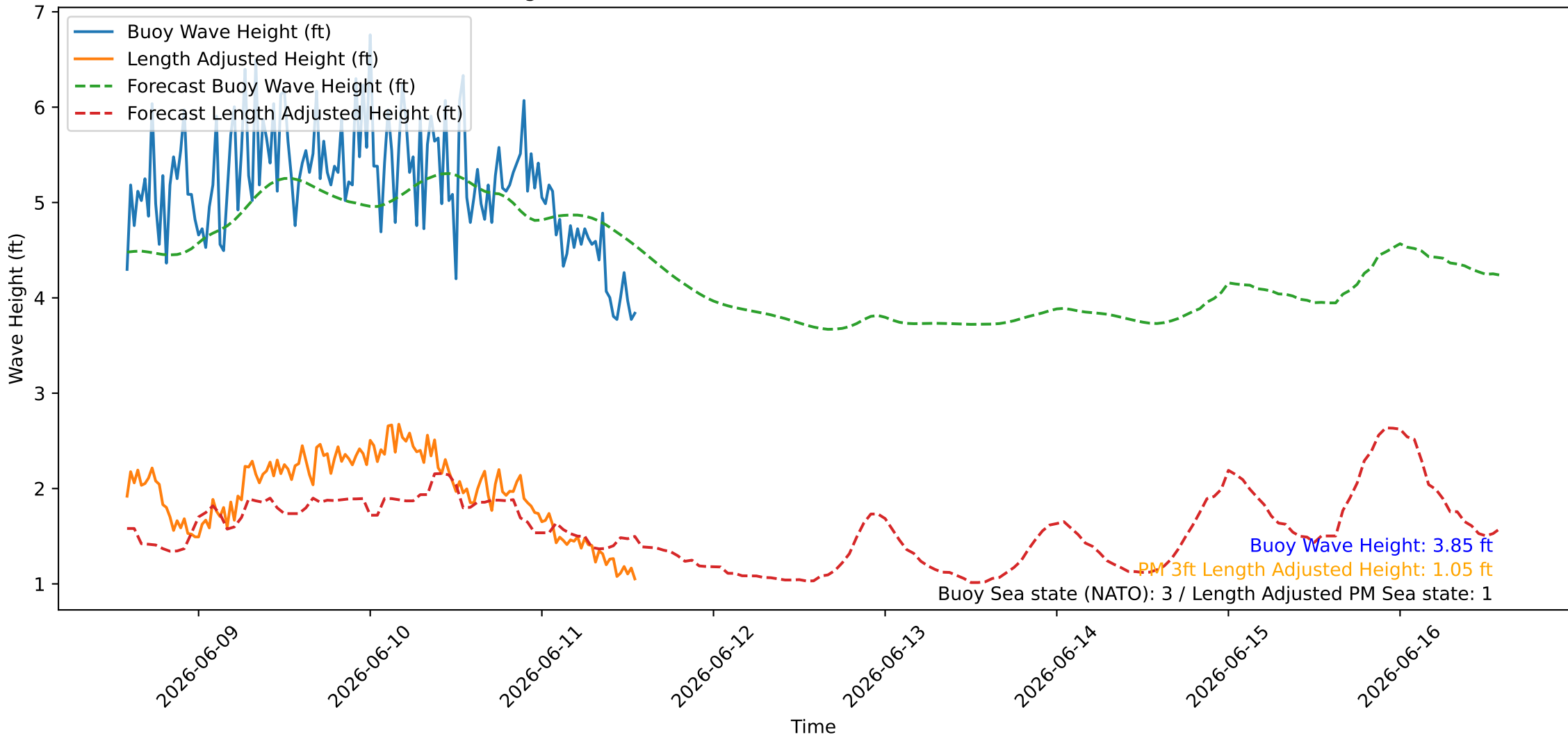
Wave Heights over Time for Oceanside Harbor at 2026-06-11 13:50:26
