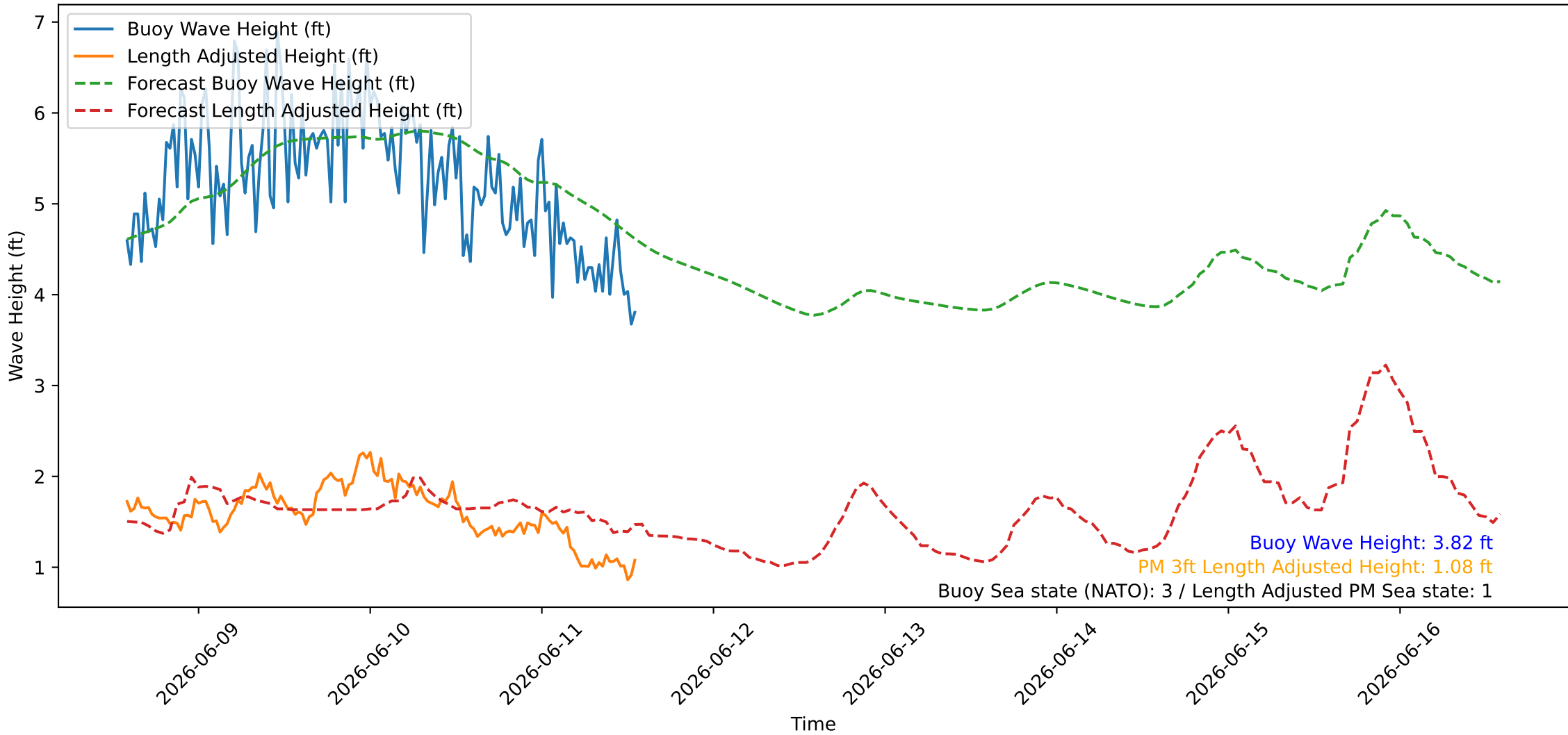
Wave Heights over Time for Green Beach at 2026-06-11 13:51:09
