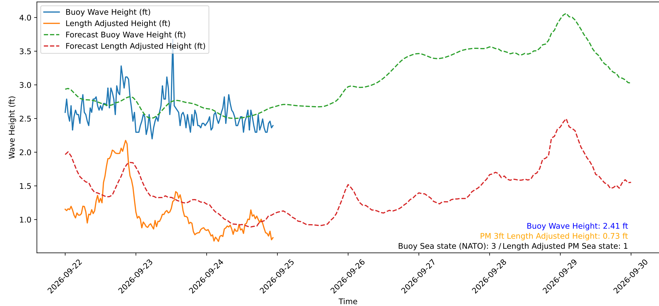
Wave Heights over Time for Red Beach at 2026-09-24 23:30:50
