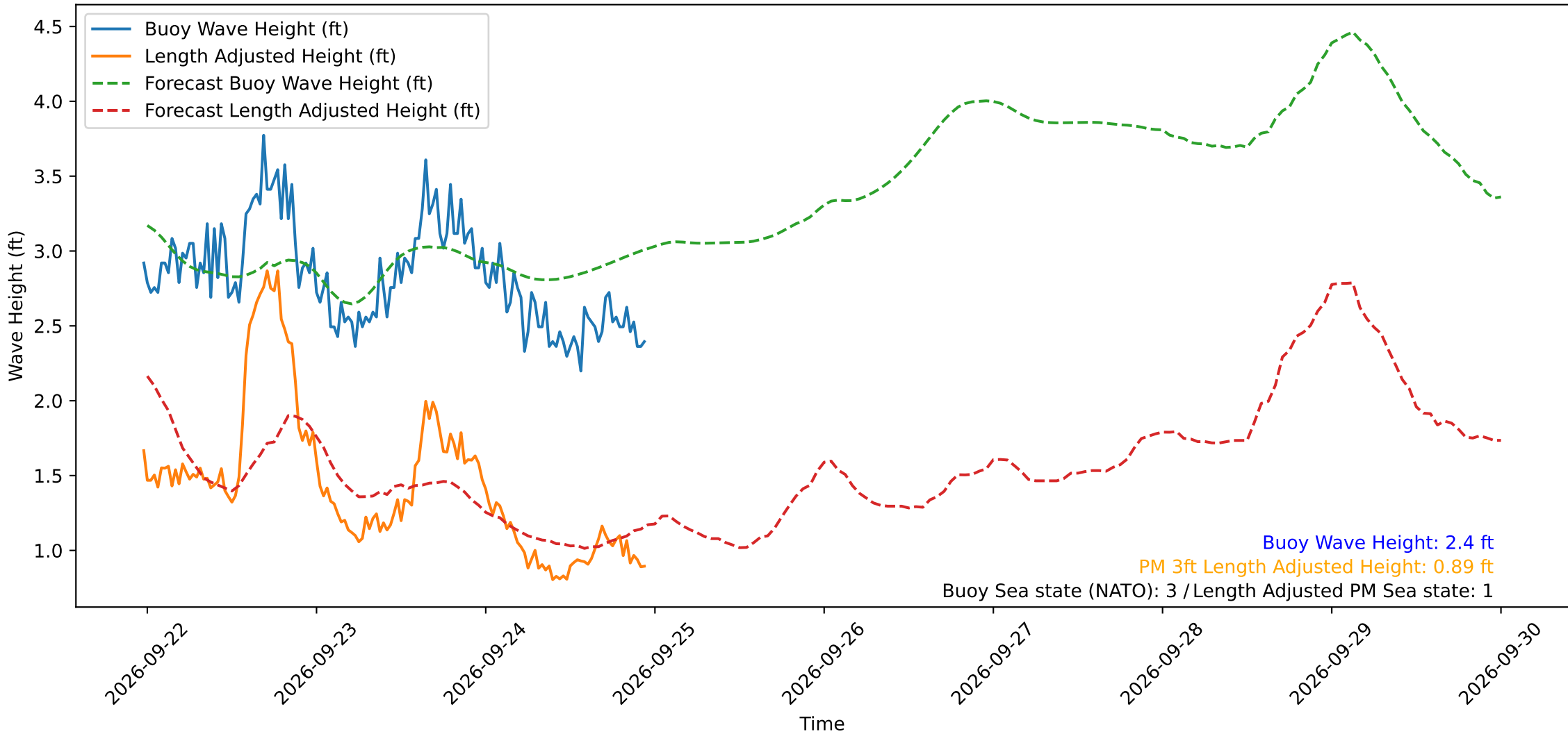
Wave Heights over Time for Oceanside Harbor at 2026-09-24 23:30:31
