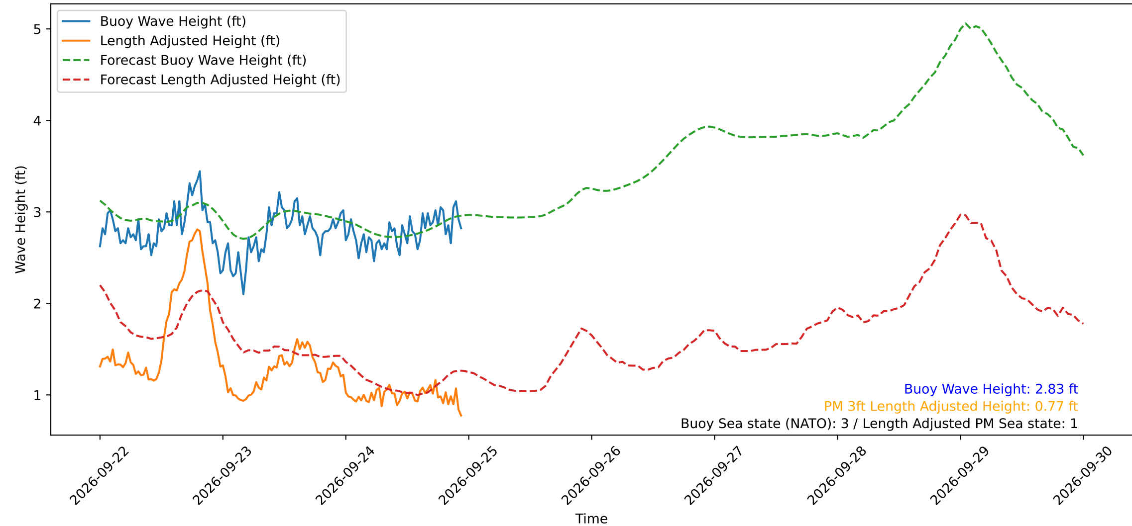
Wave Heights over Time for Green Beach at 2026-09-24 23:31:13
