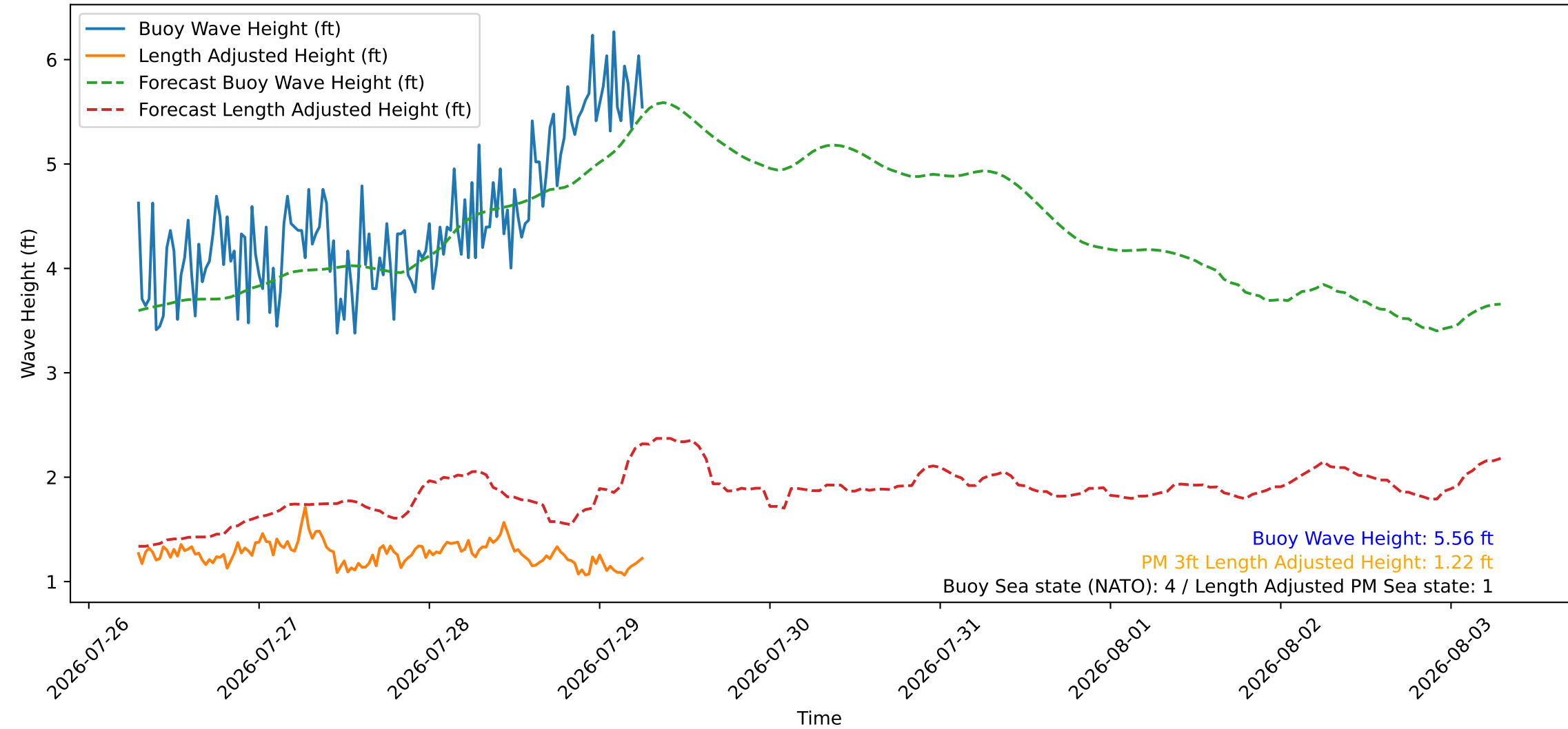
Wave Heights over Time for Green Beach at 2026-07-29 07:01:09
