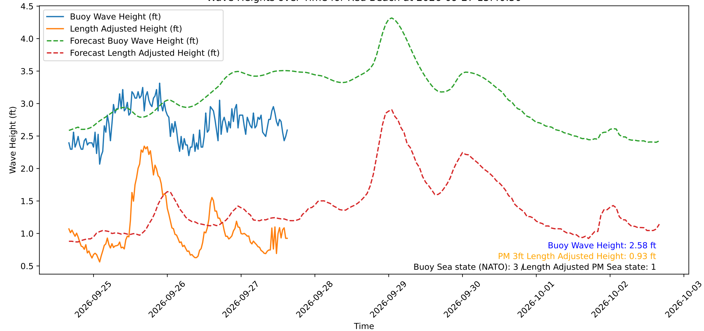
Wave Heights over Time for Red Beach at 2026-09-27 15:40:50
