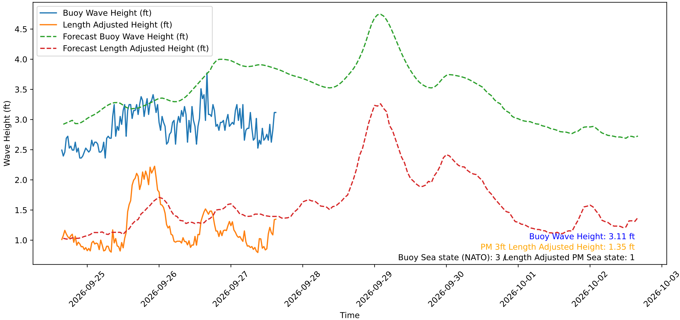
Wave Heights over Time for Oceanside Harbor at 2026-09-27 15:40:30
