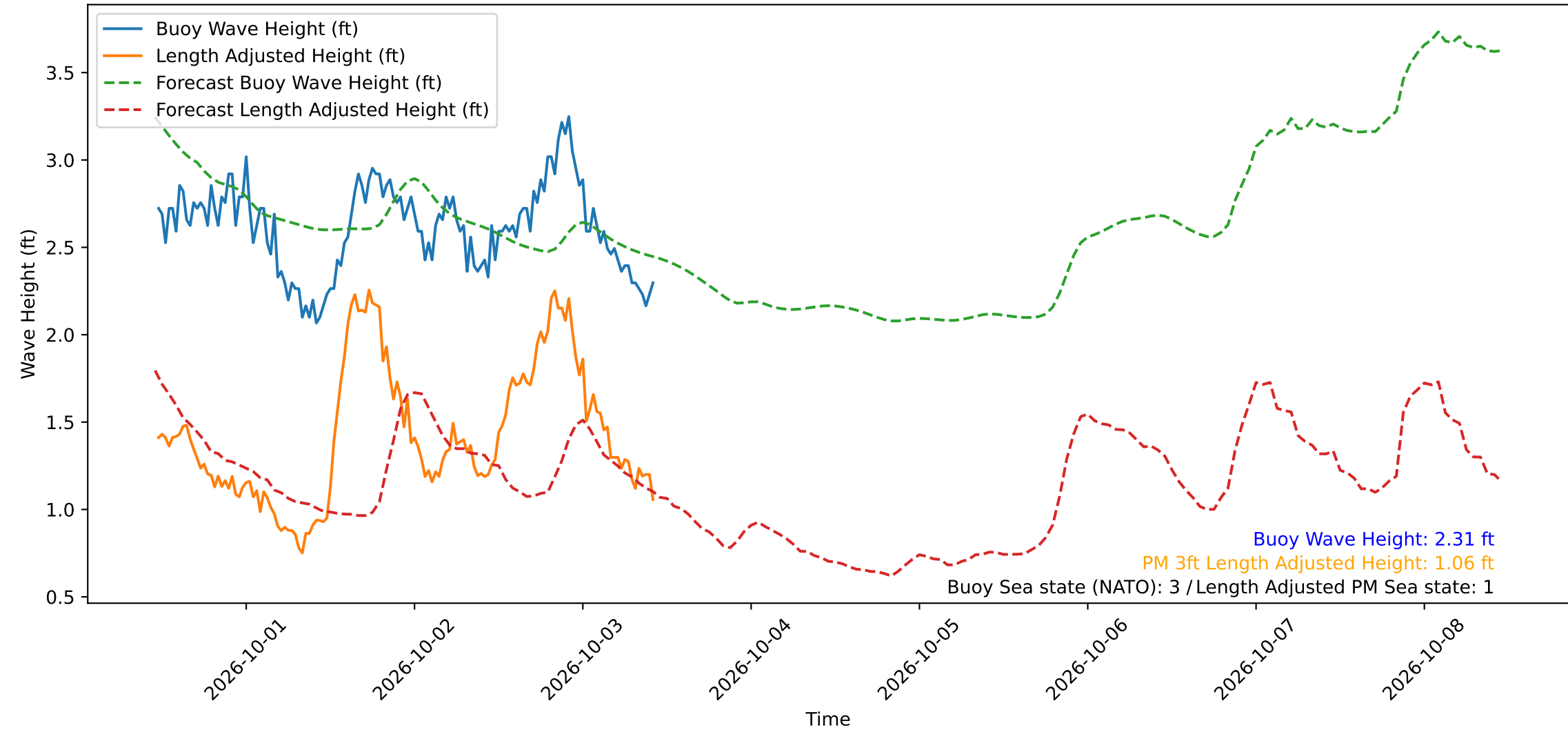
Wave Heights over Time for Red Beach at 2026-10-03 11:00:49
