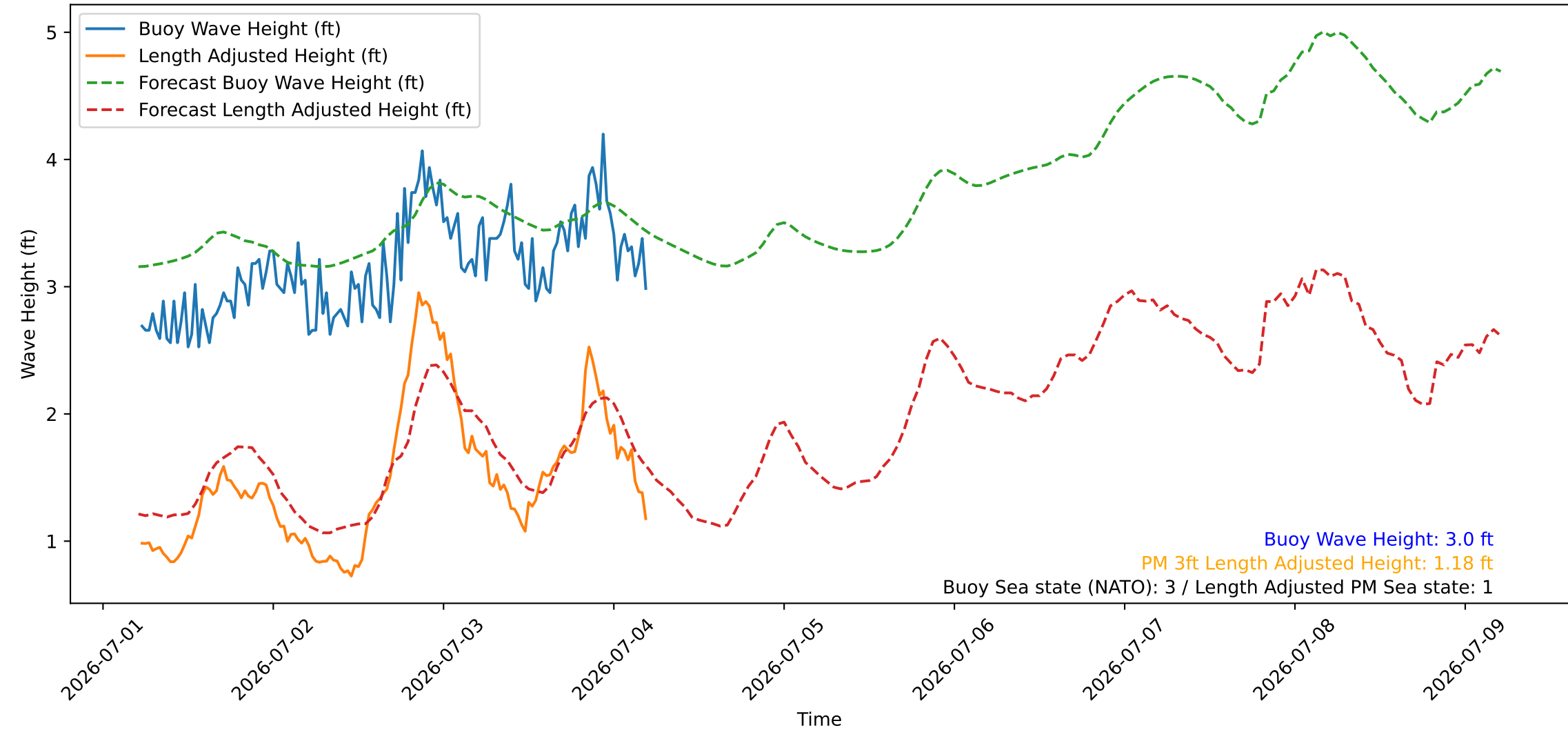
Wave Heights over Time for Green Beach at 2026-07-04 05:21:09
