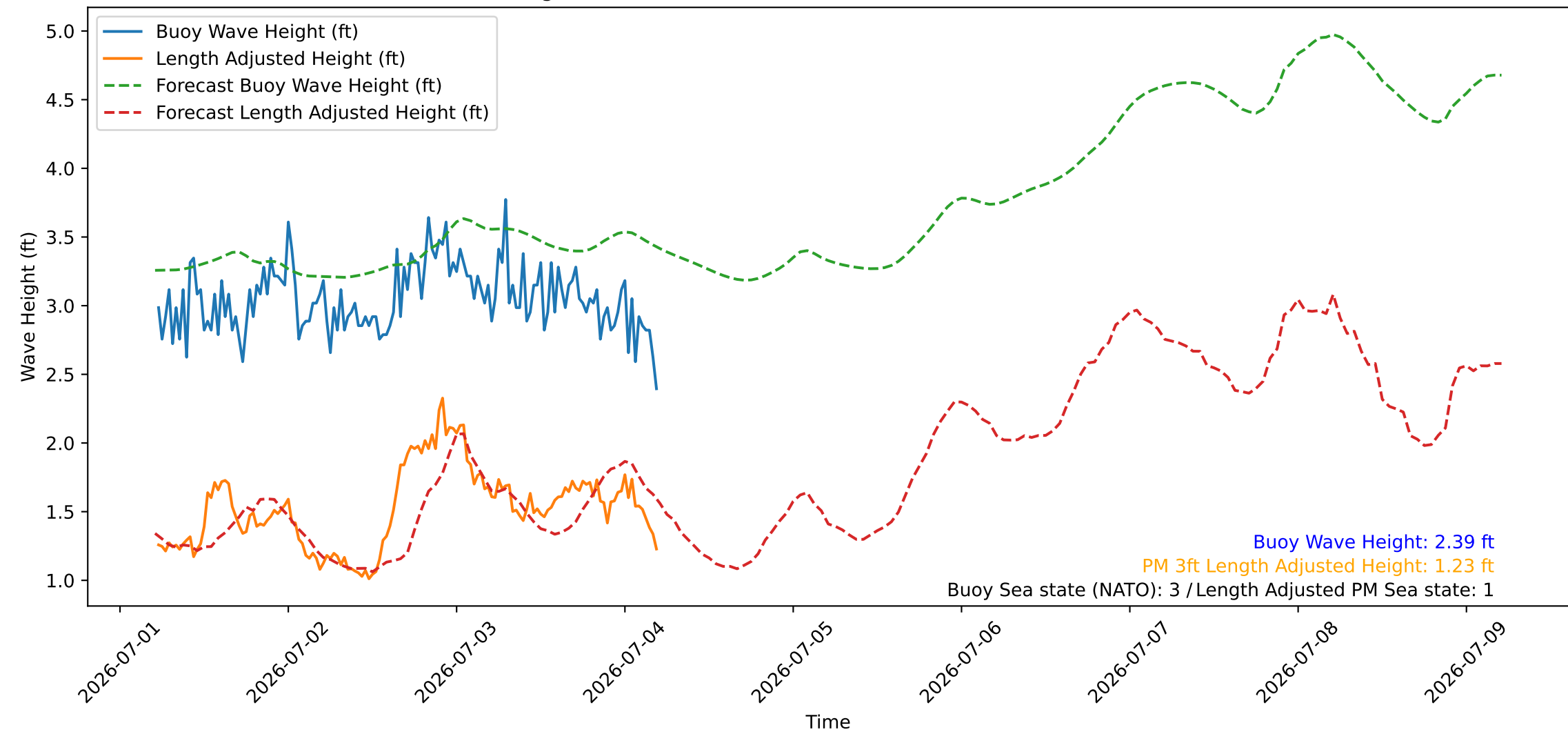
Wave Heights over Time for Oceanside Harbor at 2026-07-04 05:20:26
