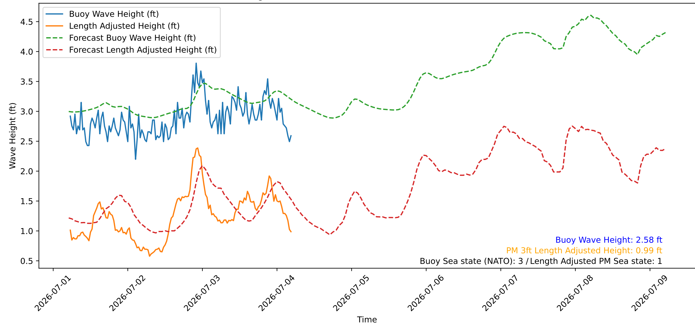
Wave Heights over Time for Red Beach at 2026-07-04 05:20:47
