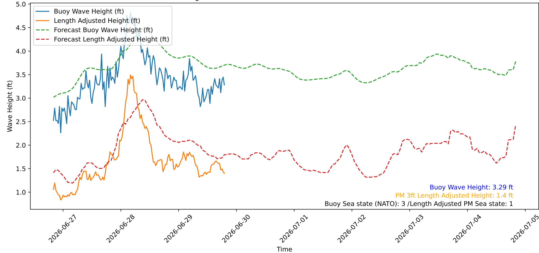
Wave Heights over Time for Green Beach at 2026-06-29 19:51:09
