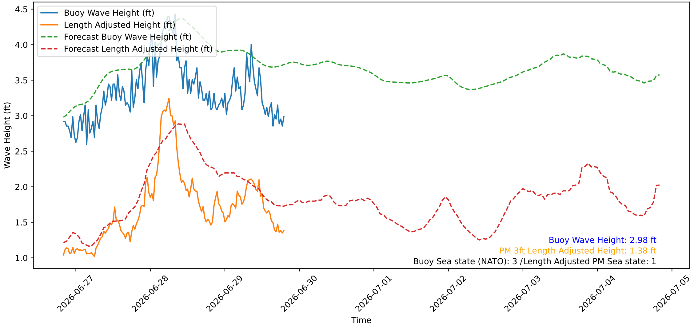
Wave Heights over Time for Oceanside Harbor at 2026-06-29 19:50:25
