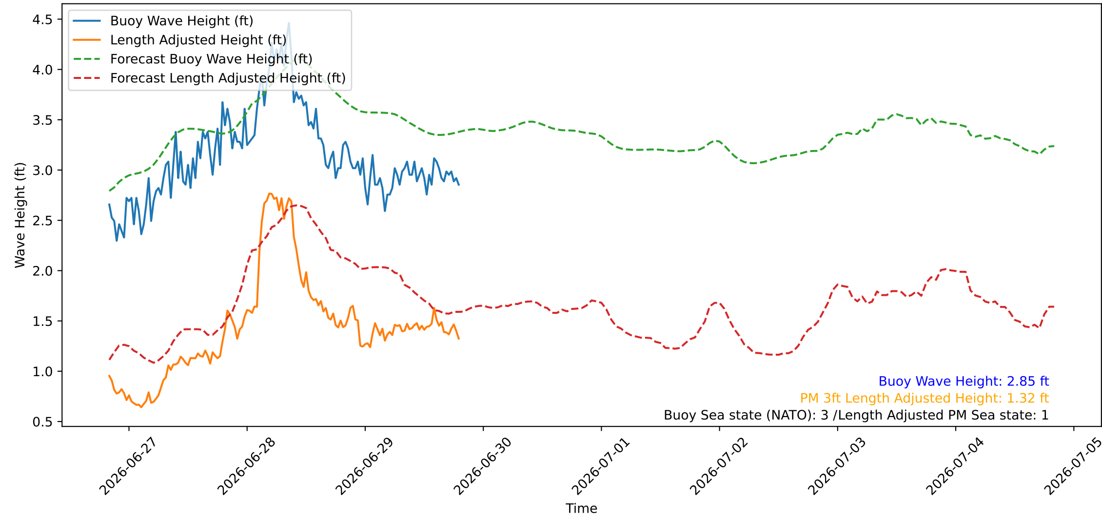
Wave Heights over Time for Red Beach at 2026-06-29 19:50:46
