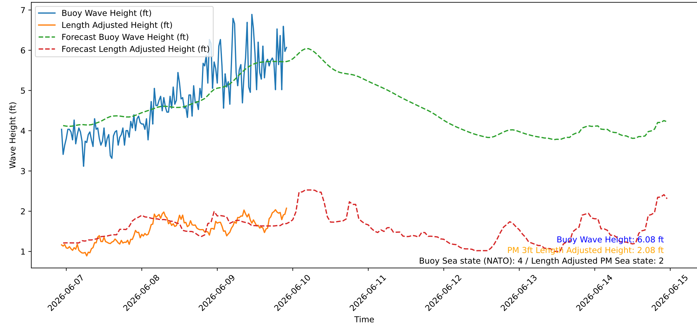
Wave Heights over Time for Green Beach at 2026-06-09 22:41:10
