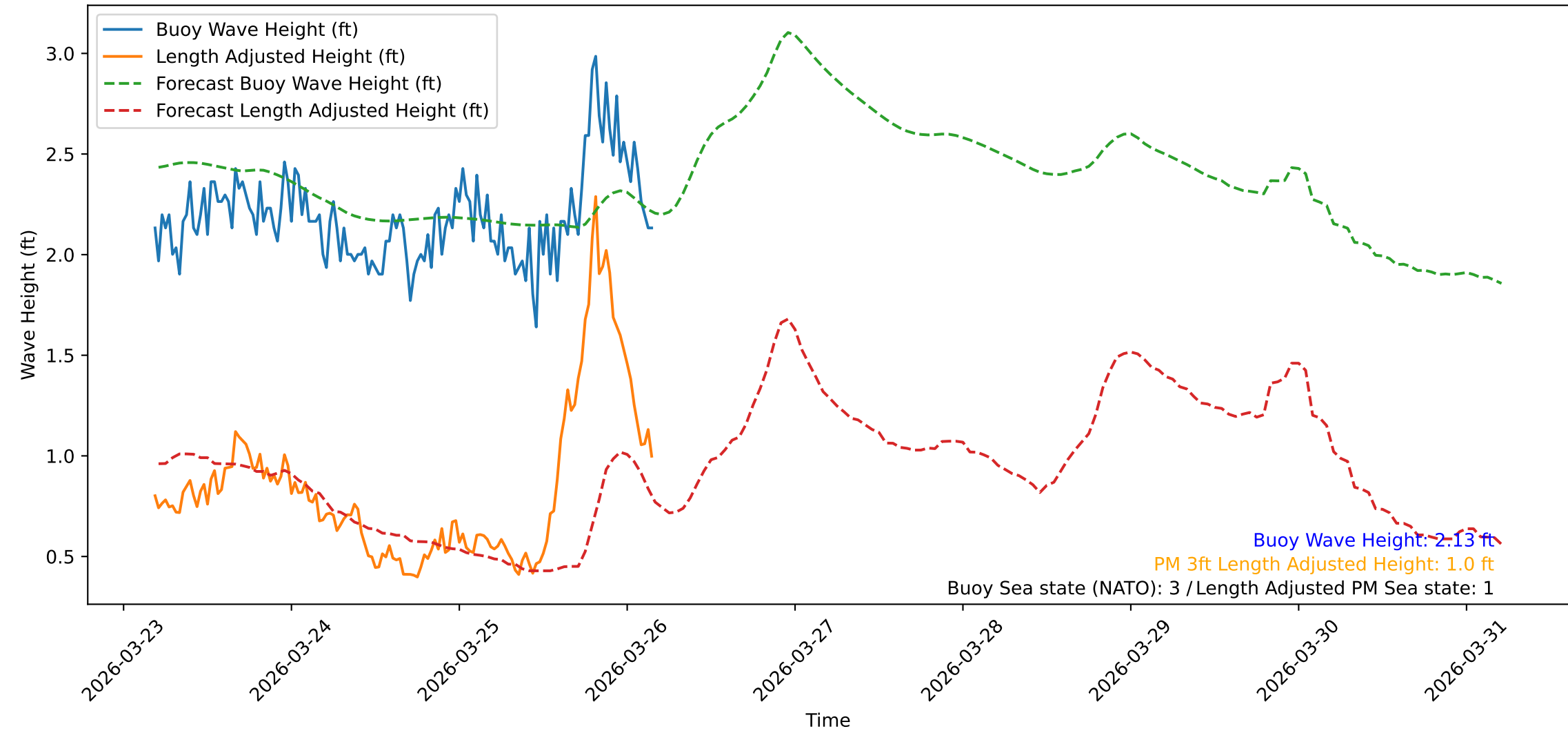
Wave Heights over Time for Green Beach at 2026-03-26 04:31:10
