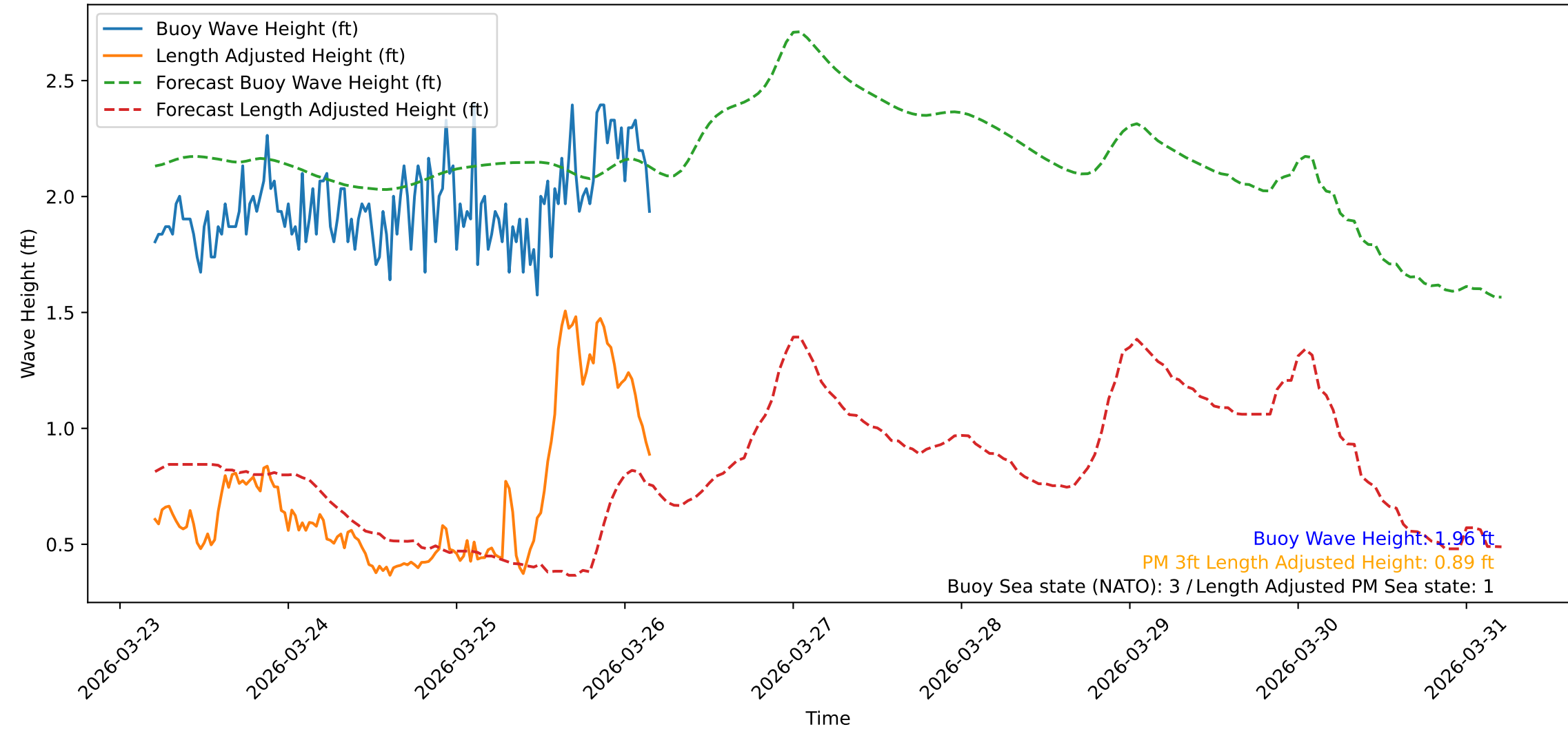
Wave Heights over Time for Red Beach at 2026-03-26 04:30:47
