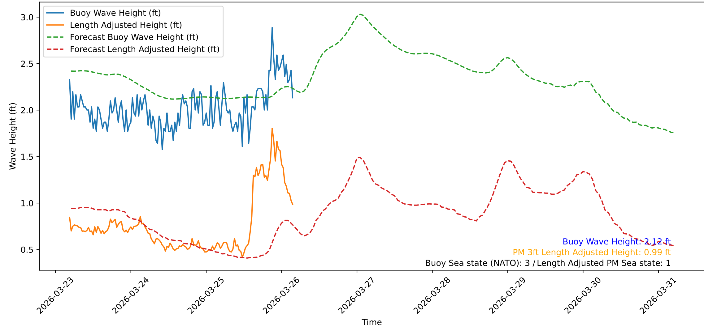
Wave Heights over Time for Oceanside Harbor at 2026-03-26 04:30:32
