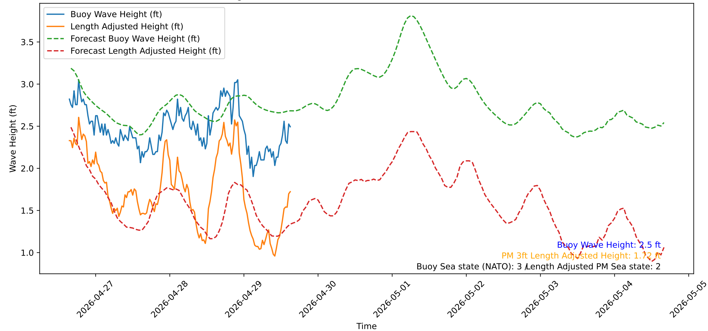
Wave Heights over Time for Oceanside Harbor at 2026-04-29 15:40:32
