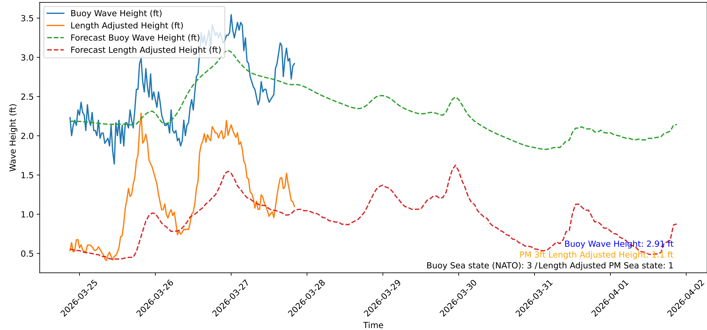
Wave Heights over Time for Green Beach at 2026-03-27 20:51:08
