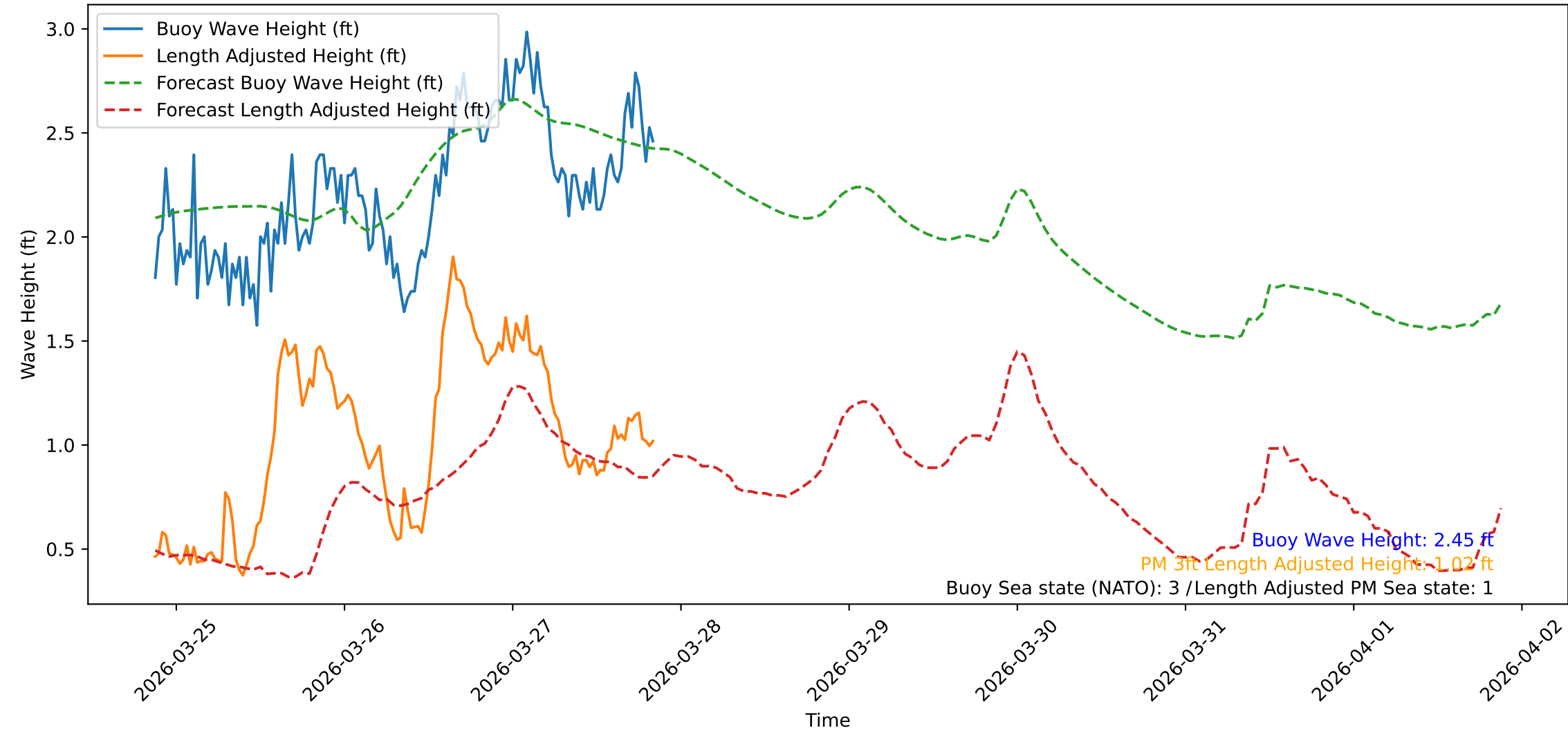
Wave Heights over Time for Red Beach at 2026-03-27 20:50:46
