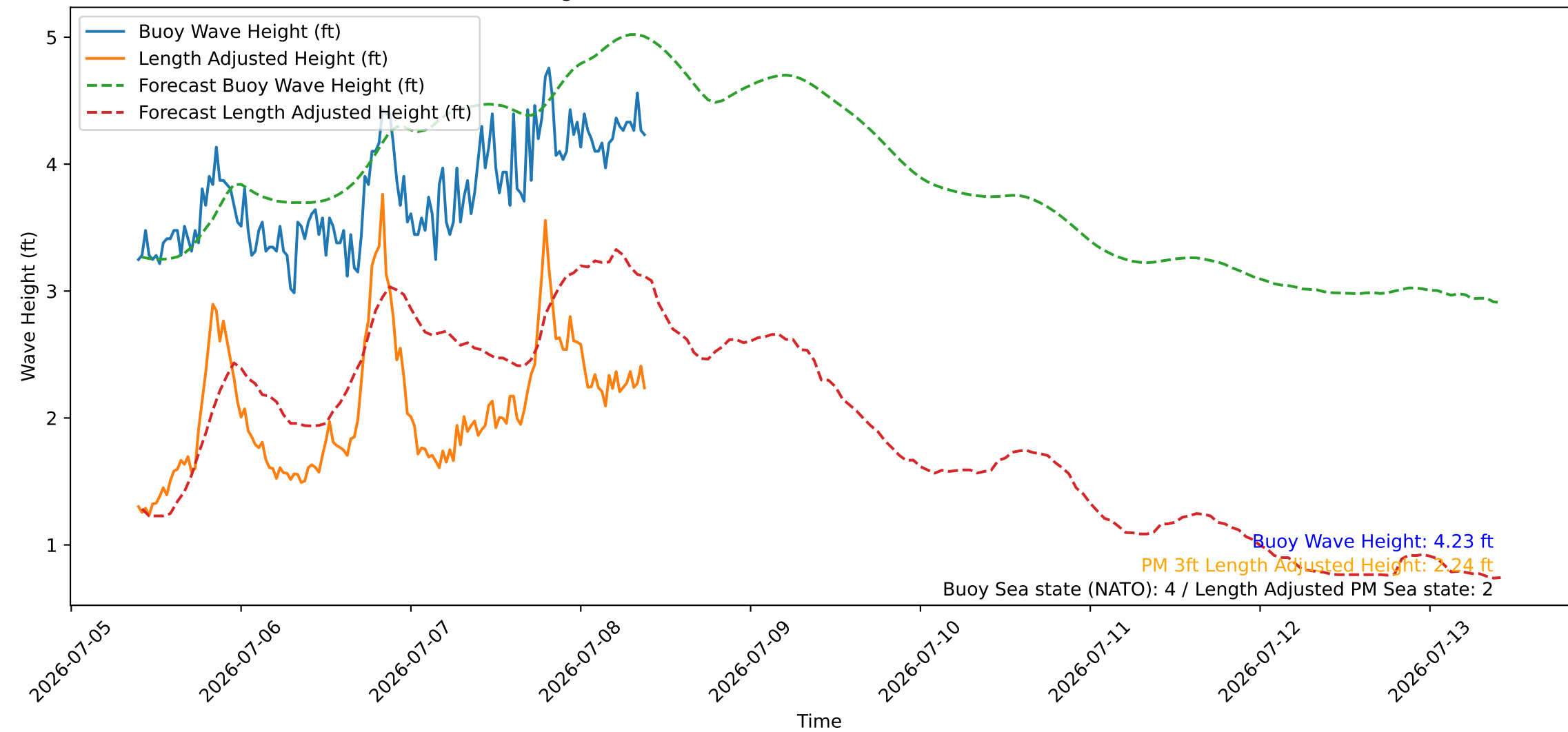
Wave Heights over Time for Green Beach at 2026-07-08 09:41:08
