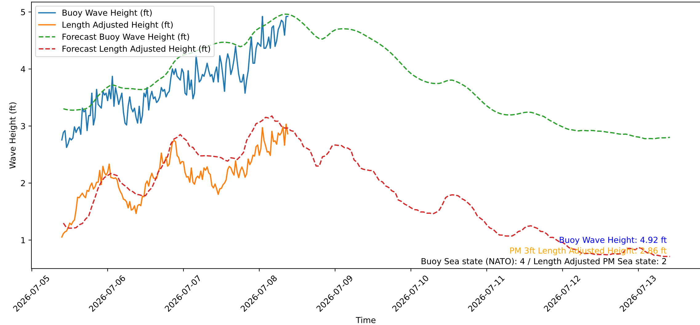
Wave Heights over Time for Oceanside Harbor at 2026-07-08 09:40:26
